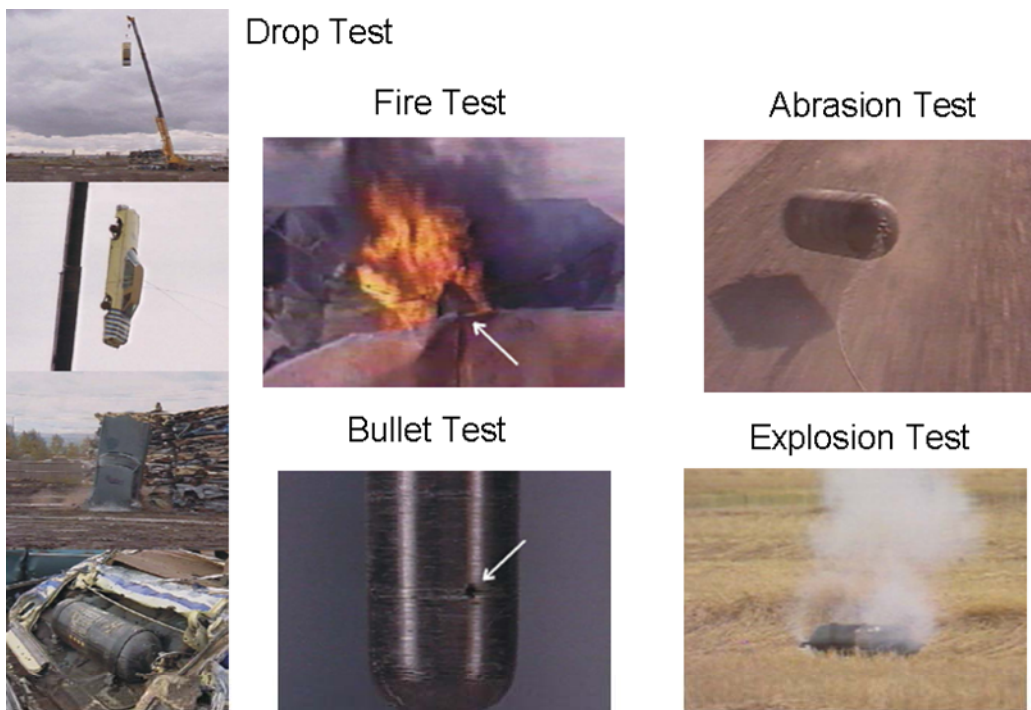
Figure 14. High-Pressure Storage Vessel Qualification Tests
