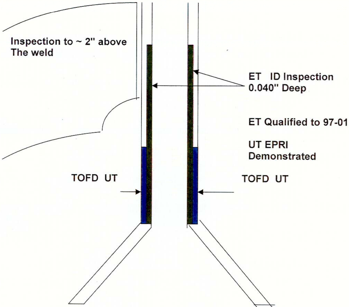
Figure 6: Open Housing Probe Wetted Surfaces ET & UT TOFD CH 2 (Axial Shooting) Area of Coverage
