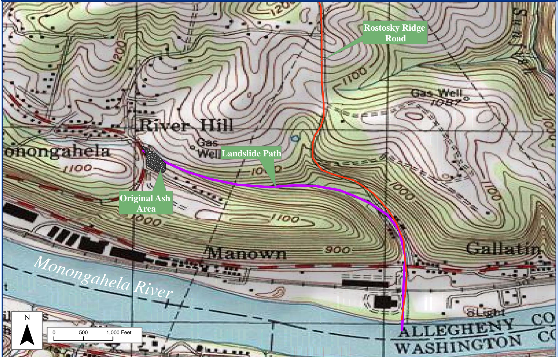
Figure 1: Coal Fly Ash Landslide Forward Township, Allegheny County, Pennsylvania
