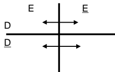
Nondifferential Exposure Misclassification
