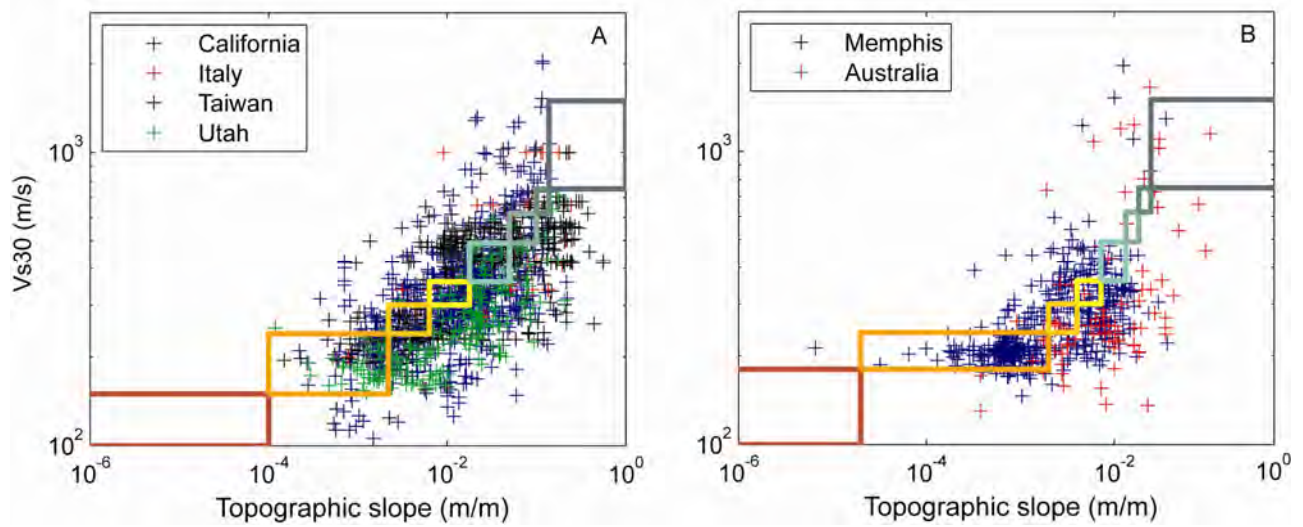
Figure 2. Correlations of measured V_{S^{30}} (m/s) versus topographic slope (m/m) for A , active tectonic, and B , stable continental regions. Color-coded polygons represent V_{S^{30}} and slope ranges consistent with ranges given in table 2 and also consistent with the V_{S^{30}} legends for all geologic- and topographic-based maps throughout this paper.
