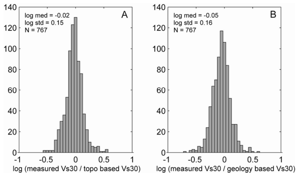
Figure 3. Histograms indicating logarithmic differences of measured Californian V_{S^{30}} values compared with A , values derived from topographic slope correlations and, B , values based on existing V_{S^{30}} site-condition maps. N is the number of V_{S^{30}} measurements.
