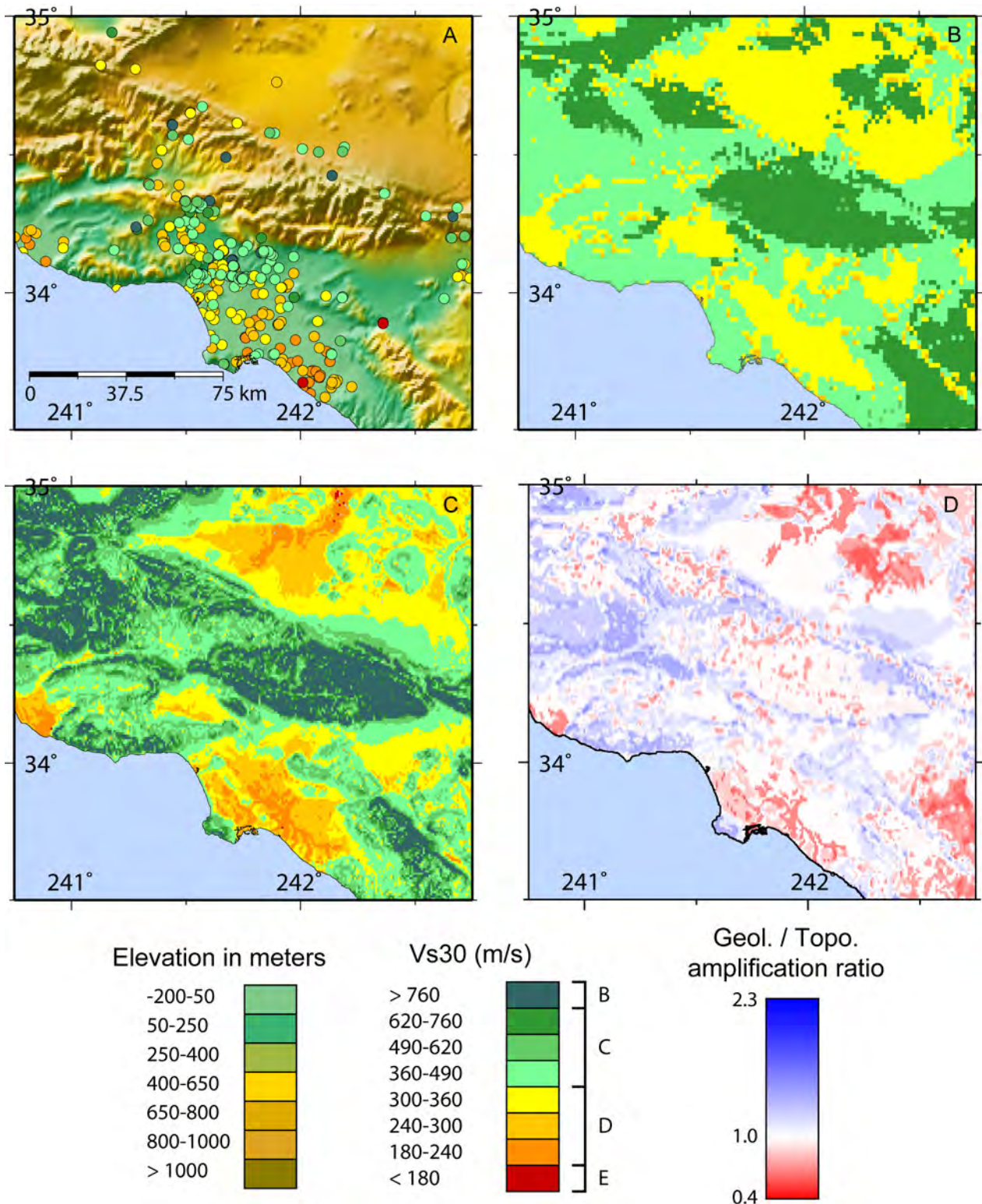
Figure 5. A, Topographic map of the Los Angeles region. Circles indicate the location of measurements, color-coded by V_{s30} in m/s. B, site-condition map based on geology and V_{s30} observations (modified from Wills and others, 2000). C, Site-condition map derived from topographic slope. D, The ratio of the predicted amplification for a uniform PGA of 250 cm/s 2 for the geologically- and topographically-based V_{s30} maps.
