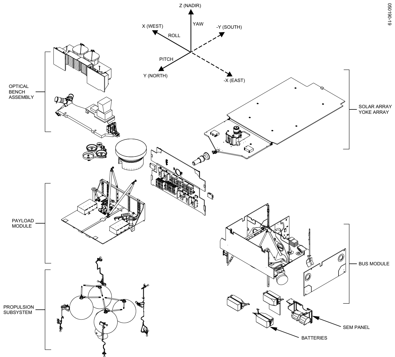
Figure 2-3. GOES N-P Spacecraft Expanded Overview
