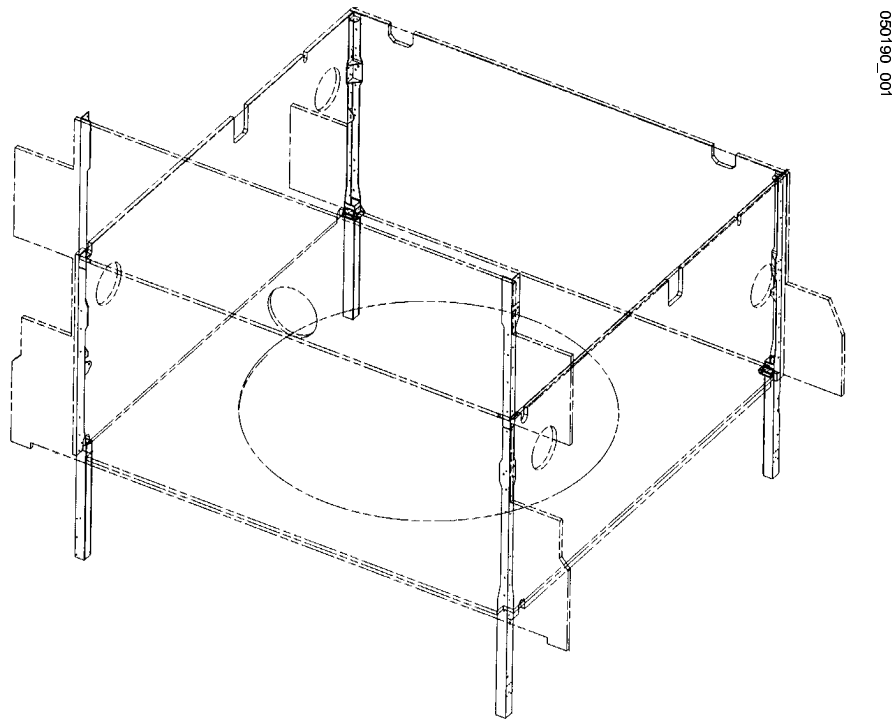
Figure 14-8. Spacecraft Primary Structure
