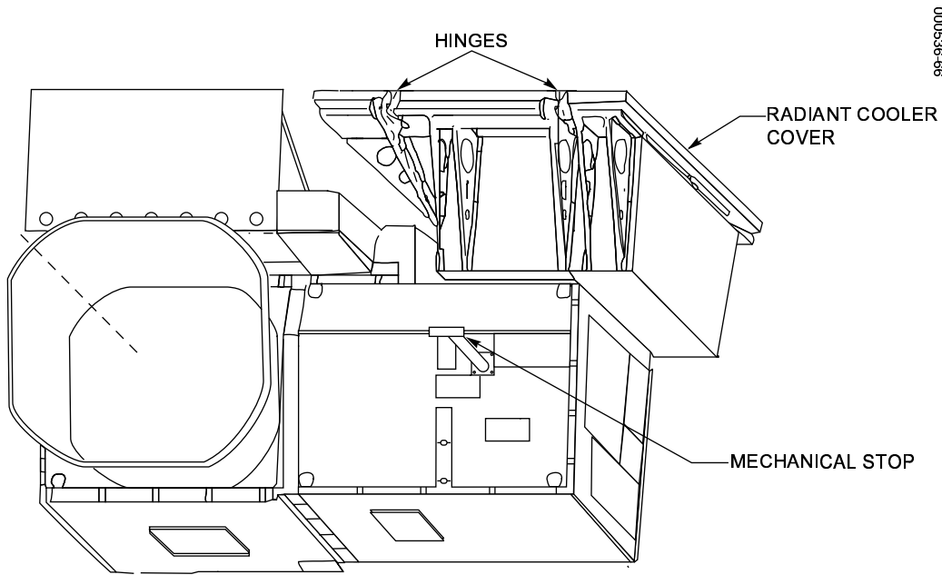
Figure 14-5. Instrument in Closed Position
