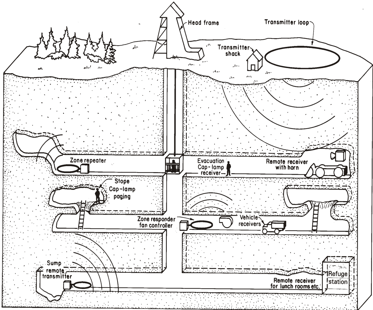
Figure 4.—Conceptual representation of a wireless mine communication and warning system.
