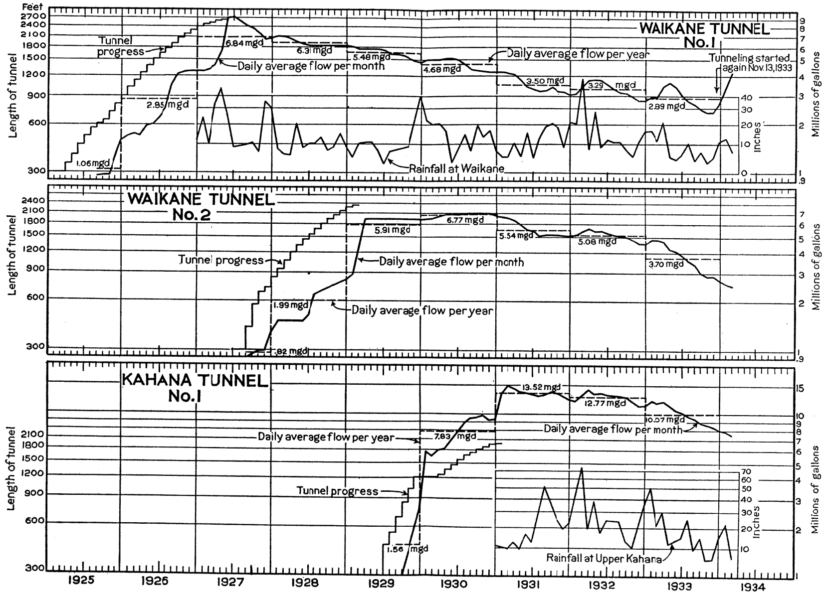
DISCHARGE OF KAHANA AND WAIKANE TUNNELS IN RELATION TO RAINFALL AND TUNNEL PROGRESS
