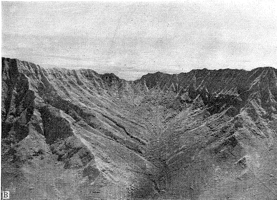
B, AIRPLANE VIEW OF A TRIBUTARY OF LUALUALEI VALLEY, WAIANAE RANGE.
