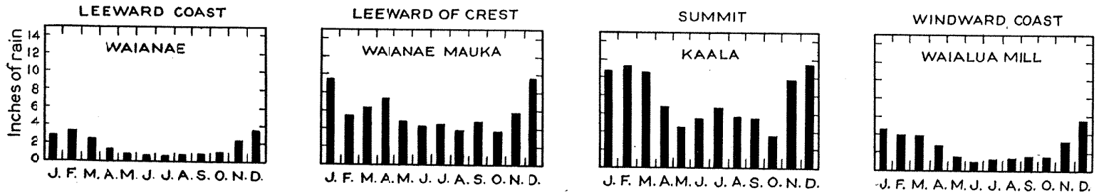
FIGURE 14.—Comparative monthly distribution of rainfall on Oahu.
