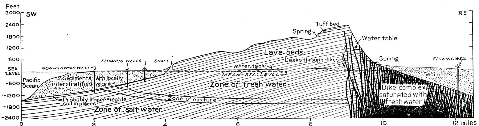
FIGURE 5A.—Diagrammatic section of the Koolau Range at Honolulu showing basal and perched water tables and relation of the fresh water in the dike complex and in the flow lavas to the zone of salt water.
