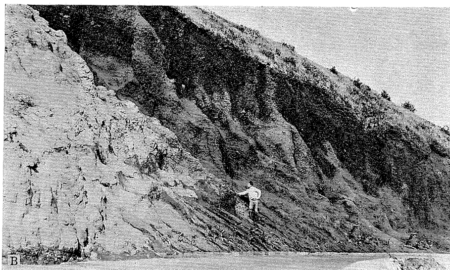
B, UNCONFORMITY ON THE PALI ROAD. Dark-colored cinders from the Pali eruption (on the right) resting unconformably on the eroded light-colored Koolau basalt (on the left). Photograph by Harold T. Stearns.
