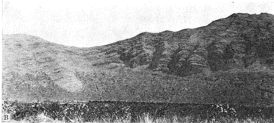
B, VIEW LOOKING NORTH TO SEAWARD END OF MAKAHA RIDGE, WAIANAË RANGE.
