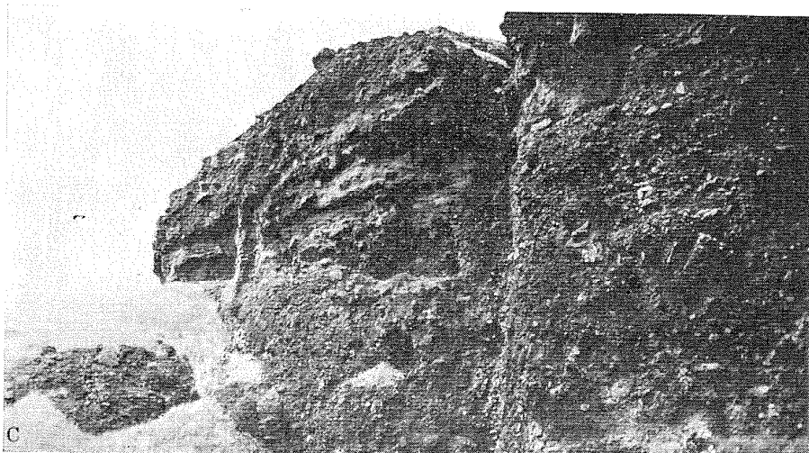
C, BRECCIA IN PUU KAILIO SHOWING FINE TUFFACEOUS BEDS.
