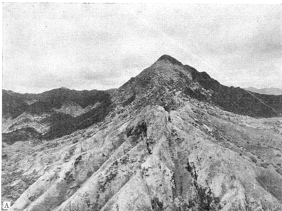
A, AIR VIEW OF THE CLOSELY SPACED DIKES IN PUU PUEO. In the heart of the dike complex of the Koolau volcanic series near Kaneohe Bay. Photograph by 11th Photo Section, Air Corps, Luke Field, T. H.
