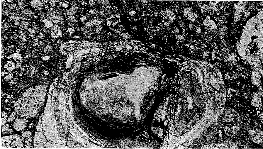
A, SPHEROIDAL WEATHERED BOULDER IN THE OLDER ALLUVIUM NEAR KOLEKOLE PASS, WAIANAE RANGE
