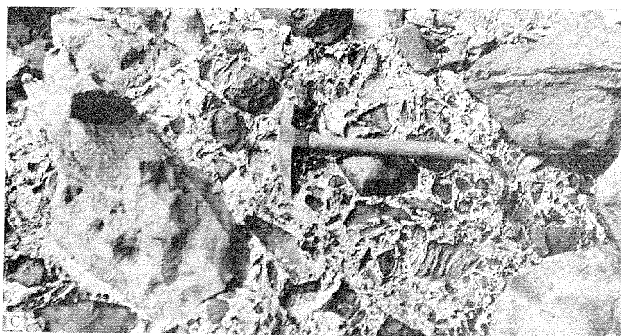
C, BASALT TALUS BRECCIA ON NORTH MOKULUA ISLAND WITH CALCAREOUS CEMENT.
