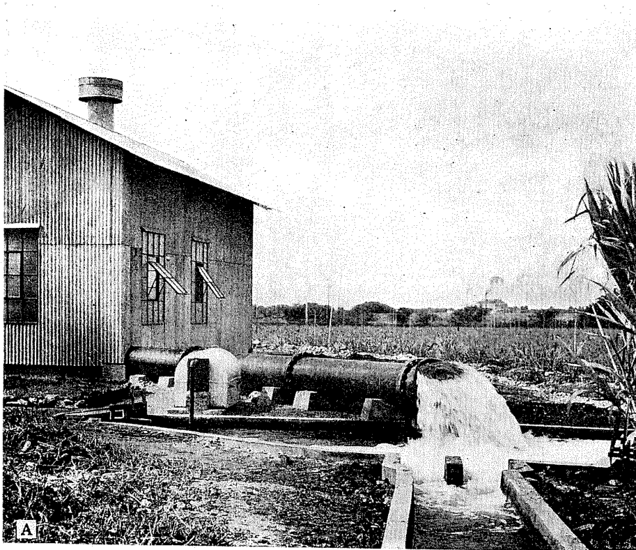
A, WELL 23, DUG IN REEF LIMESTONE AT EWA.
