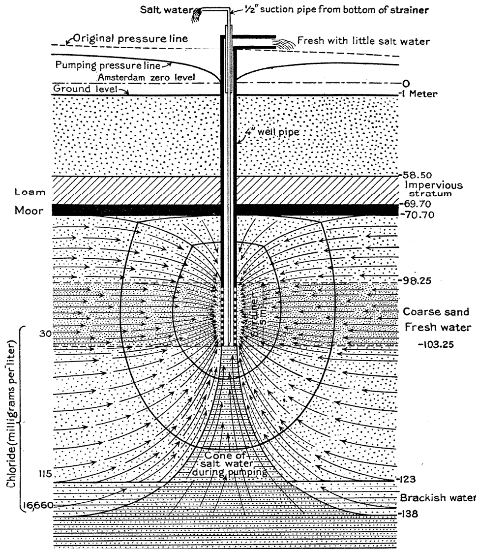
FIGURE 28.—Cone of salt water induced by pumping overlying fresh water. (From Pennink, J.M.K., Am. Soc. Civil Eng. Proc., vol. 54, pt. 4, p. 179, 1905.) Pumping at the rate of 1,200 cubic meters daily. Strainer placed about 35 meters above the level of water having a density equal to sea water. Salinity of sea water approximately 17,000 parts per million of chloride. Zero level of Amsterdam, 0.2 meter above mean sea level.
