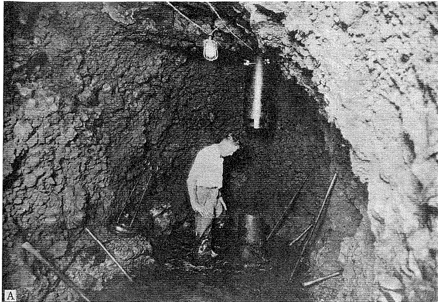
A, TUNNEL ABOUT 20 FEET ABOVE SEA LEVEL IN UPPER WAIANAË AA CLINKER.
