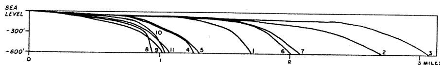
FIGURE 3.—Profiles of the ocean floor seaward from the Lithothamnium ridge near Barbers Point (1 to 5) and near Honolulu (6 and 7) and of the reefless ocean floor southeast of Kaena Point (8 to 11).
