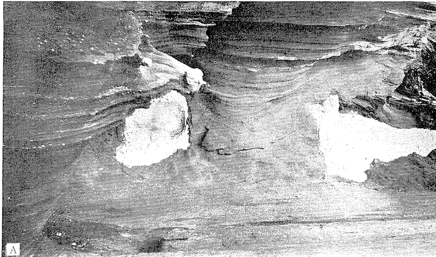
A, TYPICAL LITHIC TUFF ON THE SOUTH SIDE OF KOKO CRATER, MANTLING EMERGED REEF LIMESTONE.
