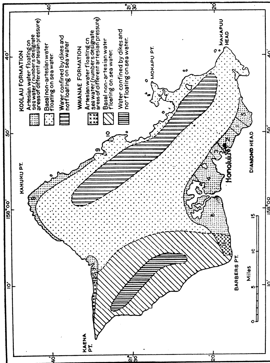
FIGURE 16.—Ground-water areas on Oahu.
