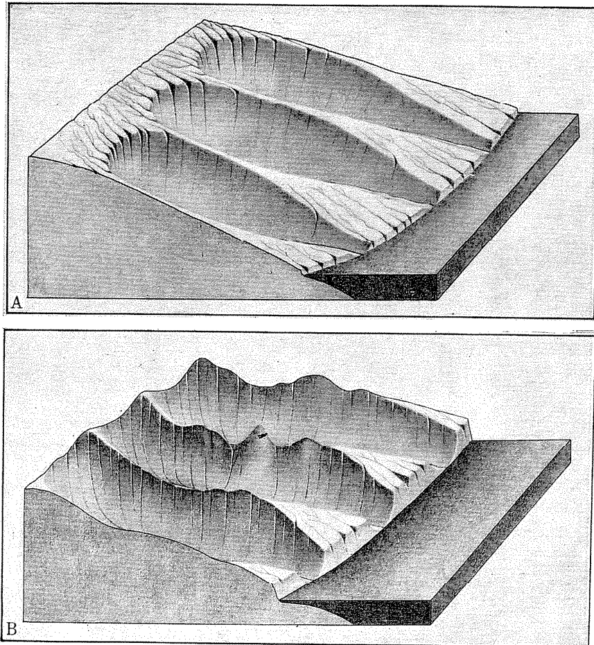
BLOCK DIAGRAMS ILLUSTRATING DEVELOPMENT OF THE PALI BY EROSION
