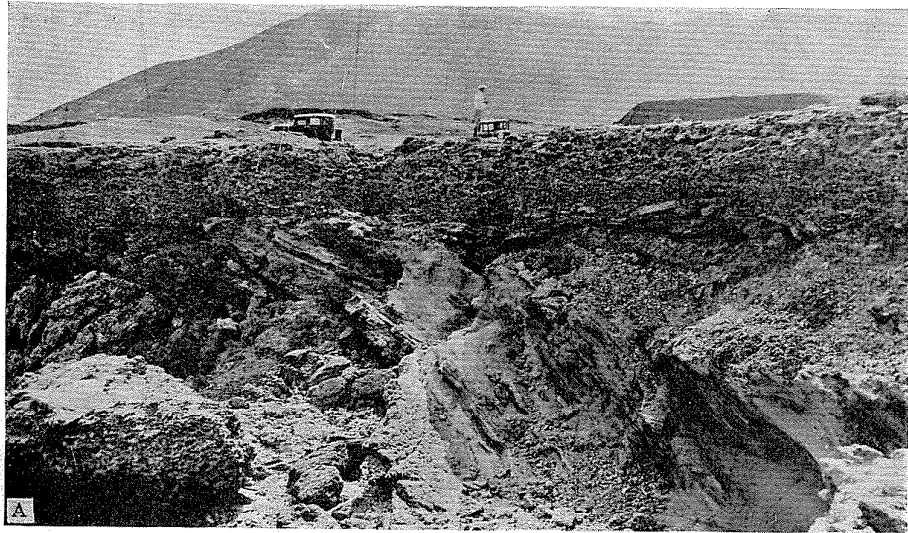
A, UNCONFORMITY ON THE MOKAPU PENINSULA. Calcareous tuff conglomerate forming horizontal bed resting unconformably upon older steeply-dipping fossiliferous marine sediments in the crater of Ulupau cone. The base of the conglomerate is about 22 feet above mean sea level.
