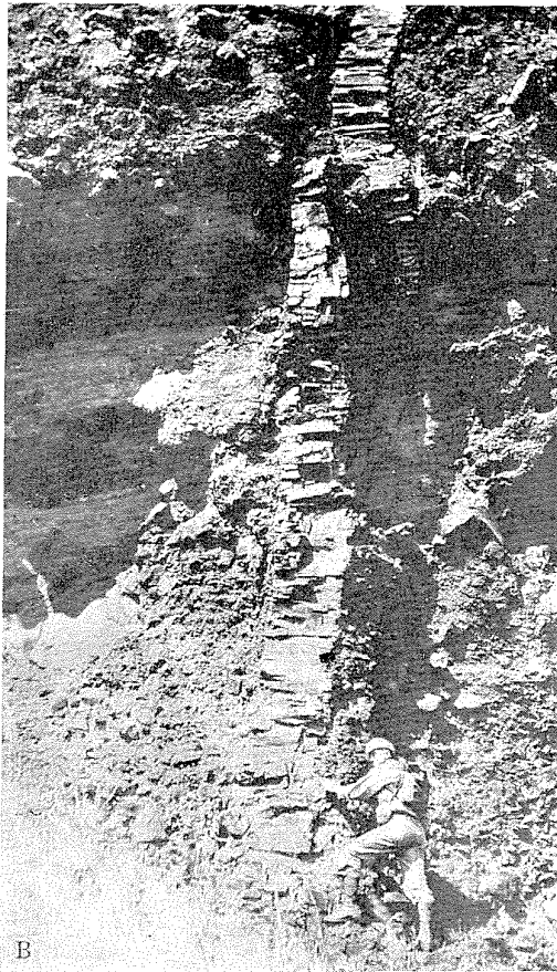
B, DIKE INTRUDED INTO BRECCIA AT PUU KAILIO, LUALUALEI VALLEY, WAIANAË RANGE.
