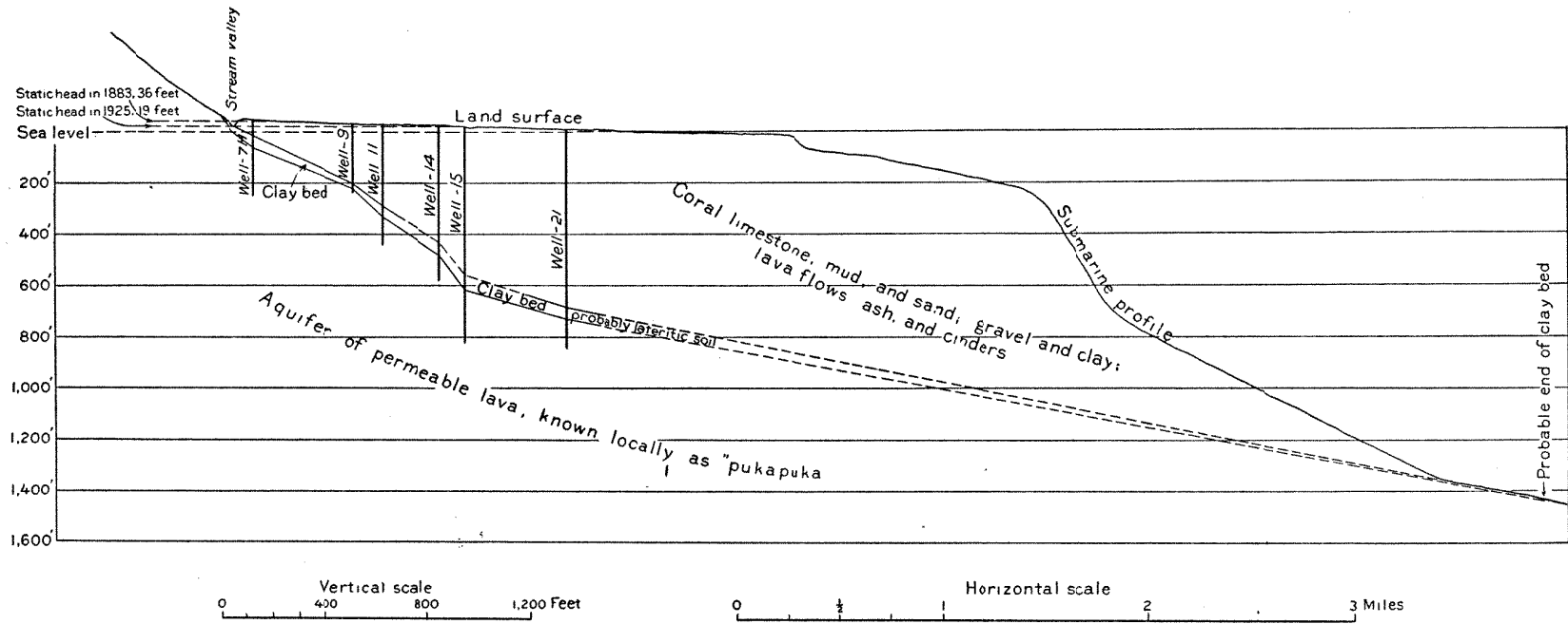
FIGURE 19.—Section of the Waikiki artesian area, Honolulu. The section extends from the junction of Waialae and Kapahula Avenues, in Honolulu, through Aina hau, to a point about 3½ miles offshore. Based on topography by U. S. Geological Survey, soundings by U. S. Coast and Geodetic Survey, and logs of artesian wells. In this area the artesian water originally rose to a height of 36 feet above sea level. (After McCombs).
