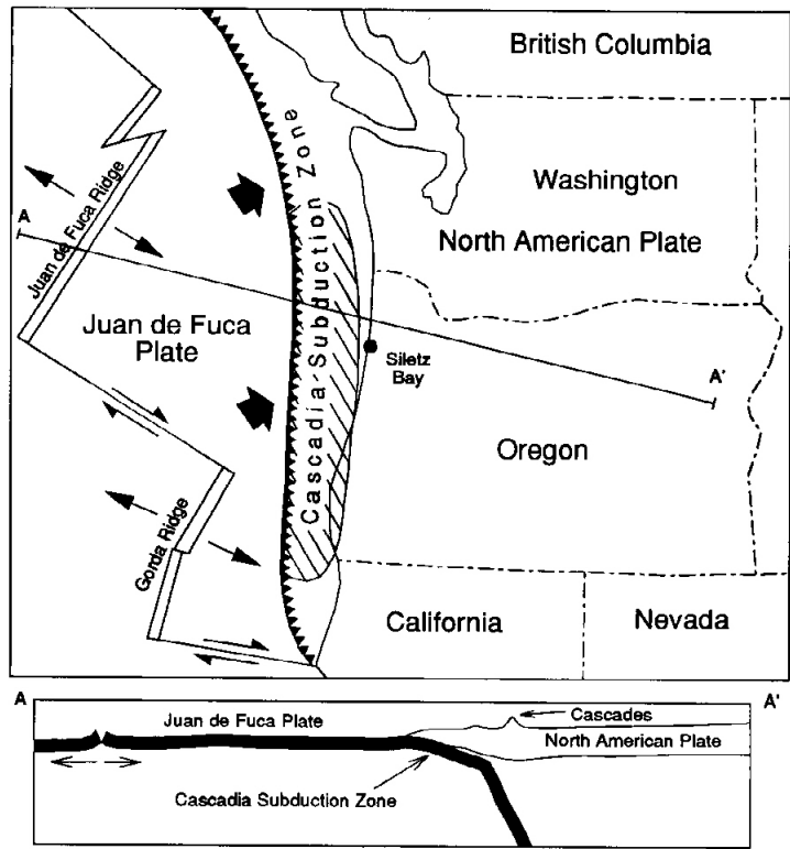
Figure 1. The length of the crosshatched area is the approximate length of the postulated fault rupture for a magnitude 8.8 earthquake on the Cascadia subduction zone.
