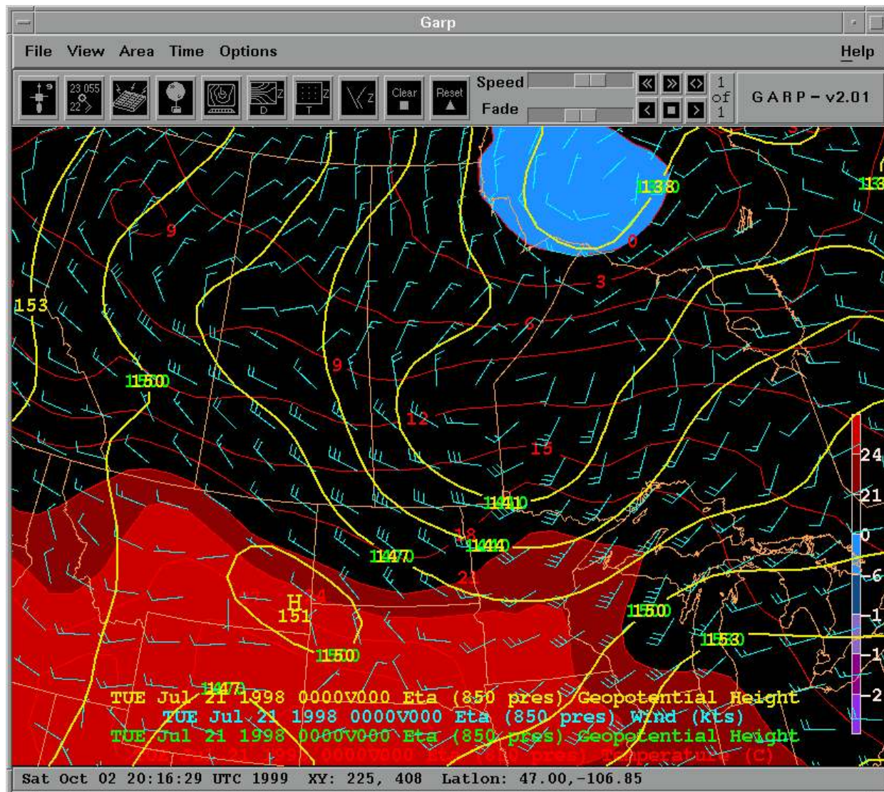
Figure 2: ETA 850 hPa analysis for 0000 UTC 21 July 1998.
