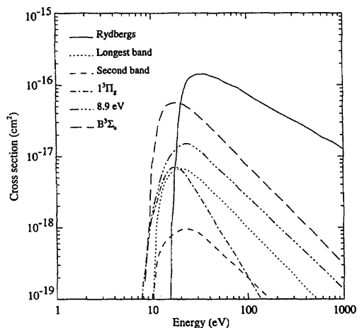
FIG. 11. The remaining excitation cross sections from Table 2.
