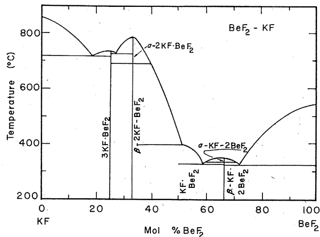
FIGURE 15. Temperature-composition phase diagram for \text{BeF}_2\text{-KF} . M. P. Borzenkova, A. V. Novoselova, Yu. P. Simanov, V. I. Chernikh, and E. I. Yarembash, Zh. Neorg. Khim. , 1 , 2071-82 (1956).
