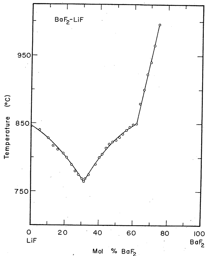
FIGURE 13. Temperature-composition phase diagram for BaF 2 -LiF. A. G. Bergman and E. I. Banachek, Izv. Sekt. Fiz. Khim. A. , 23 , 201 (1953).
