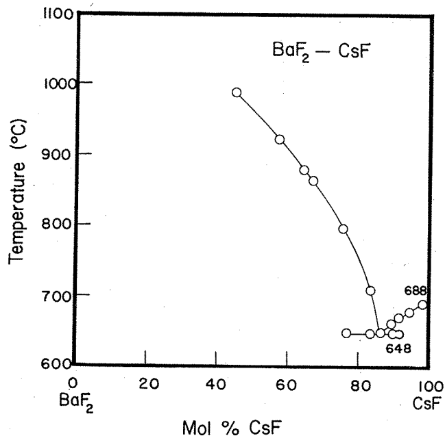
FIGURE 9. Temperature-composition phase diagram for \text{BaF}_2\text{-CsF} . G. A. Bukhalova and E. S. Yagubyan, Izv. Akad. Nauk S.S.S.R., 3, 1096 (1967).
