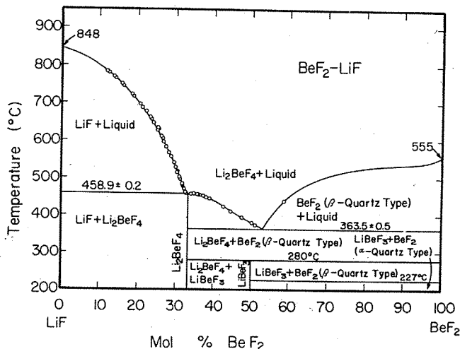
FIGURE 16. Temperature-composition phase diagram for BeF 2 -LiF. K. A. Romberger, J. Braunstein, and R. E. Thoma, J. Phys. Chem., 76 , 1159 (1972).
