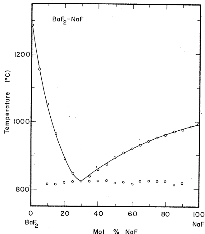
FIGURE 14. Temperature-composition phase diagram for \text{BaF}_2\text{-NaF} . G. Z. Grube, Z. Elektrochem. , 33 , 481 (1927).
