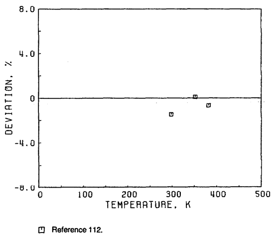
FIG. 42. Deviation plot for the self-diffusion coefficient of ethane, secondary data.
