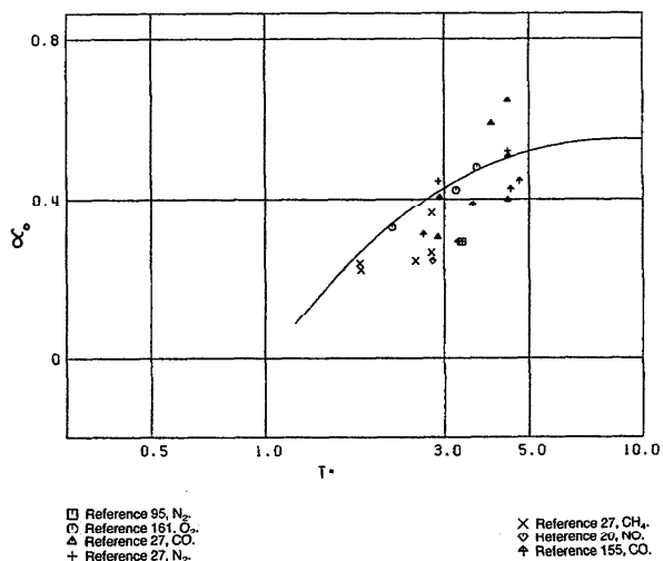
FIG. 43. Isotopic thermal diffusion factor of nitrogen, oxygen, nitric oxide, carbon monoxide, and methane.
