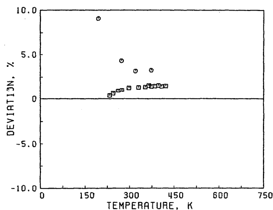
FIG. 18. Deviation plot for the self-diffusion coefficient of carbon monoxide, primary and secondary data.
