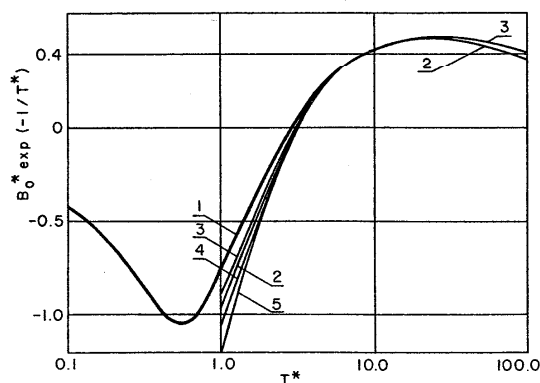
Fig. 1. Correlation of spherical, reduced second virial coefficient, B_0^* , as a function of reduced temperature. (1) Najafi et al. 2 ; (2) N_2 , O_2 , NO , CO ; (3) CH_4 ; (4) CF_4 ; (5) SF_6 .
