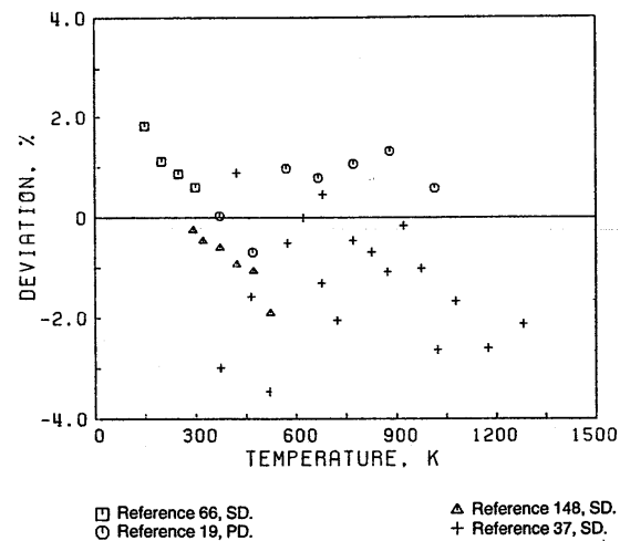
FIG. 15. Deviation plot for the viscosity of nitric oxide, primary and secondary data.
