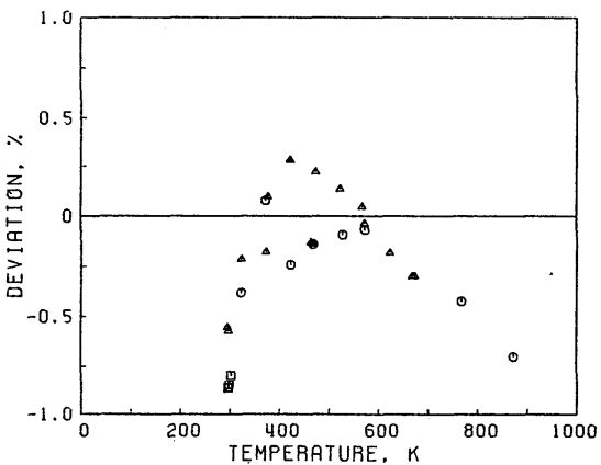
FIG. 31. Deviation plot for the viscosity of carbon tetrafluoride, primary data.
