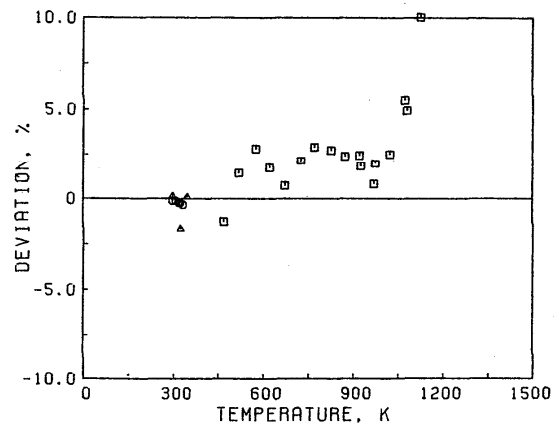
FIG. 33. Deviation plot for the viscosity of sulfur hexafluoride, primary data.
