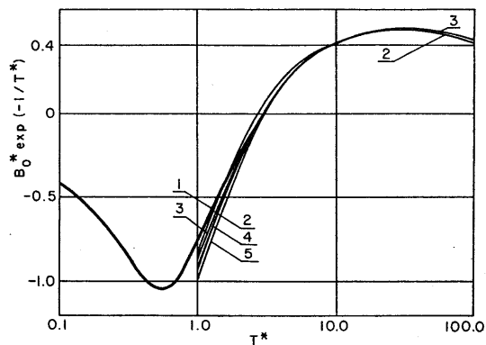
Fig. 2. Correlation of spherical, reduced second virial coefficient, B_0^* , as a function of reduced temperature. (1) Najafi et al. 2 ; (2) CO_2 ; (3) N_2O ; (4) C_2H_4 ; (5) C_2H_6 .
