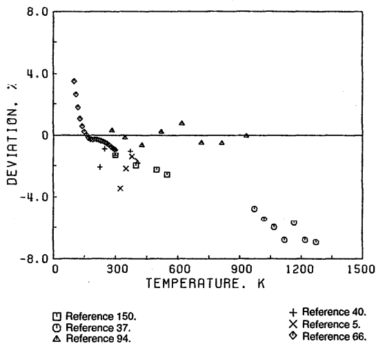
FIG. 7. Deviation plot for the viscosity of nitrogen, secondary data.
