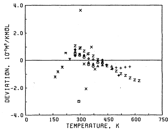
FIG. 24. Deviation plot for the self-diffusion coefficient of carbon dioxide, secondary data.
