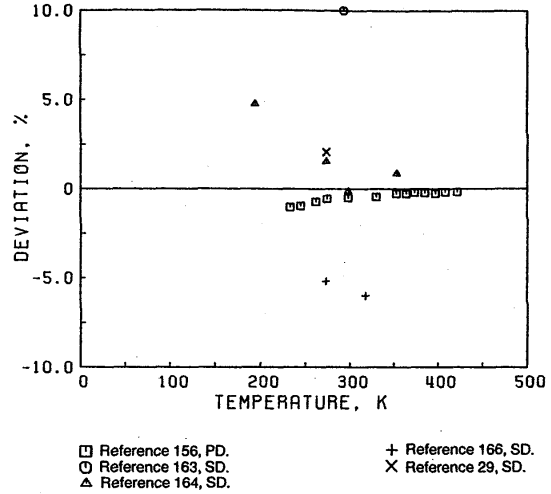
FIG. 8. Deviation plot for the self-diffusion coefficient of nitrogen, primary and secondary data.
