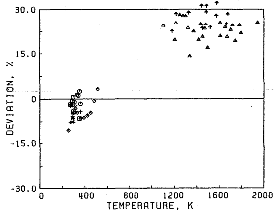
FIG. 23. Deviation plot for the viscosity of carbon dioxide, primary and secondary data.
