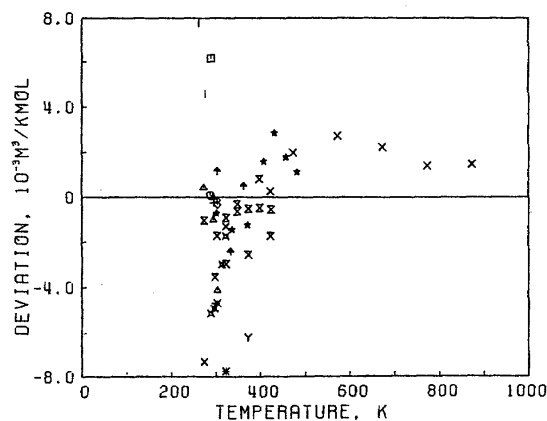
FIG. 21. Deviation plot for the second virial coefficient of carbon dioxide, primary data.
