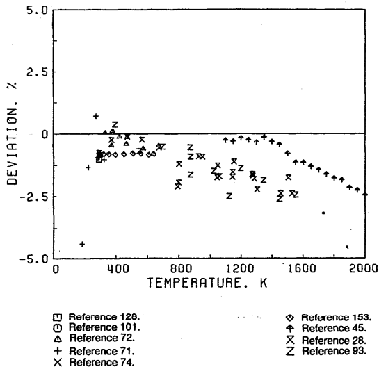
FIG. 6. Deviation plot for the viscosity of nitrogen, primary data.
