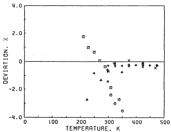
FIG. 26. Deviation plot for the second virial coefficient of methane, secondary data.
