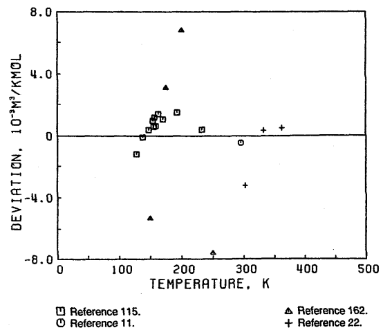
FIG. 10. Deviation plot for the second virial coefficient of oxygen, secondary data.
