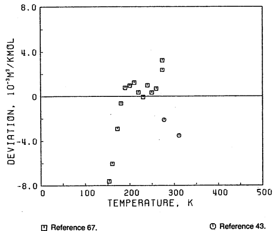
FIG. 14. Deviation plot for the second virial coefficient of nitric oxide, secondary data.
