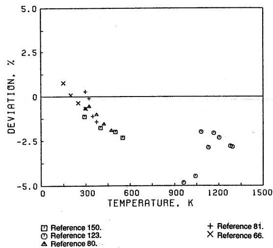
FIG. 12. Deviation plot for the viscosity of oxygen, secondary data.
