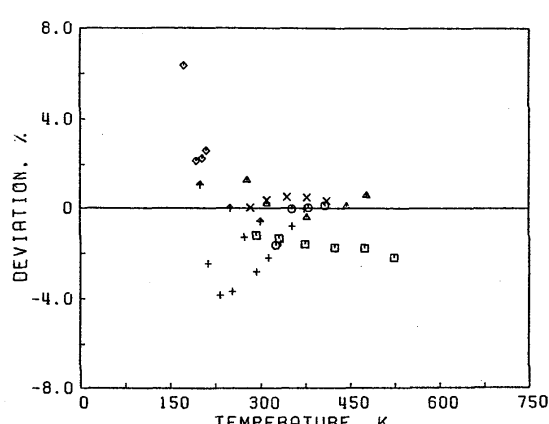
FIG. 27. Deviation plot for the viscosity of methane, primary data.
