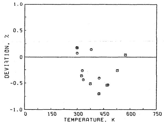
FIG. 33. Deviation plot for the viscosity of sulfur hexafluoride, primary data.
