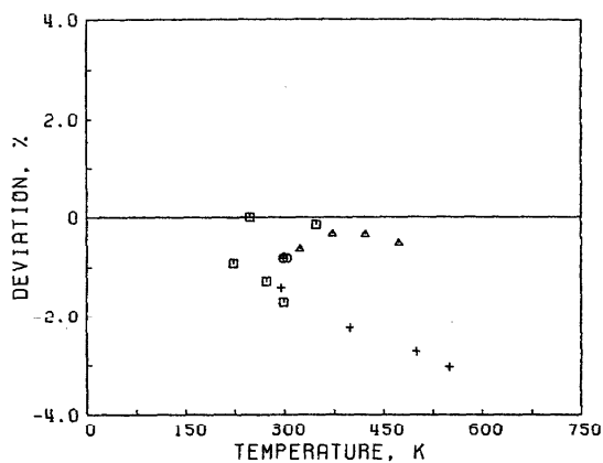
FIG. 17. Deviation plot for the viscosity of carbon monoxide, primary and secondary data.
