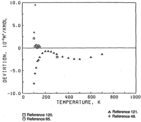
FIG. 5. Deviation plot for the second virial coefficient of nitrogen, secondary data.
