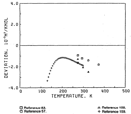
FIG. 9. Deviation plot for the second virial coefficient of oxygen, primary data.
