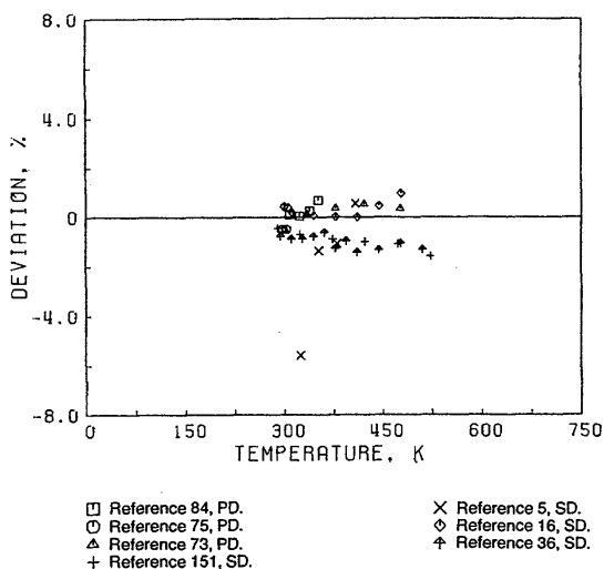
FIG. 41. Deviation plot for the viscosity of ethane, primary and secondary data.
