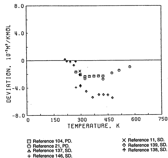
FIG. 16. Deviation plot for the second virial coefficient of carbon monoxide, primary and secondary data.
