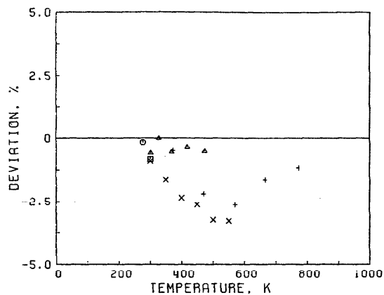
FIG. 20. Deviation plot for the viscosity of nitrous oxide, primary and secondary data.
