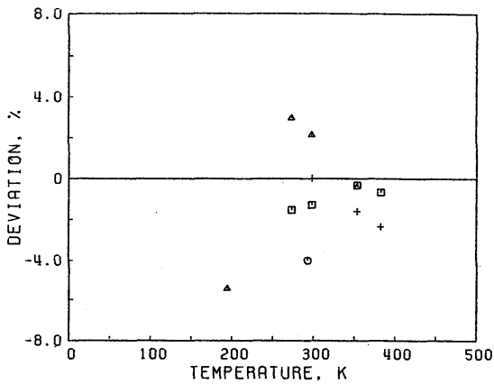
FIG. 29. Deviation plot for the self-diffusion coefficient of methane, primary and secondary data.
