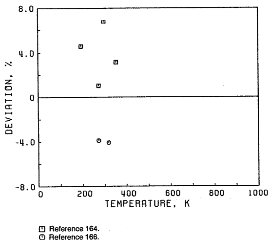
FIG. 13. Deviation plot for the self-diffusion coefficient of oxygen, secondary data.
