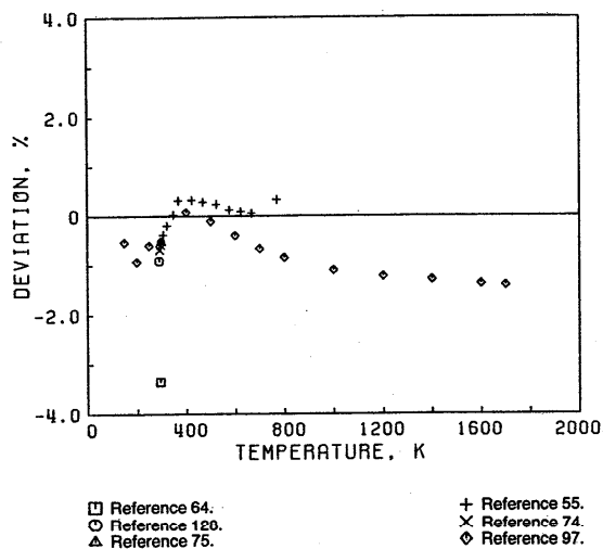
FIG. 11. Deviation plot for the viscosity of oxygen, primary data.
