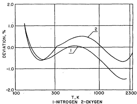
FIG. 3. Deviation of Imperial College (IC) correlation due to Cole and Wakeham (Ref. 30) from Brown (B) correlation.
