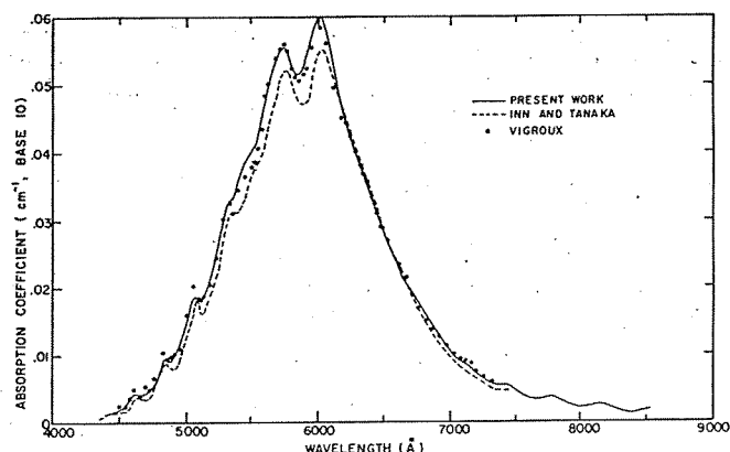
FIGURE 1. Absorption coefficient of ozone, 440–850 nm (Chappuis bands). Absorption coefficient in units of \text{cm}^{-1} (atm at 273 K) -1 base 10, i.e. k = (1/p \cdot l) \log_{10}(I_0/I) . (Figure 4 from M. Griggs, J. Chem. Phys. 49 , 857 (1968) with consent of the author.)
