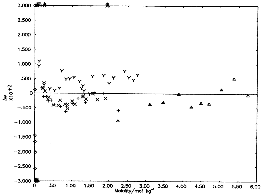
Deviation Plot for \text{CuCl}_2 : \Delta\theta vs molality
