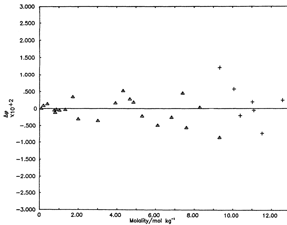
Deviation Plot for \text{Pb}(\text{ClO}_4)_2 : \Delta\phi vs molality
