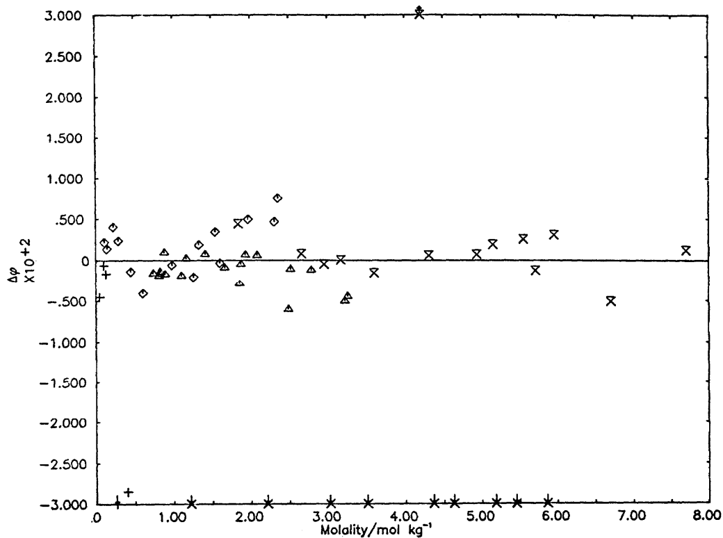
Deviation Plot For MnCl 2 : Δφ vs molality
