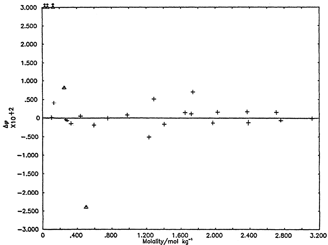
Deviation Plot For UO_2Cl_2 : \Delta\phi vs molality
