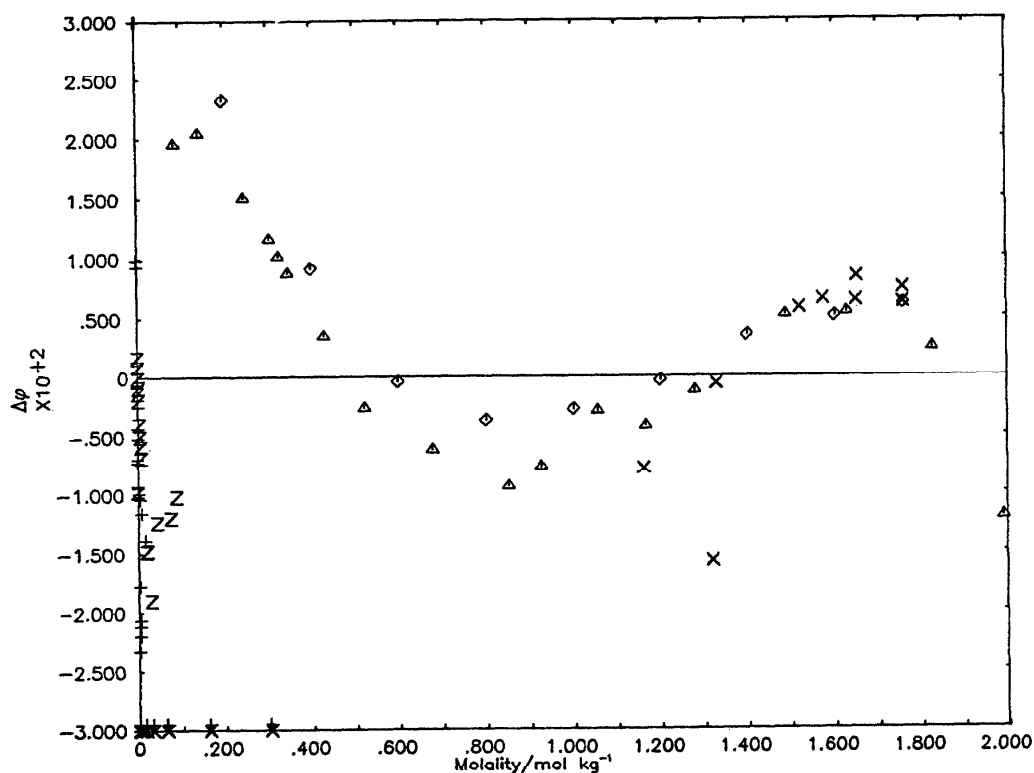
Deviation Plot for Pb(NO_3)_2 : \Delta\phi vs molality
