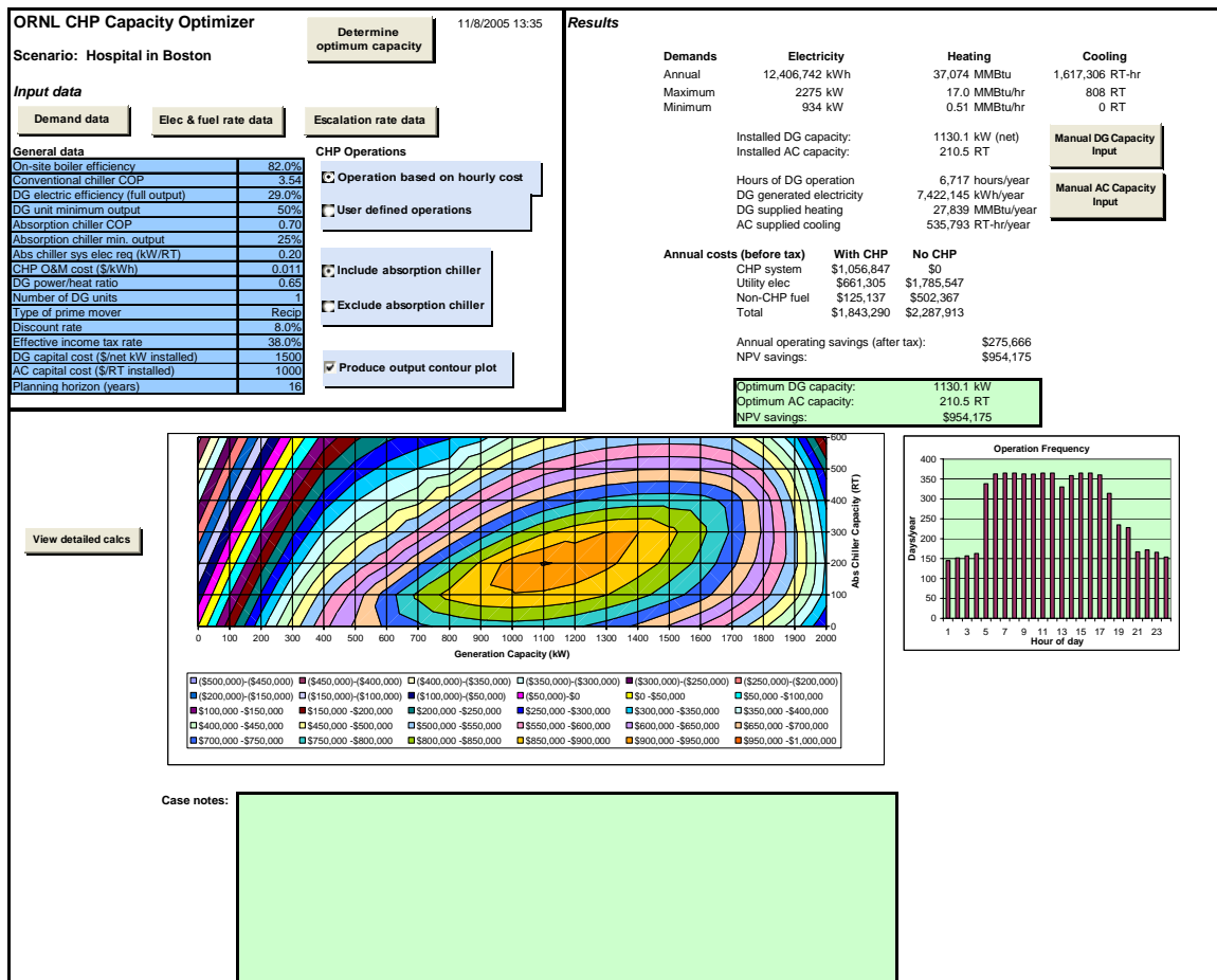
Fig. 3. Main screen of ORNL CHP capacity optimizer.
