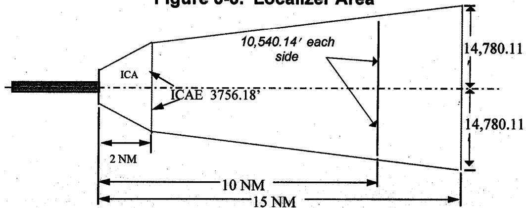
Figure 3-3. Localizer Area
