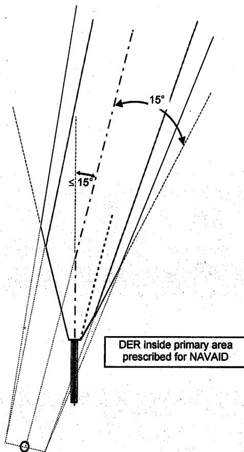
Figure 3-5. DER within Primary Area Facility
