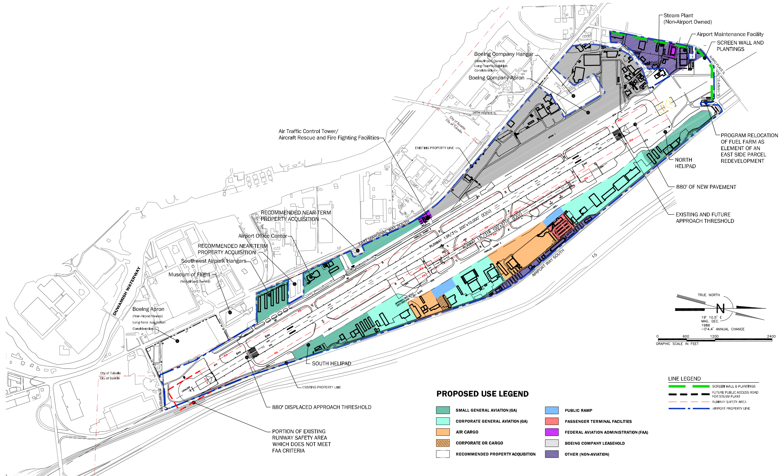
Figure D2 Conceptual Airport Development Plan
