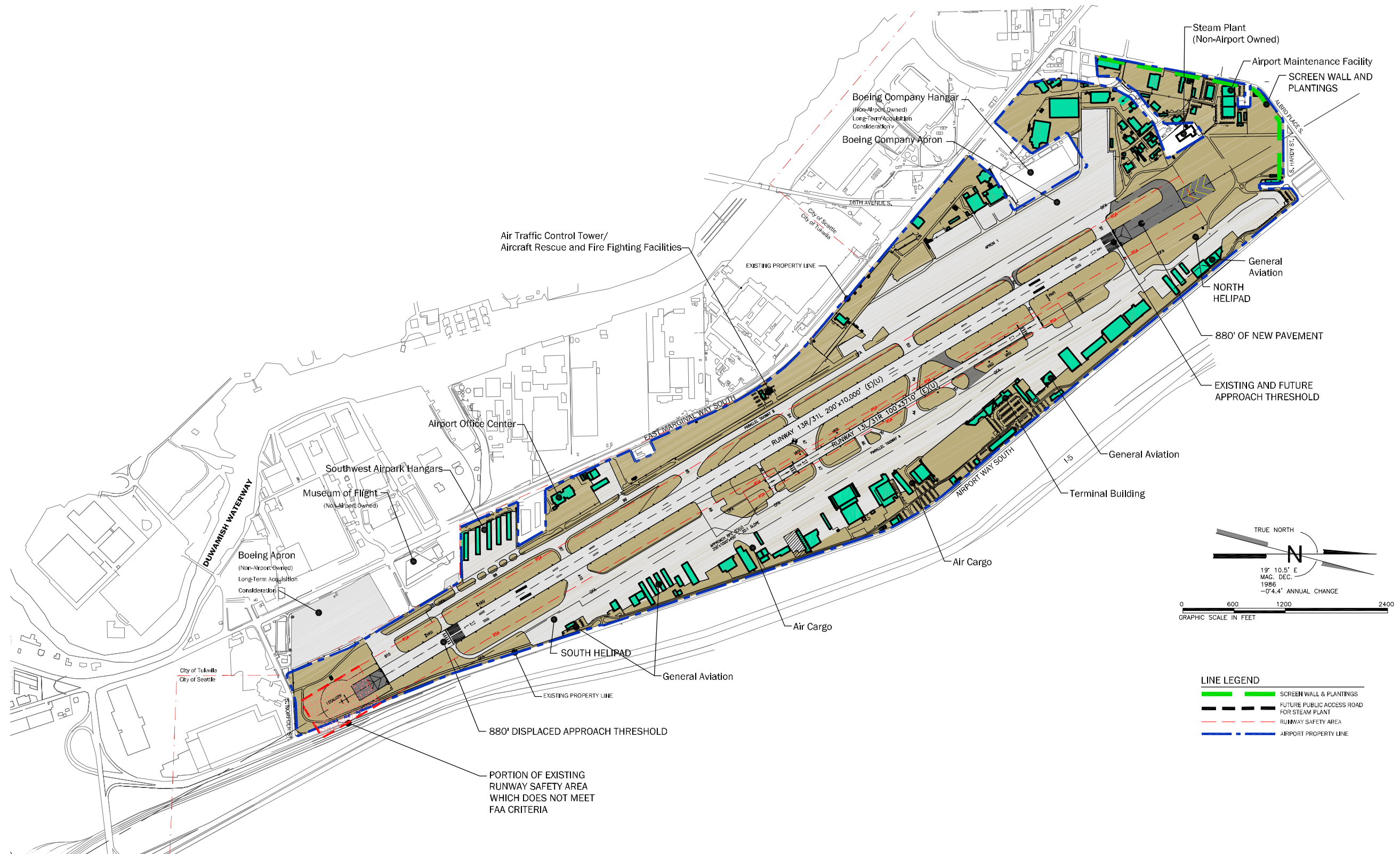
Figure D1 Airside Development Plan
