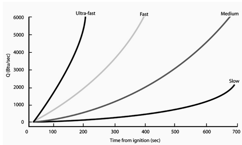
Figure 2-6 Fire Growth Rates for T 2 Fires (Btu/sec)
