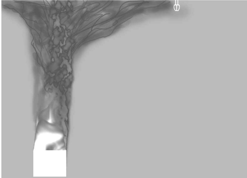
Figure 2-9 A Fire Plume and a Ceiling Jet
