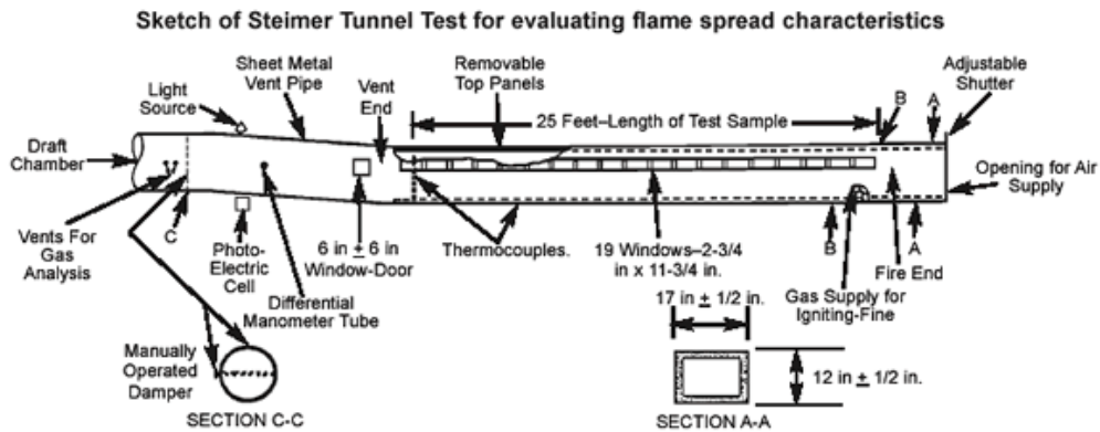
Figure 2-10 Steiner Tunnel Test Apparatus
