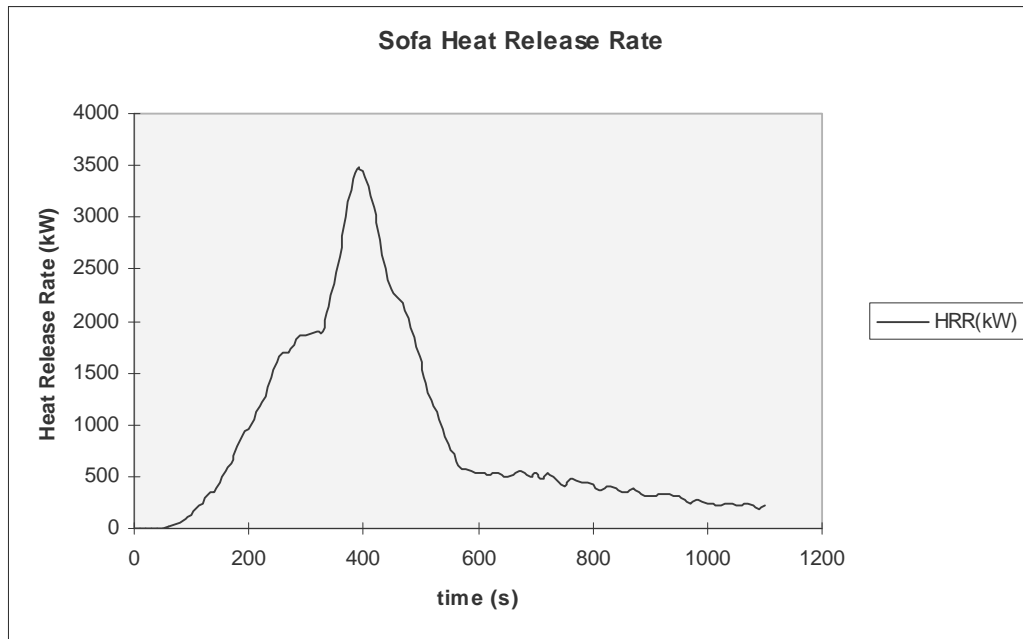
Figure 2-7 Heat Release Rate for a Sofa
