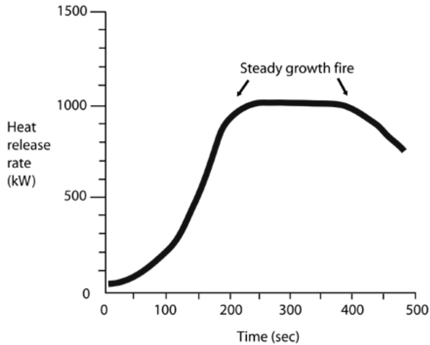
Figure 2-4 Graph of a Growing and Steady-State Fire
