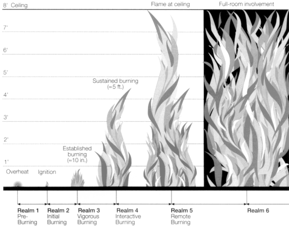
Figure 2-8 Graphic Depiction of the Fire Realms
