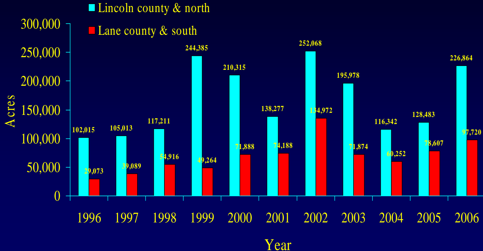
Fig. 3. Acres of Douglas-fir Forest with Swiss Needle Cast Symptoms Detected by Aerial Surveys, Coast Range, Oregon, 1996-2006
