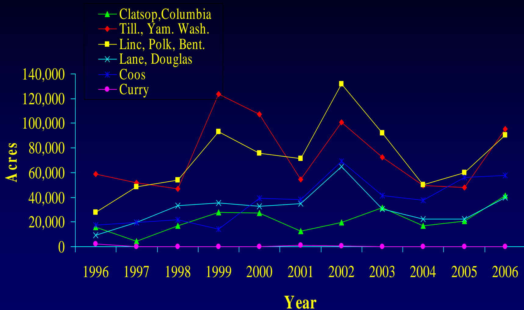
Figure 4. Acres of Douglas-fir Forest with Swiss Needle Cast Symptoms Detected by Aerial Surveys, Coast Range, Oregon, 1996-2006
