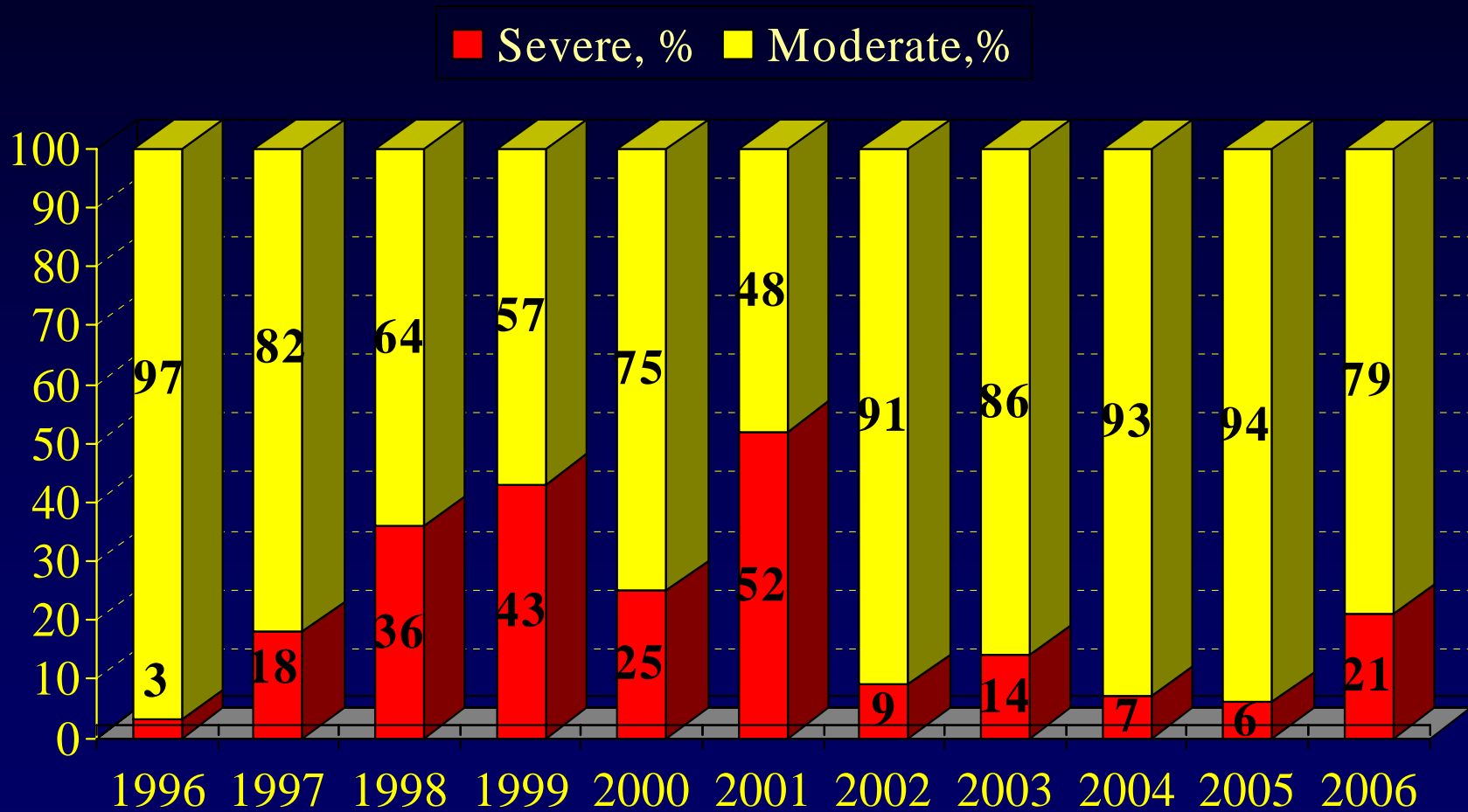
Figure 5. Swiss Needle Cast Aerial Survey, 1996-2006 Percentage of Acres classified as “Moderate “ or “Severe” Symptoms
