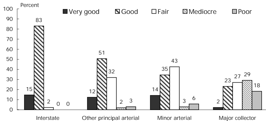
Figure 1-1: Rural Road Conditions in New Hampshire: 2000
