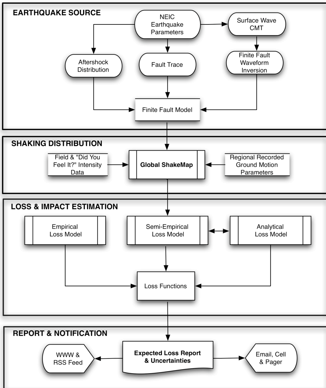
Figure 1. PAGER flowchart for operations, calibration, and loss estimation.
