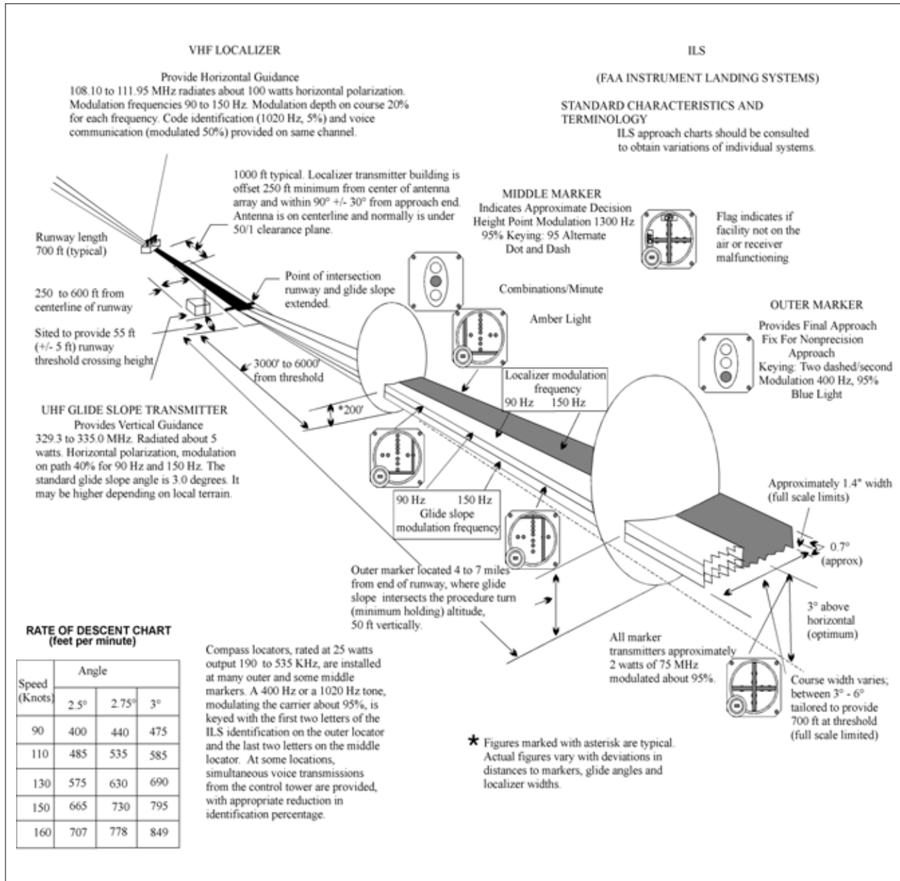
FIG ENR 4.1-2 FAA Instrument Landing Systems
