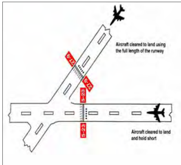
FIG ENR 1.1-4 Land and Hold Short of an Intersecting Runway
