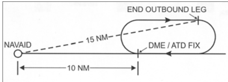
FIG ENR 1.5-4 Inbound Toward NAVAID
