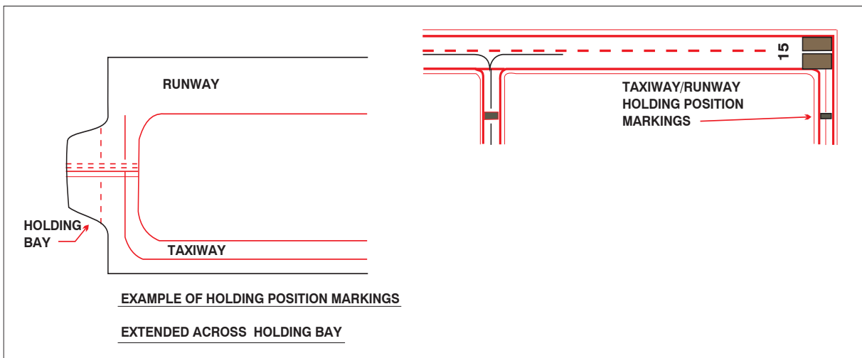
FIG AD 1.1-22 Runway Holding Position Markings on Taxiway
