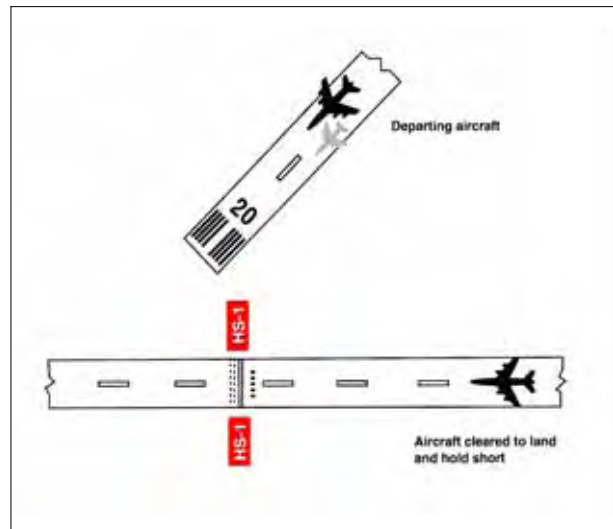
FIG ENR 1.1-6 Land and Hold Short of a Designated Point on a Runway Other Than an Intersecting Runway or Taxiway
