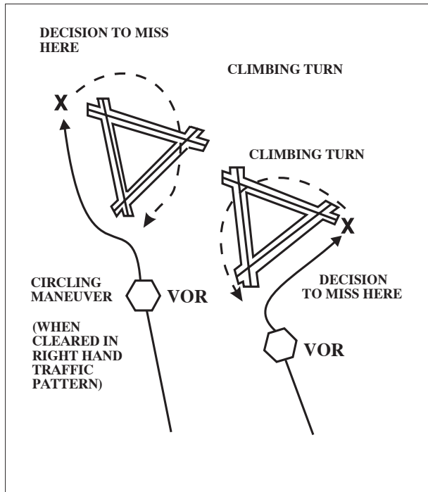
FIG 5-4-25 Circling and Missed Approach Obstruction Clearance Areas
