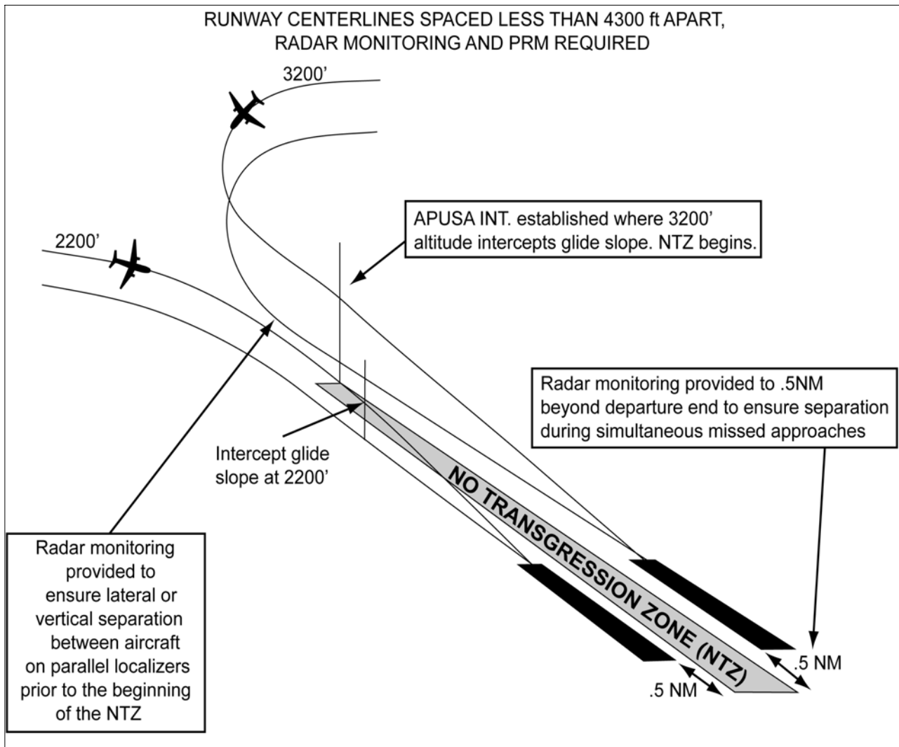
FIG 5-4-18 ILS PRM Approaches (Simultaneous Close Parallel)
