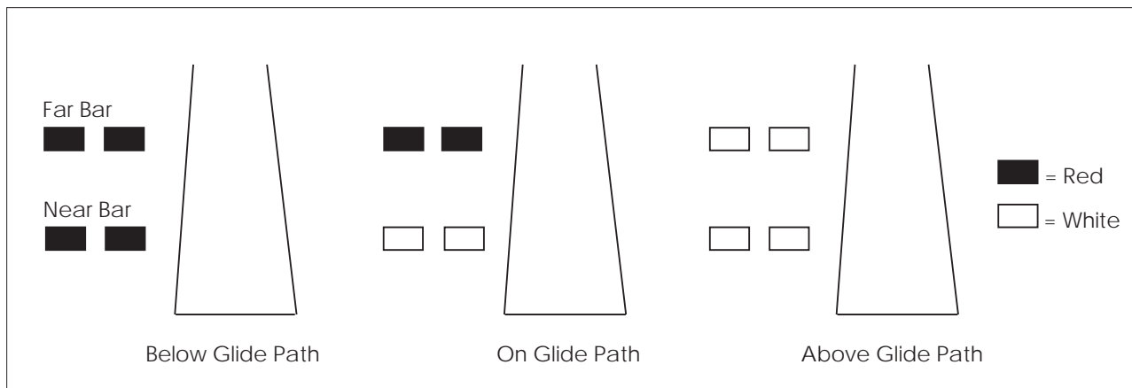
FIG 2-1-2 2-Bar VASI
