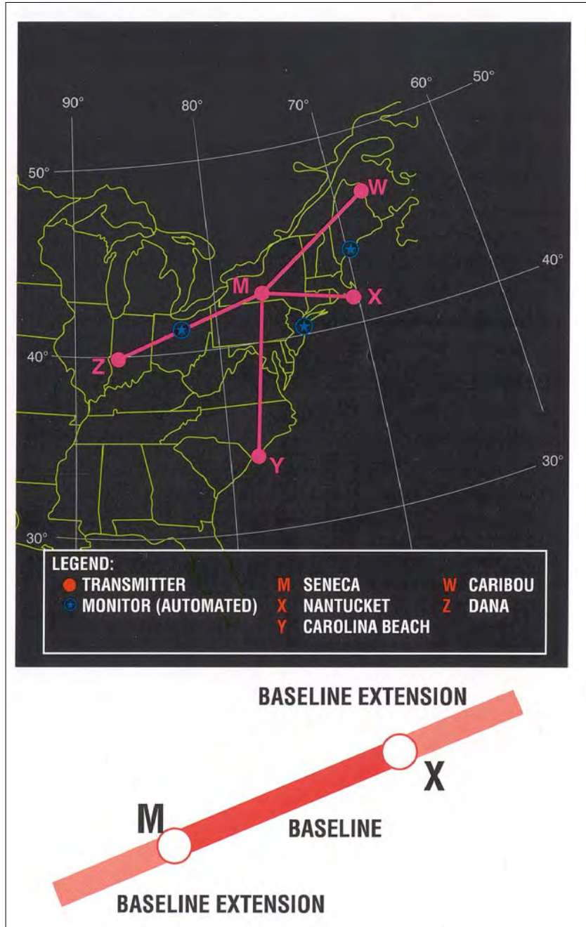
FIG 1-1-14 Northeast U.S. LORAN Chain
