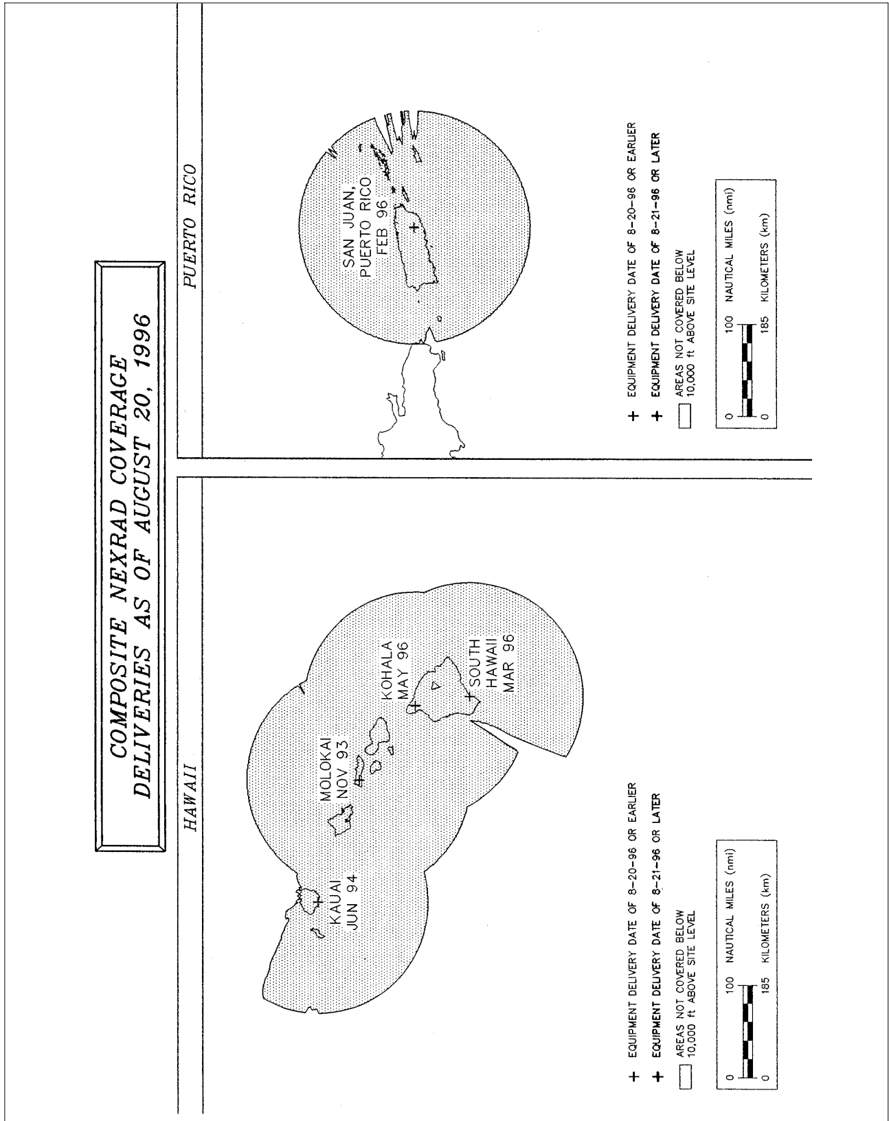
FIG 7-1-12 NEXRAD Coverage
