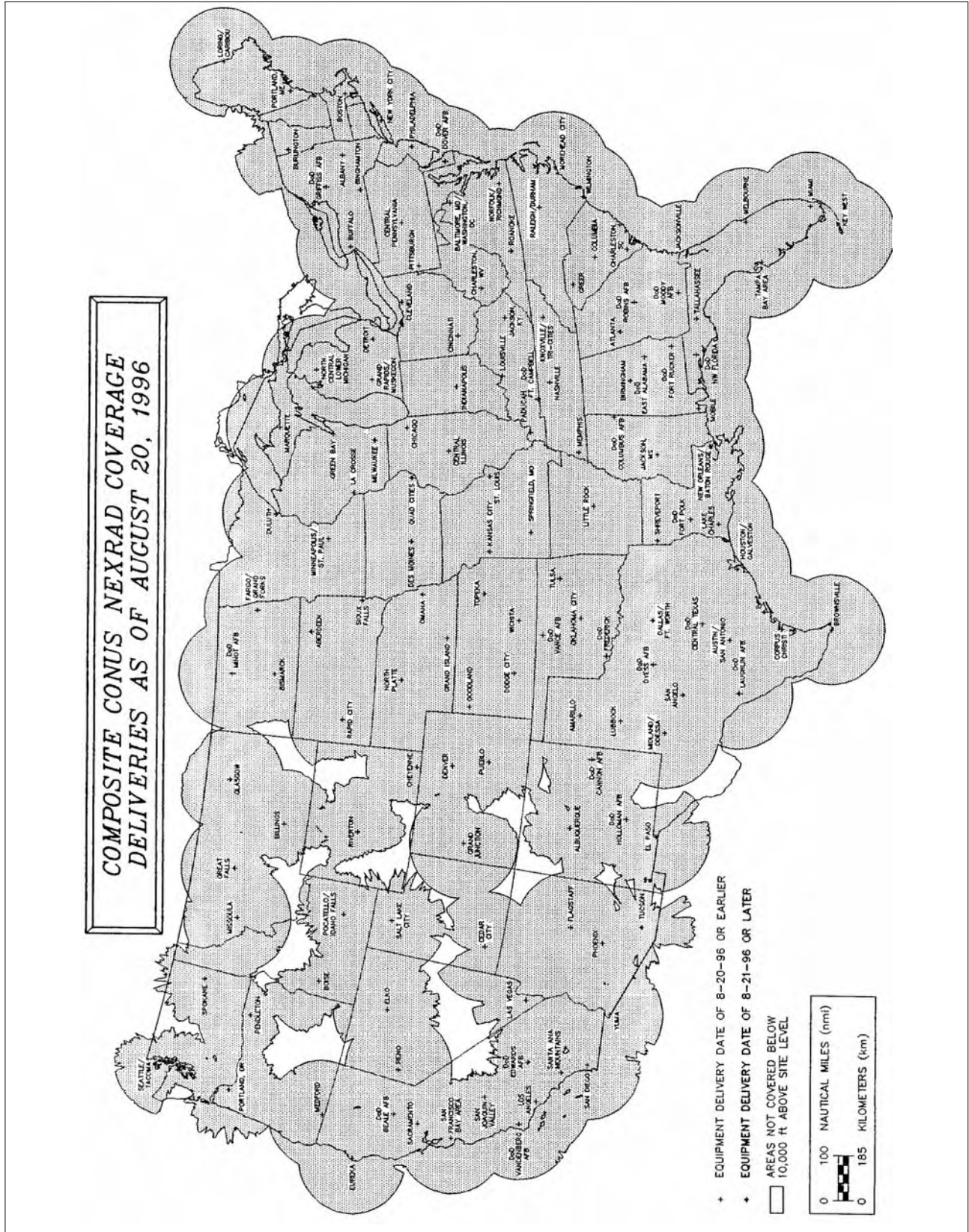
FIG 7-1-10 NEXRAD Coverage
