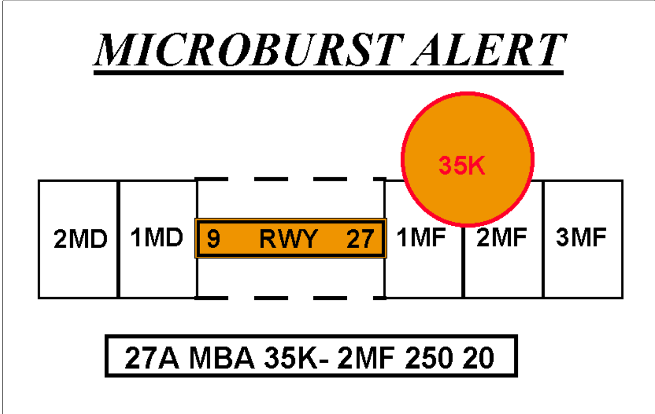
FIG 7-1-18 Microburst Alert
