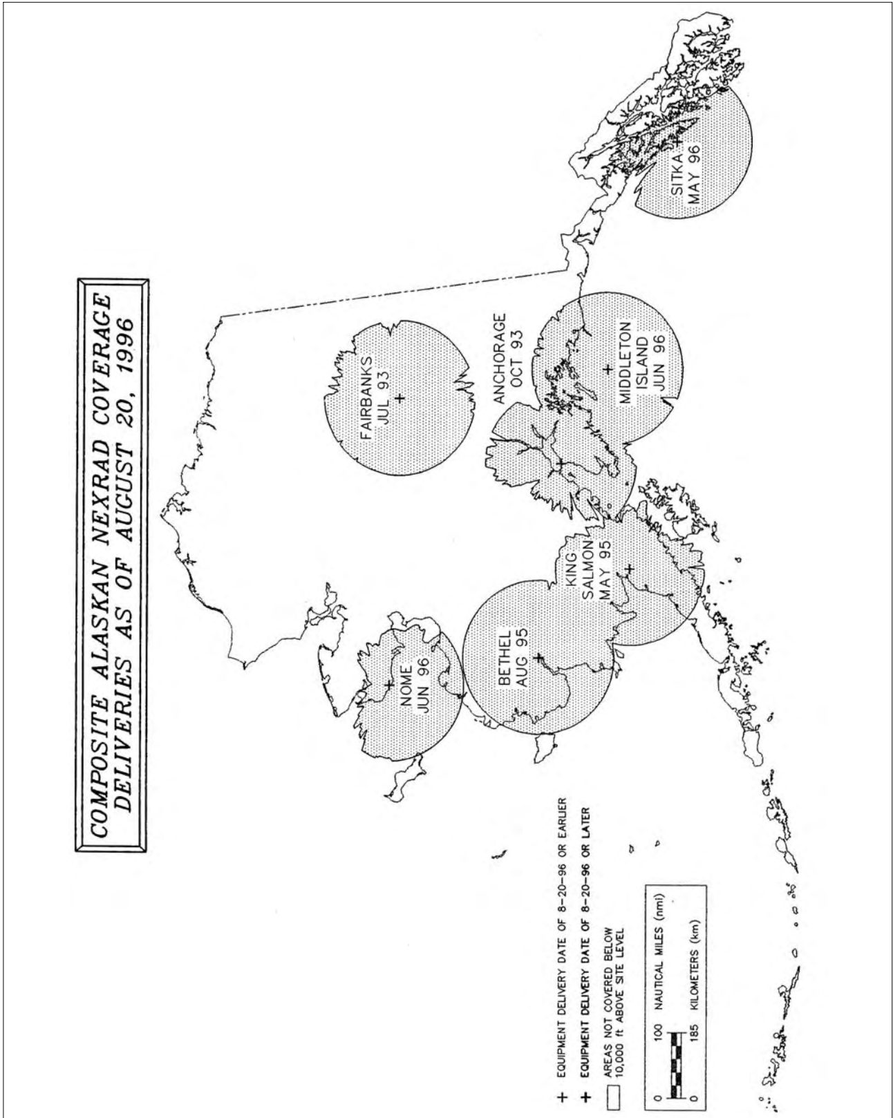
FIG 7-1-11 NEXRAD Coverage
