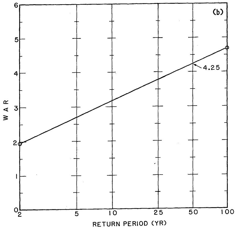
← Figure 16.—Examples of WAR return period interpolation for 41°30'N, 112°10'W, (a) 1-day amounts, and (b) 5-day amounts.
