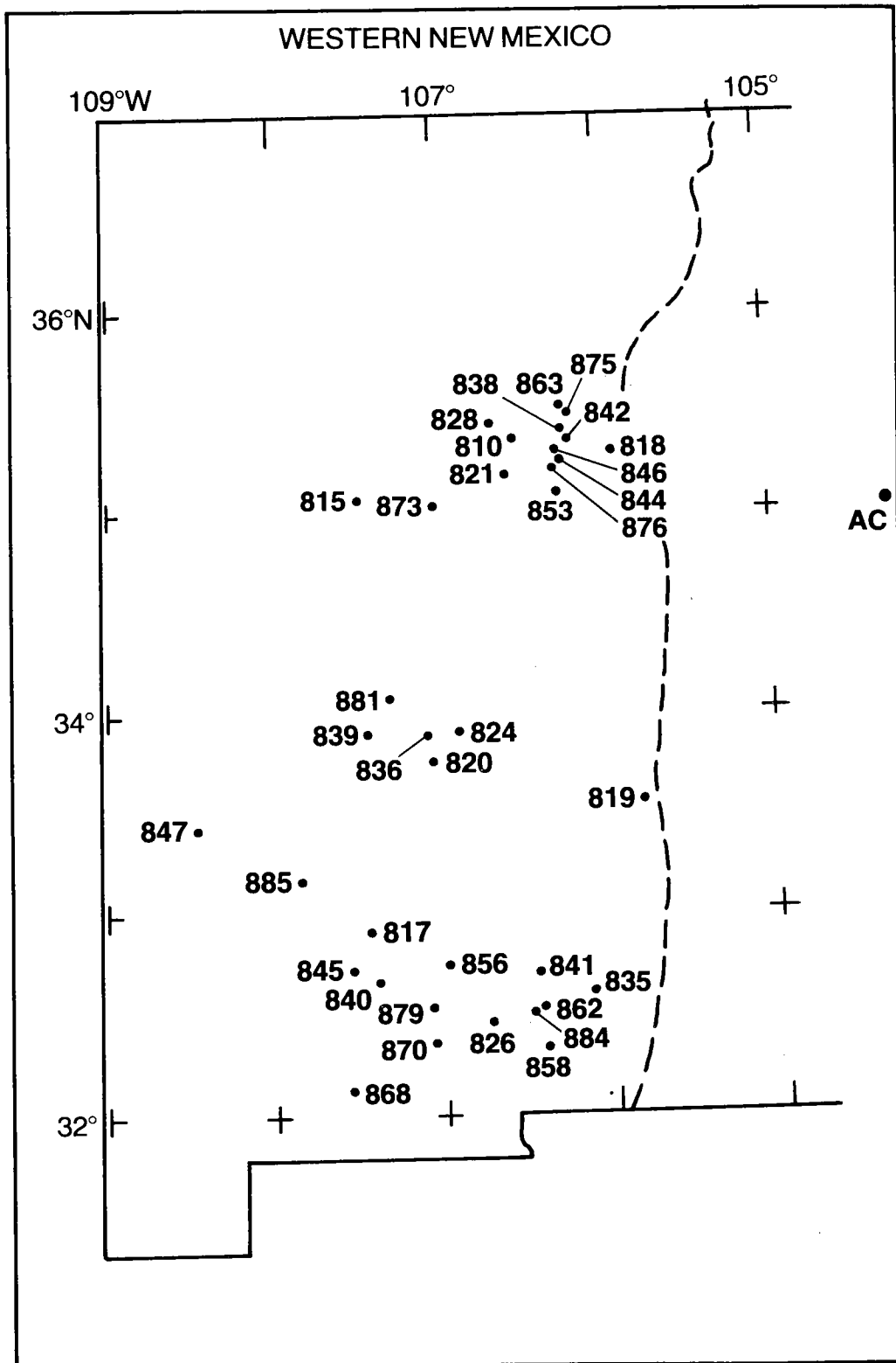
Figure 7b.--Locations of midpoints between New Mexico recorder pairs. Identification numbers are from table 3. Point labeled AC is Alamogordo Creek.
