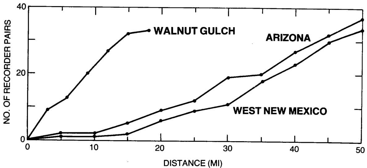
Figure 8. --Distribution of recorder-pair interstation distances for Arizona, western New Mexico, and Walnut Gulch 24-hr data. Points denote total number of pairs with interstation distance less than or equal to the plotted distance.
