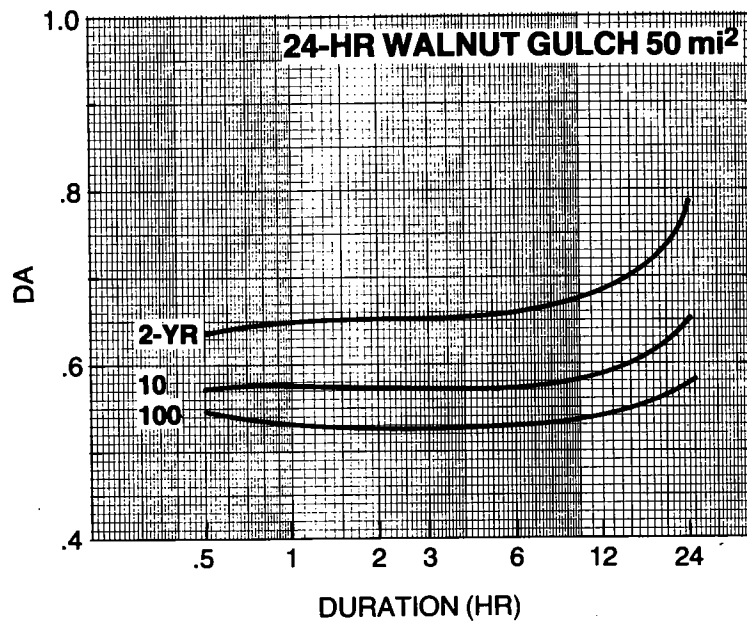
Figure 6.--Depth-area ratio vs. duration at 50 mi 2 (129.5 km 2 ) for 2-, 10-, and 100-yr return periods. The 24-hr Walnut Gulch results are combined with the Walnut Gulch depth-area ratios for 30 min, 1-hr, 2-hr, and 6-hr from Osborn et al. (1980).
