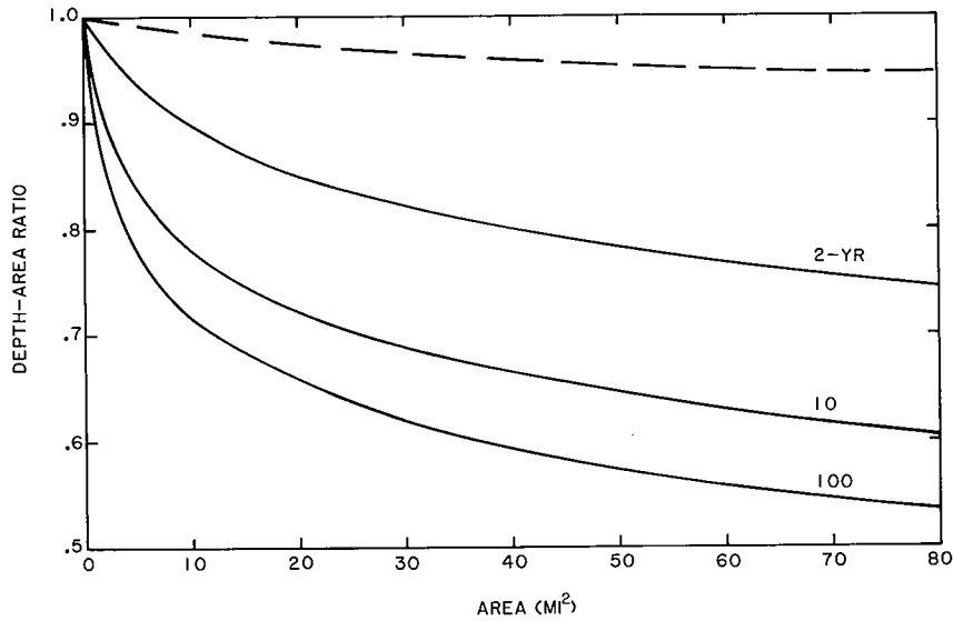
Figure 5.--24-hr depth-area ratio at Walnut Gulch for 2-, 10-, and 100-yr return periods. The dashed line is the NOAA Atlas 2 (Miller et al. 1973) 24-hr depth-area curve.
