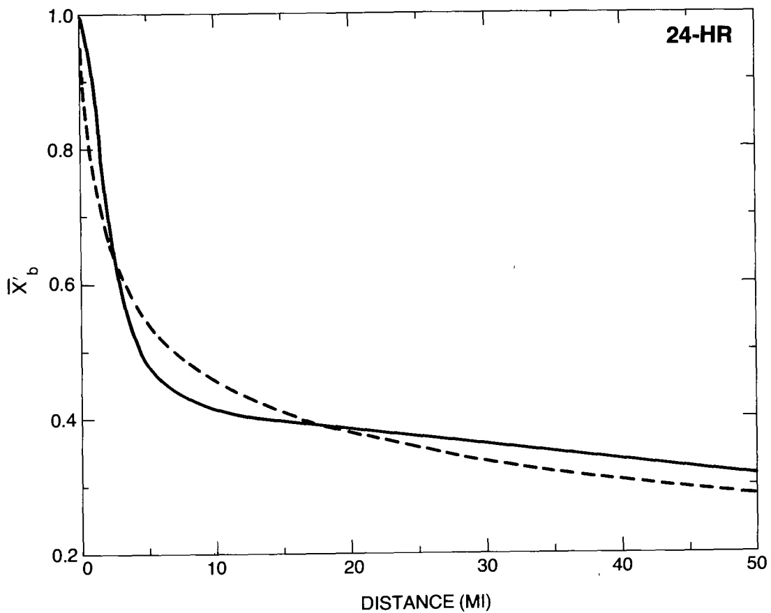
Figure III-2.--Same as figure III-1, except for \bar{X}'_b .
