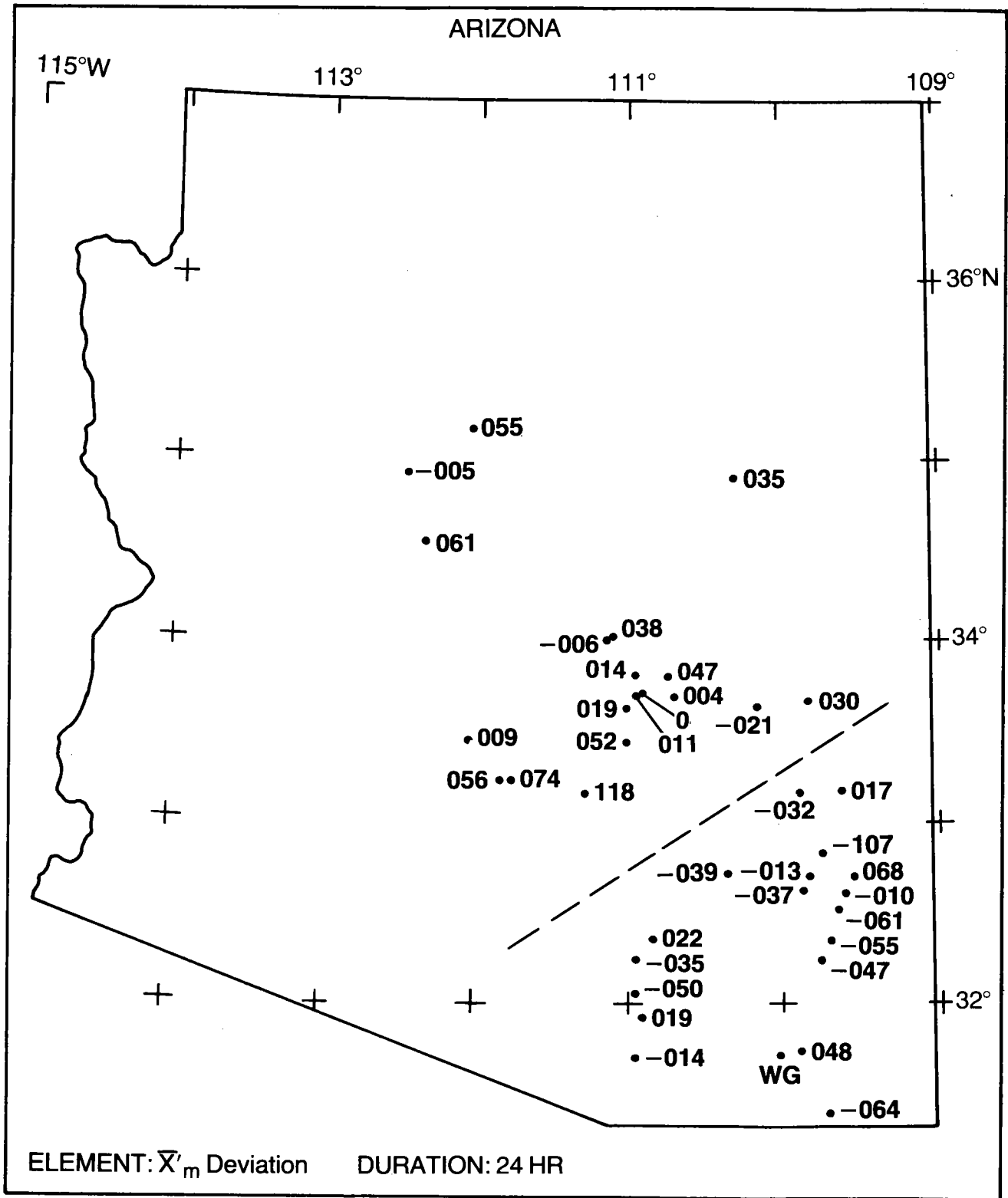
Figure 11a.--Deviation ( \times 10^{-3} ) of \bar{X}'_m from the fitted curve for the 24-hr duration in Arizona.
