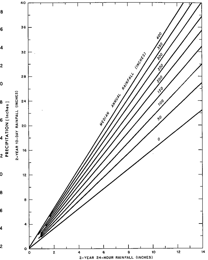
FIGURE 4.—Relation for estimating 2-year 10-day rainfall.
