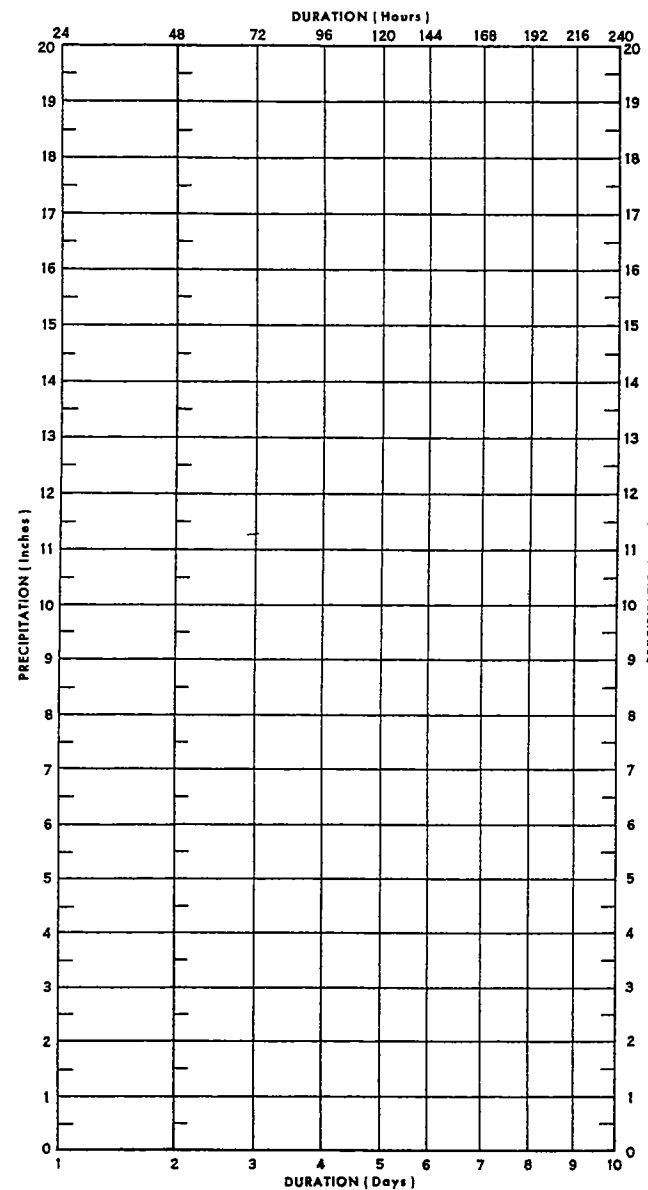
FIGURE 3.—Duration-interpolation diagram.
