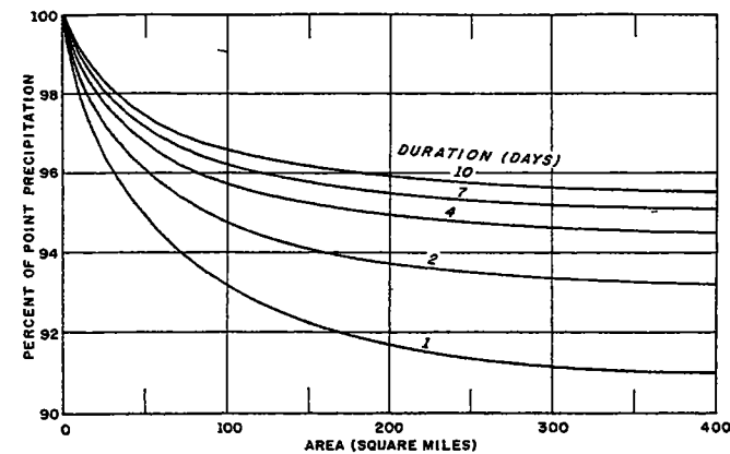
FIGURE 10.—Depth-area curves.
