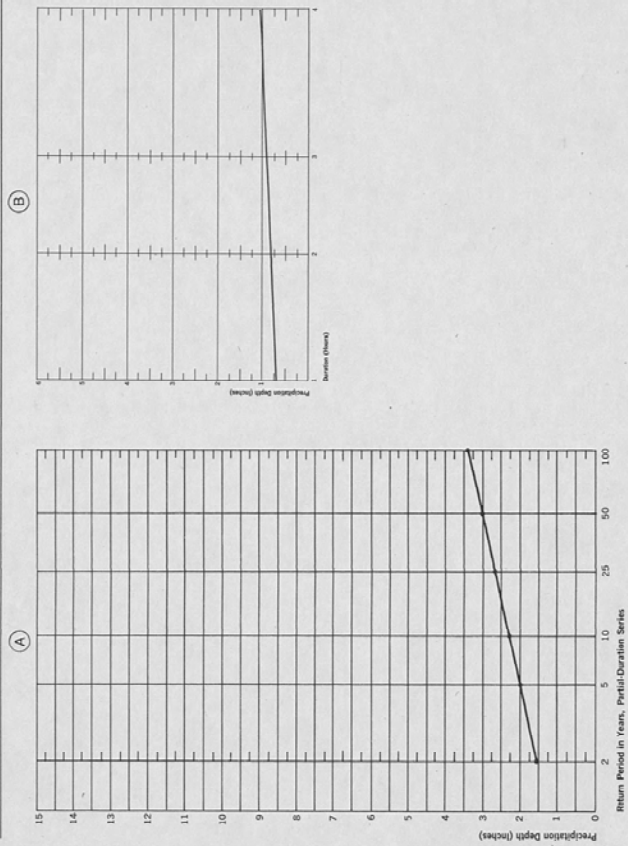
Figure 18. Illustration of use of precipitation-frequency diagrams using values from precipitation-frequency maps and relations at 105°00' W., 39°00' N.
