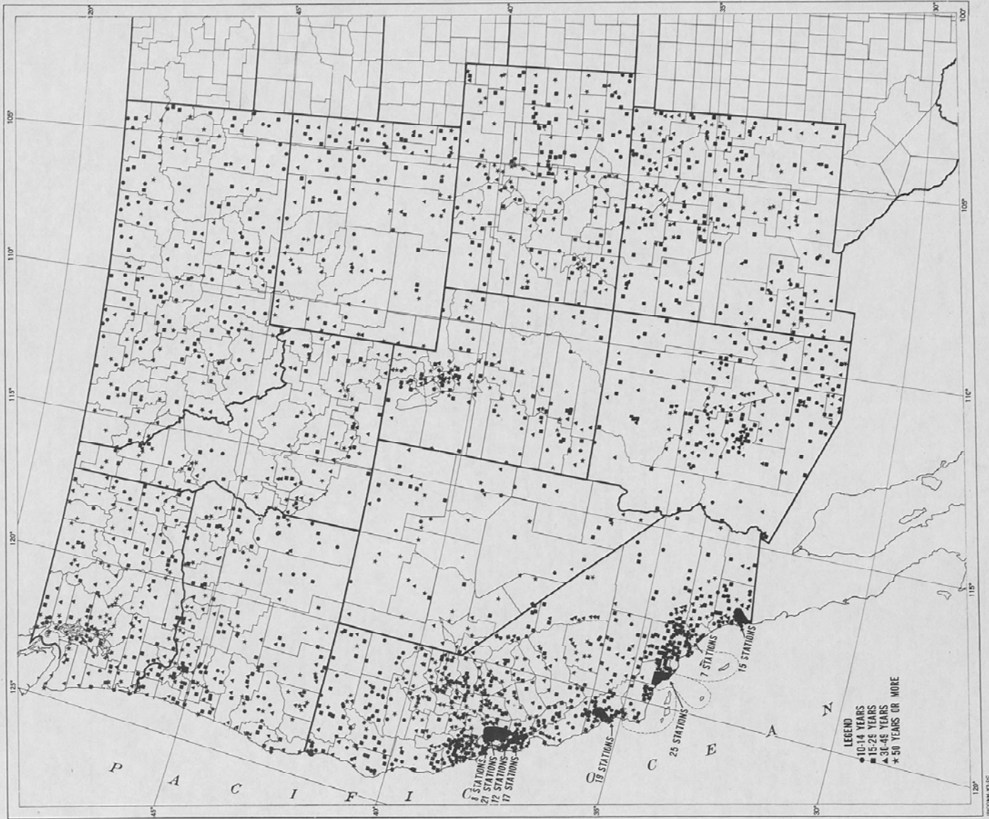
Figure 4. Geographic distribution of stations with recording gages. Symbols indicate total length of record available.
