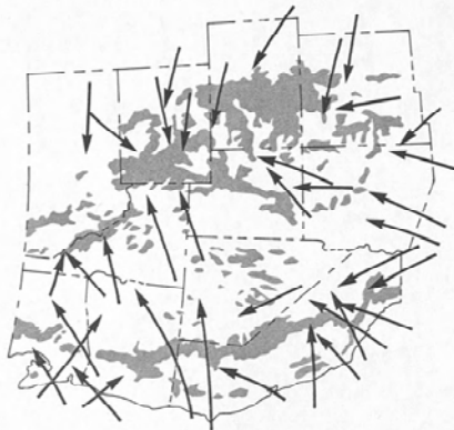
Figure 7. Principal paths of moisture inflow in the western United States for storms producing large precipitation amounts. Toned areas are major orographic barriers.
