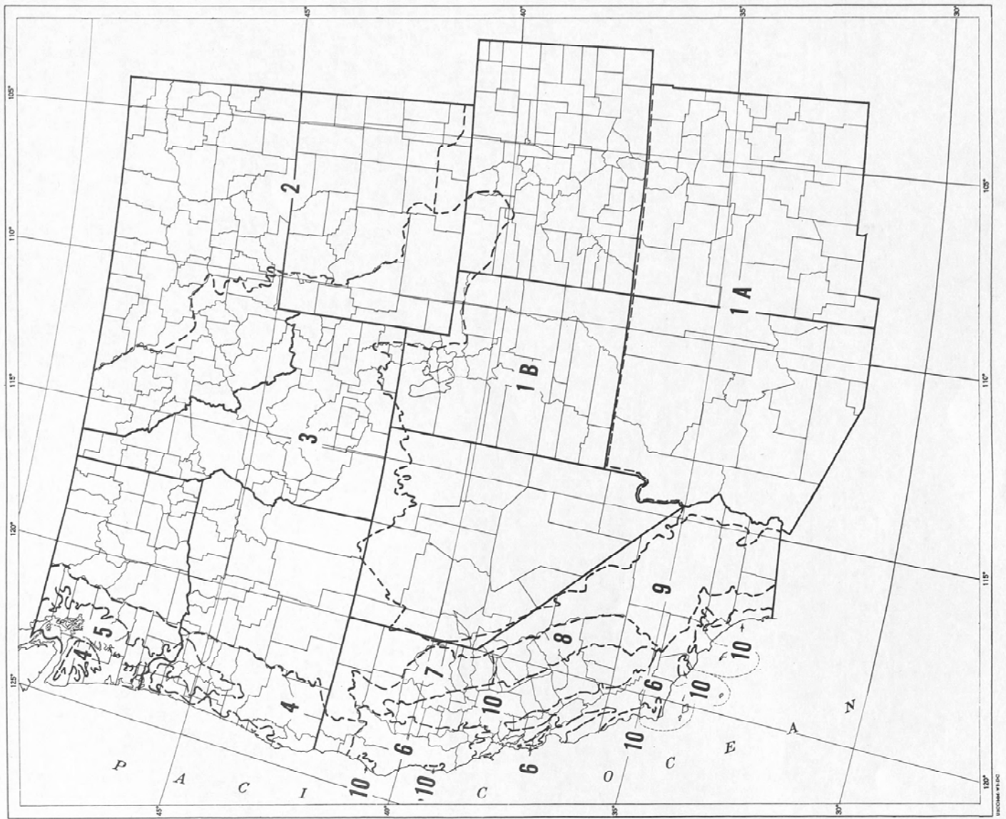
Figure 10. Regions used to develop statistical parameters for interpolation of 2-yr and 100-yr 6-hr precipitation values.
