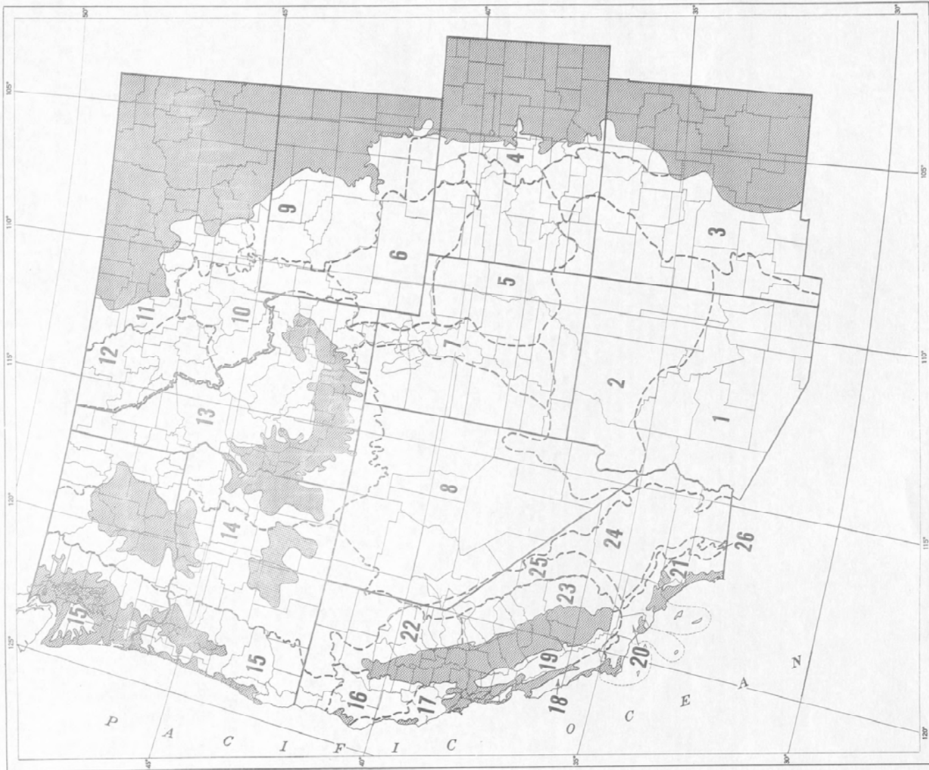
Figure 8. Regions used to develop statistical parameters for interstation interpolation of 2-yr 24-hr precipitation values.
