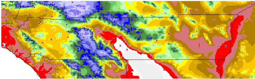
Locations of Riverside County stations used in development of the PRISM 1961-1990 mean annual precipitation (MAP) grids. Background is 1-km elevation grid.
