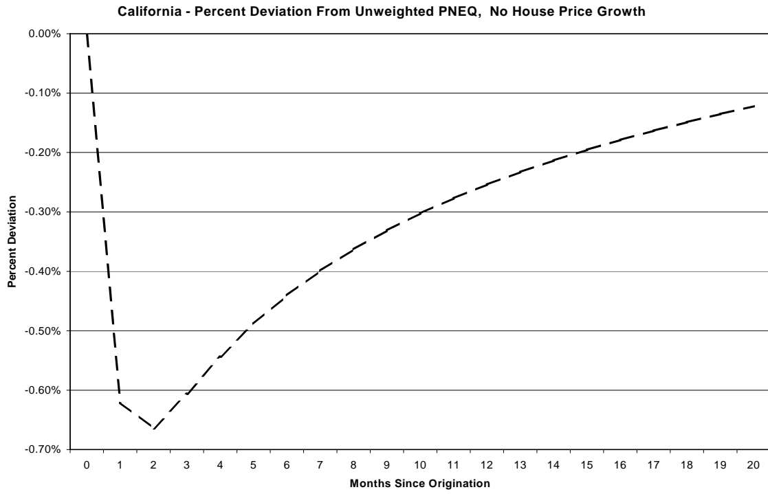
Figure 2: PNEQ Deviations
