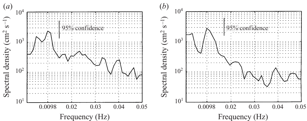
FIGURE 9. Averaged energy spectra of (a) cross-shore velocities and (b) longshore velocities measured at x = 11.43 m, 11.63 m, 11.93 m, y = 13.03 m, 13.63 m, 14.24 m (test E, runs E1–3; 819.2 s < t < 1638.4 s), \Delta f = 0.0012 Hz, d.o.f. = 18.
