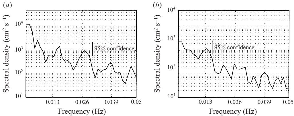
FIGURE 10. Averaged energy spectra of (a) cross-shore velocities and (b) longshore velocities measured at x = 11.43 \text{ m}, 11.63 \text{ m}, 11.93 \text{ m} , y = 13.03 \text{ m}, 13.63 \text{ m}, 14.24 \text{ m} (test G, runs G1–3; 819.2 \text{ s} < t < 1638.4 \text{ s} ), \Delta f = 0.0012 \text{ Hz} , d.o.f. = 18.
