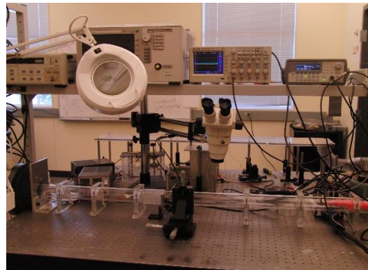
Unsteady wall pressure flow measurements
