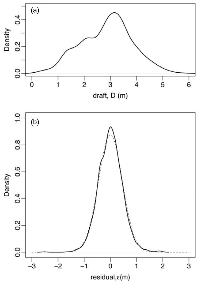
Figure 7. (a) The probability density function of observations of 50-km-mean ice drafts, with a standard deviation of 0.99 \text{ m} . (b) The probability density function of residuals \varepsilon from the OLS fit to (2), with a standard deviation of 0.46 \text{ m} , along with a Gaussian distribution (dashed) with the same standard deviation for comparison. The functions were generated using a kernel density estimator with bandwidths of 0.1907 and 0.8756 .
