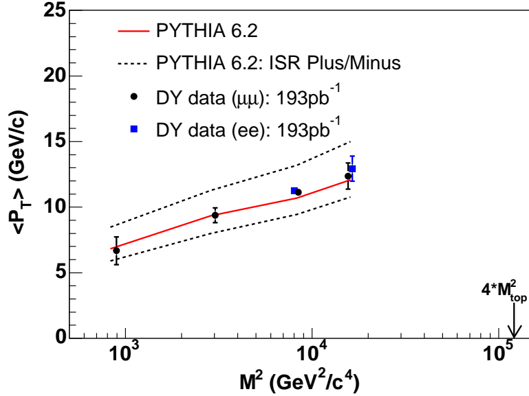
FIG. 32: The average p_T of dilepton system, which corresponds to the level of ISR activity, shows a logarithmic dependence on the dilepton invariant mass M_{\ell\ell}^2 . The data are compared with the predictions of PYTHIA 6.2 and of the +1\sigma_{ISR} and -1\sigma_{ISR} samples.
