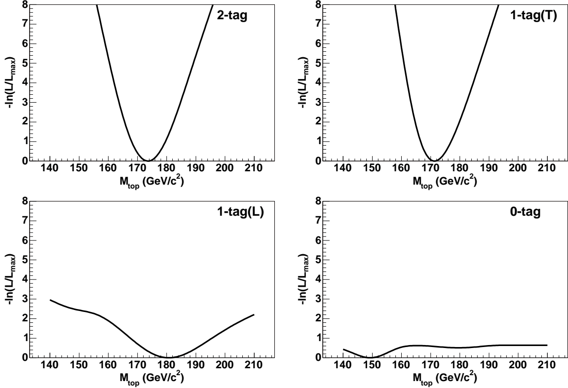
FIG. 22: The negative log-likelihood curves as a function of the top quark mass are shown for the M_{\text{top}} -only fit to each subsample in the data. Upper left: 2-tag events; upper right: 1-tag(T) events; lower left: 1-tag(L) events; lower right: 0-tag events.
