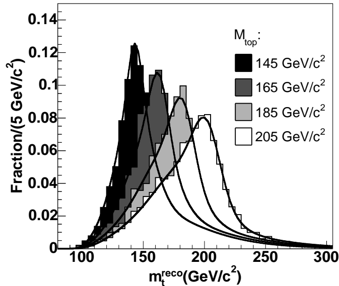
FIG. 11: Four m_t^{\text{reco}} signal templates for the 1-tag(T) sample are shown, with top quark masses ranging from 145 \text{ GeV}/c^2 to 205 \text{ GeV}/c^2 and with JES set to 0. Overlaid are the fitted parameterizations at each generated mass, taken from the full parameterization given in Eq. V.1.
