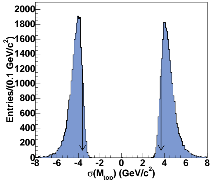
FIG. 21: The distributions of positive and negative uncertainties from the likelihood fit are shown, for pseudo-experiments generated with a top quark mass of 172.5 \text{ GeV}/c^2 , the nominal jet energy scale, and the number of events in each subsample as observed in the data. Arrows indicate the positive and negative uncertainties from the likelihood fit to the data; 9.2% of the pseudo-experiments have smaller uncertainties.
