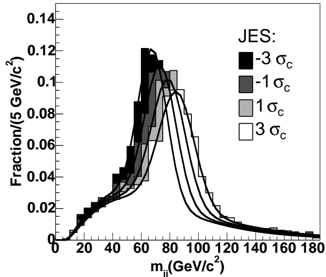
FIG. 12: Four m_{jj} signal templates for the 2-tag sample are shown, with JES values ranging from -3\sigma to 3\sigma and with the top quark mass set to 180\text{ GeV}/c^2 . Overlaid are the fitted parameterizations at each value of jet energy scale, taken from the full parameterization given in Eq. V.1.
