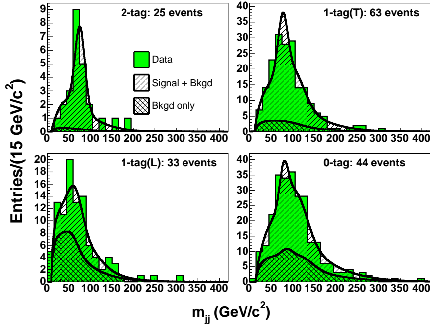
FIG. 20: The reconstructed dijet mass distribution for each subsample is shown overlaid with the expected distribution using the top quark mass, jet energy scale, signal normalization, and background normalization from the combined fit.
