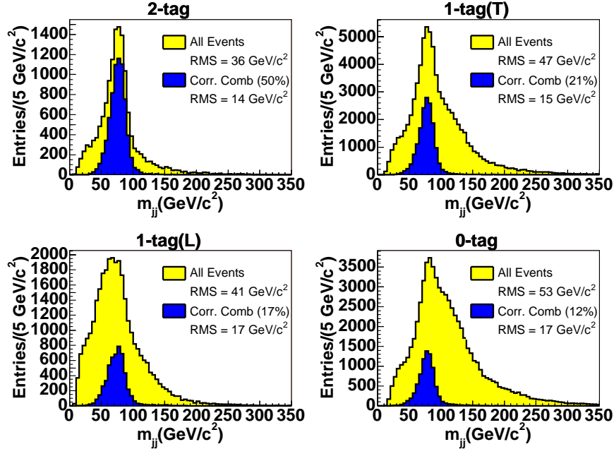
FIG. 8: The reconstructed dijet mass distributions for the 178 \text{GeV}/c^2 HERWIG t\bar{t} sample at the nominal jet energy scale. Overlaid are darker histograms of the reconstructed mass distributions using the subset of events for which the leading four jets include two jets matched (within \Delta R = 0.4 ) to the two quarks from the hadronic W decay, and plotting just the invariant mass of those two jets. Distributions are shown for 2-tag (upper left), 1-tag(T) (upper right), 1-tag(L) (lower left), and 0-tag (lower right) events.
