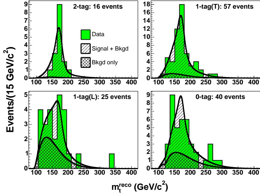
FIG. 19: The reconstructed top quark mass distribution for each subsample is shown overlaid with the expected distribution using the top quark mass, jet energy scale, signal normalization, and background normalization from the combined fit.
