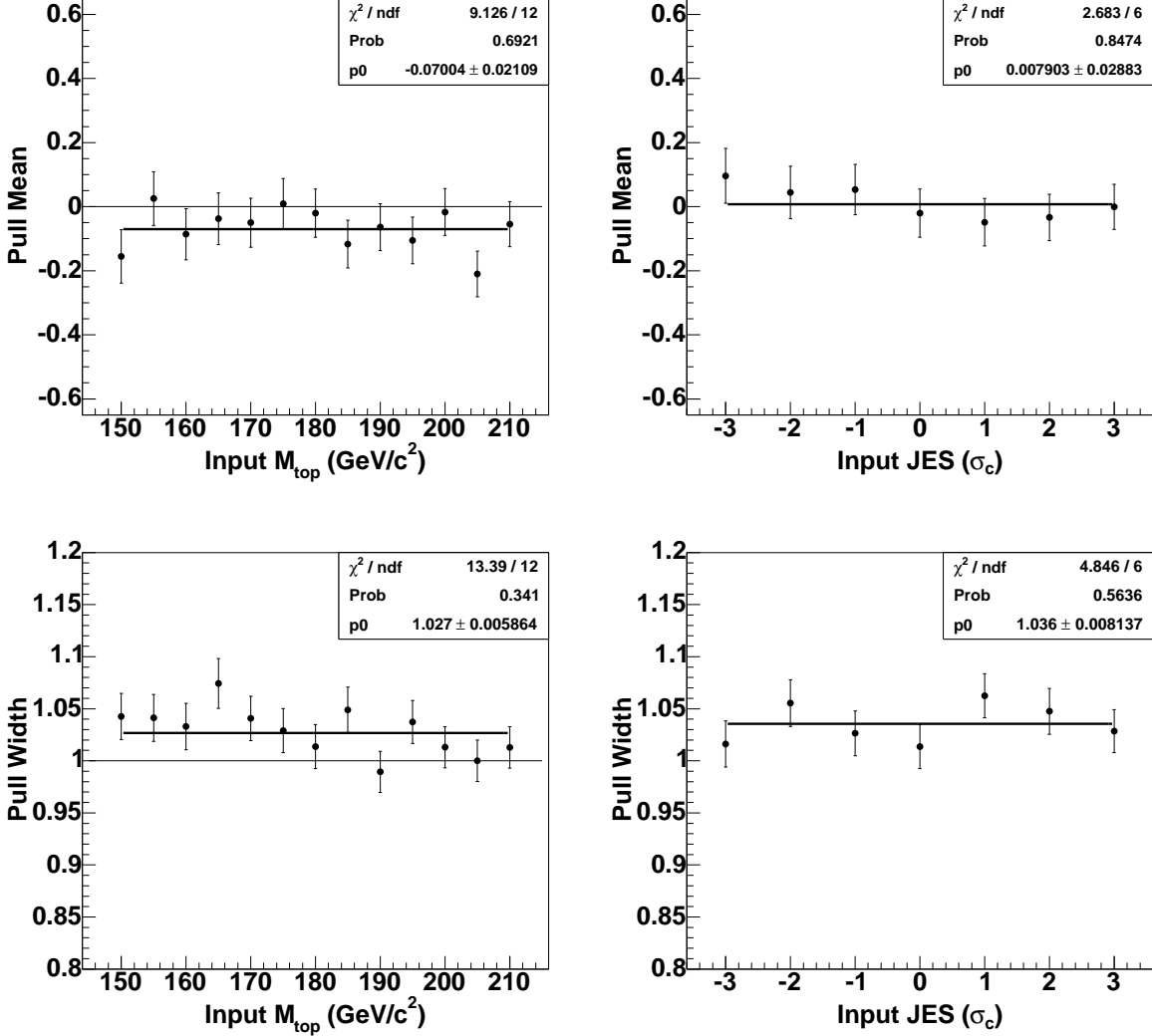
FIG. 16: The mean (top) and width (bottom) of pull distributions from sets of 2500 pseudo-experiments are shown. On the left, the jet energy scale is fixed at its nominal value, and the generated top quark mass is varied from 150 \text{ GeV}/c^2 to 210 \text{ GeV}/c^2 . On the right, the top quark mass is fixed at 180 \text{ GeV}/c^2 , and the input jet energy scale is varied from -3 \sigma to +3 \sigma . The error bars come mostly from the limited statistics of the Monte Carlo samples from which the pseudodata is taken.
