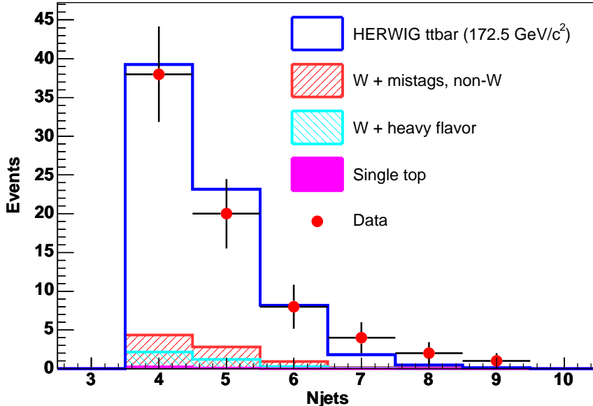
FIG. 31: The number of jets distribution for 73 signal candidate events (2-tag and 1-tag(T) sub-samples), compared to the prediction from HERWIG t\bar{t} signal events (with generated top quark mass of 172.5 \text{ GeV}/c^2 ) and simulated background events. Jets are required to have E_T > 8 \text{ GeV} and |\eta| < 2.0 .
