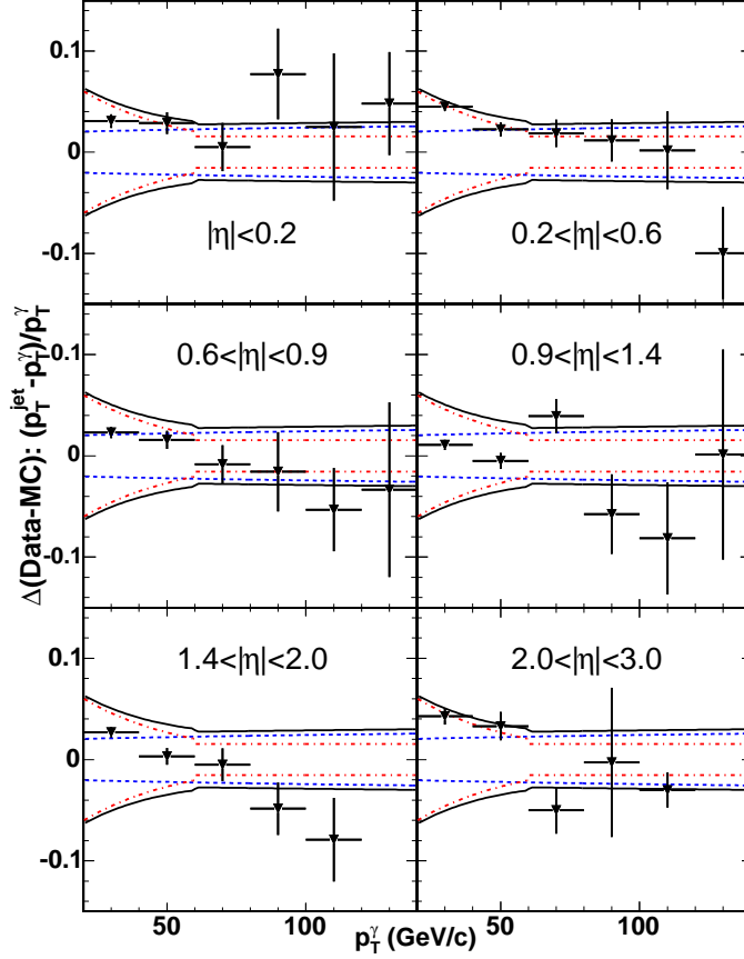
FIG. 6: For \gamma -jet events in both data and simulation, we find the fractional difference in p_T between the jet and the photon after all jet corrections are applied. Plotted here, for different ranges of jet \eta , is the difference between this quantity in data and simulated events as a function of photon p_T . The solid lines show the \pm 1 \sigma range given by the jet energy systematics. The other lines follow the same definitions as in Fig. 5.
