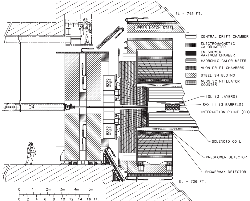
FIG. 1: An elevation view of the CDF Run II detector. From the collision region outwards, CDF consists of a silicon strip detector, a tracking drift chamber, an electromagnetic calorimeter, a hadronic calorimeter, and muon chambers.
