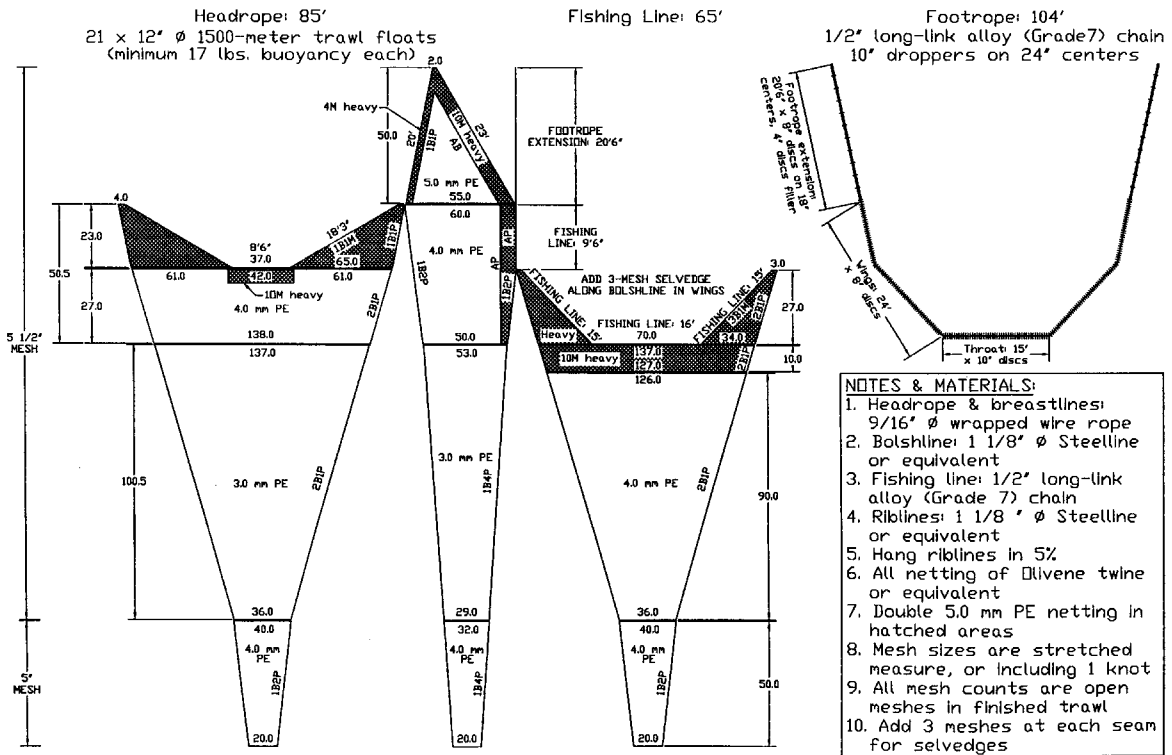
Figure 1. NMFS 85/104/5.5' Aberdeen sampling trawl
