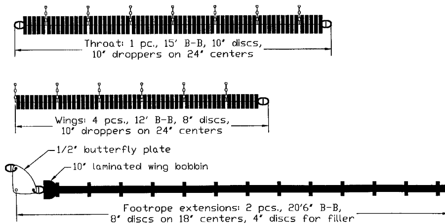
Figure 2. Footrope for NMFS 85'/104' Aberdeen Sampling Trawl 7 sections, 104' L.O.A.
