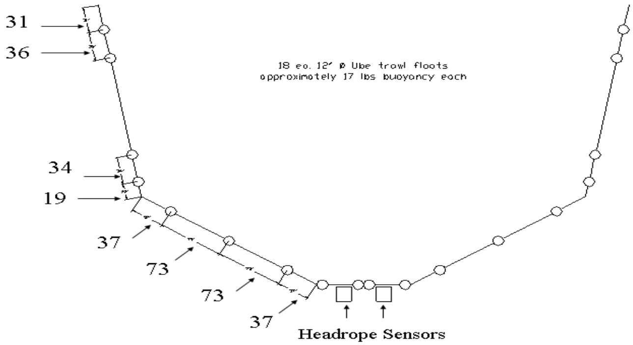
Float Placement on Aberdeen Trawl
