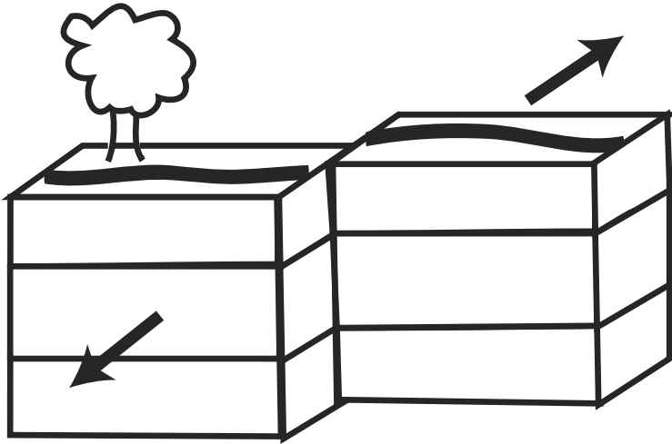
Strike-slip
