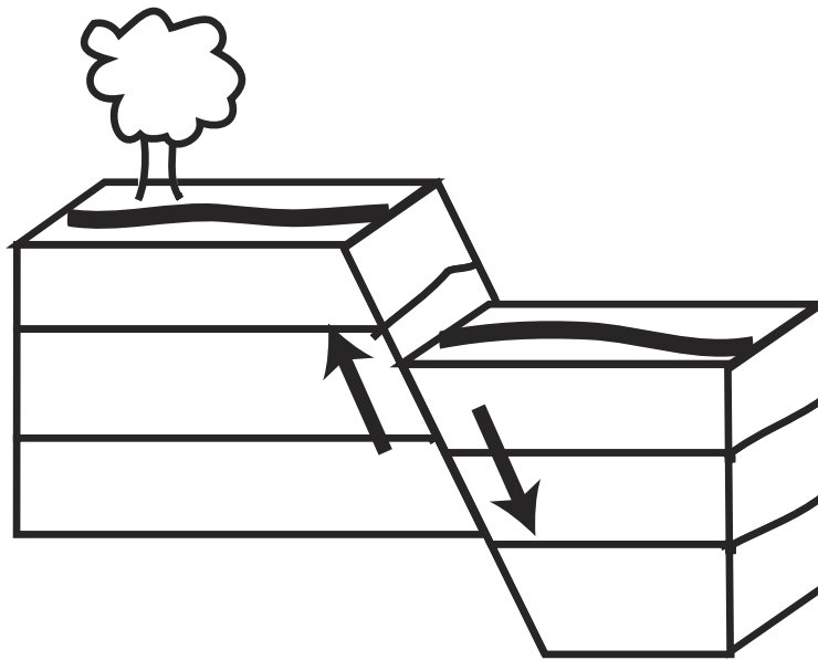
Normal
