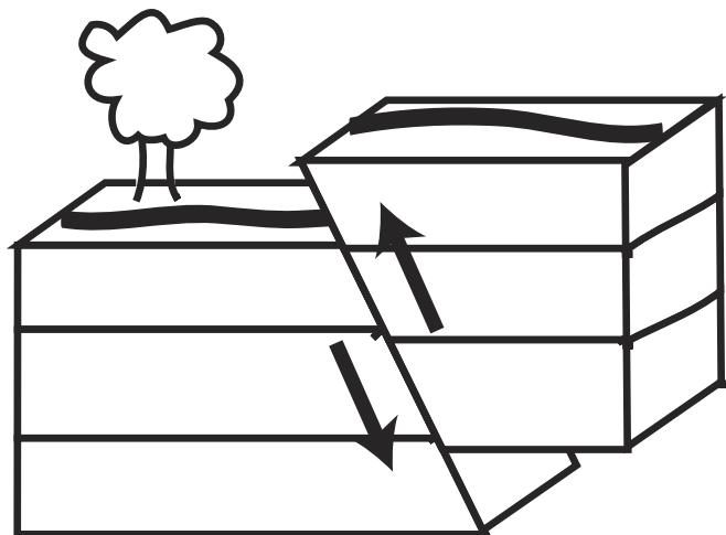
Thrust
