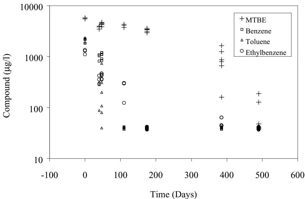
Figure 2.6 Comparison of the time lags for removal of MTBE, and of benzene, toluene, and ethylbenzene in microcosms constructed with all the compounds present together.
