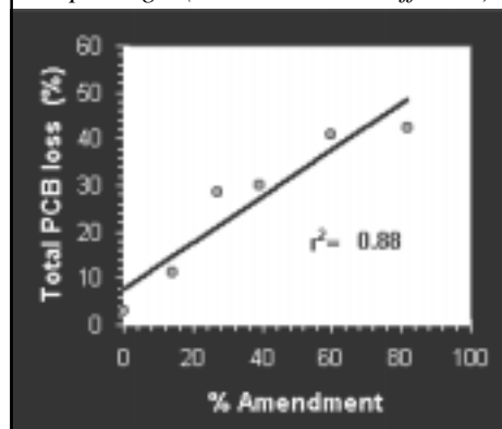
Figure 2. Effect of Amendment Addition on the Extent of PCB Degradation during Composting. ( r = correlation coefficient)
