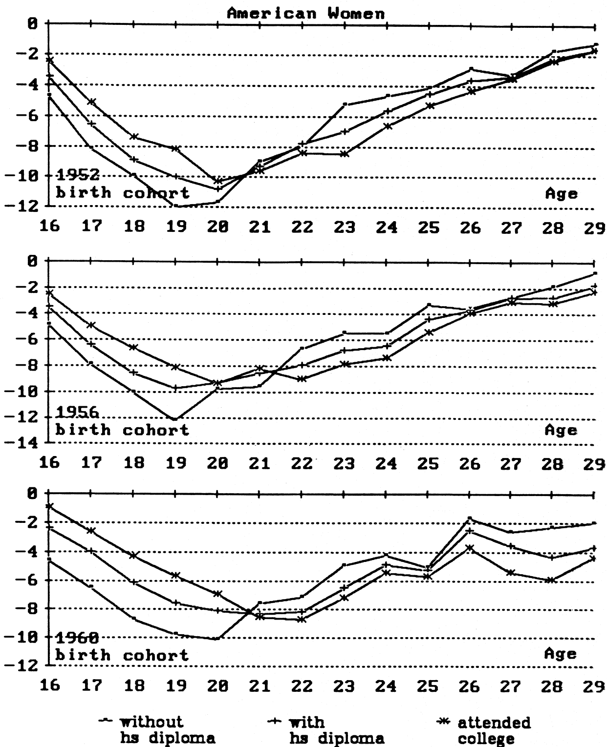
Figure 2: Relative Fluctuations in Pool of Partners
