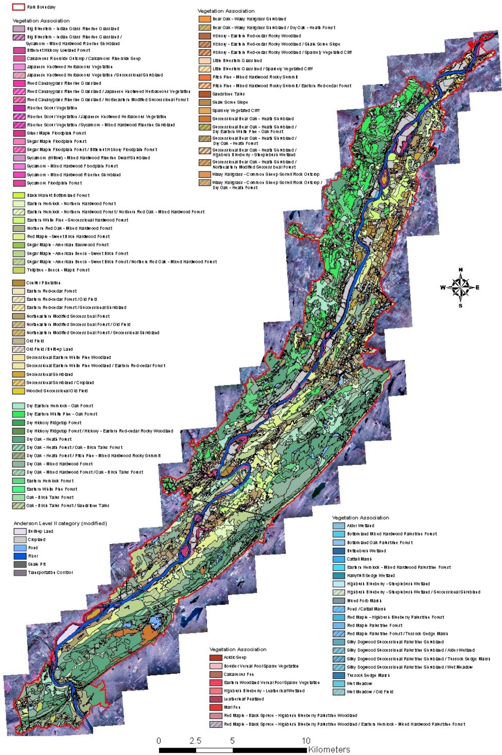
Figure 8. Vegetation associations and Anderson level II categories (modified) in Delaware Water Gap National Recreation Area.
