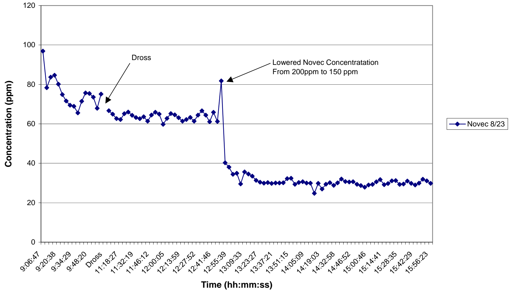
Time Series Plot for Novec™-612 on 8/23/06
