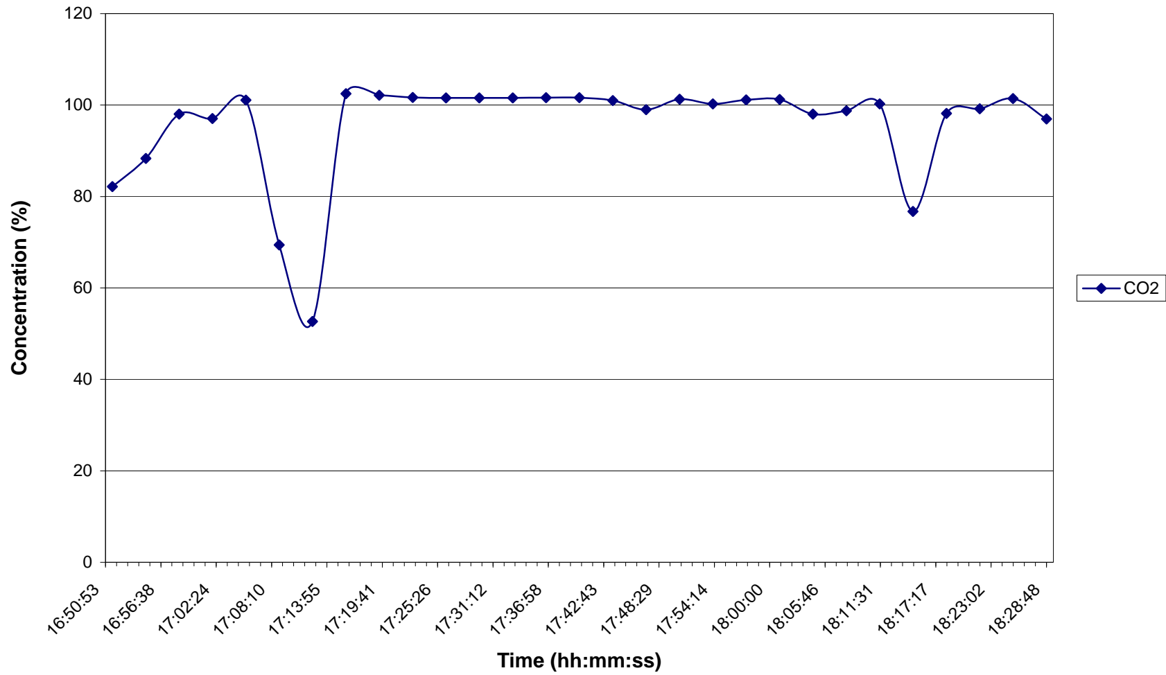
Time Series Plot of CO 2 During CO 2 Injection on 8/29/06
