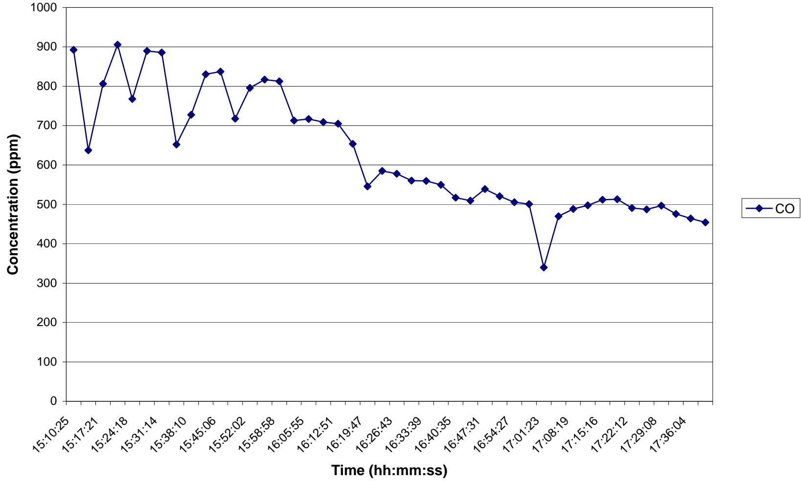
Time Series Plot for CO During HFC-134a Injection at 4200 ppm on 8/24/06
