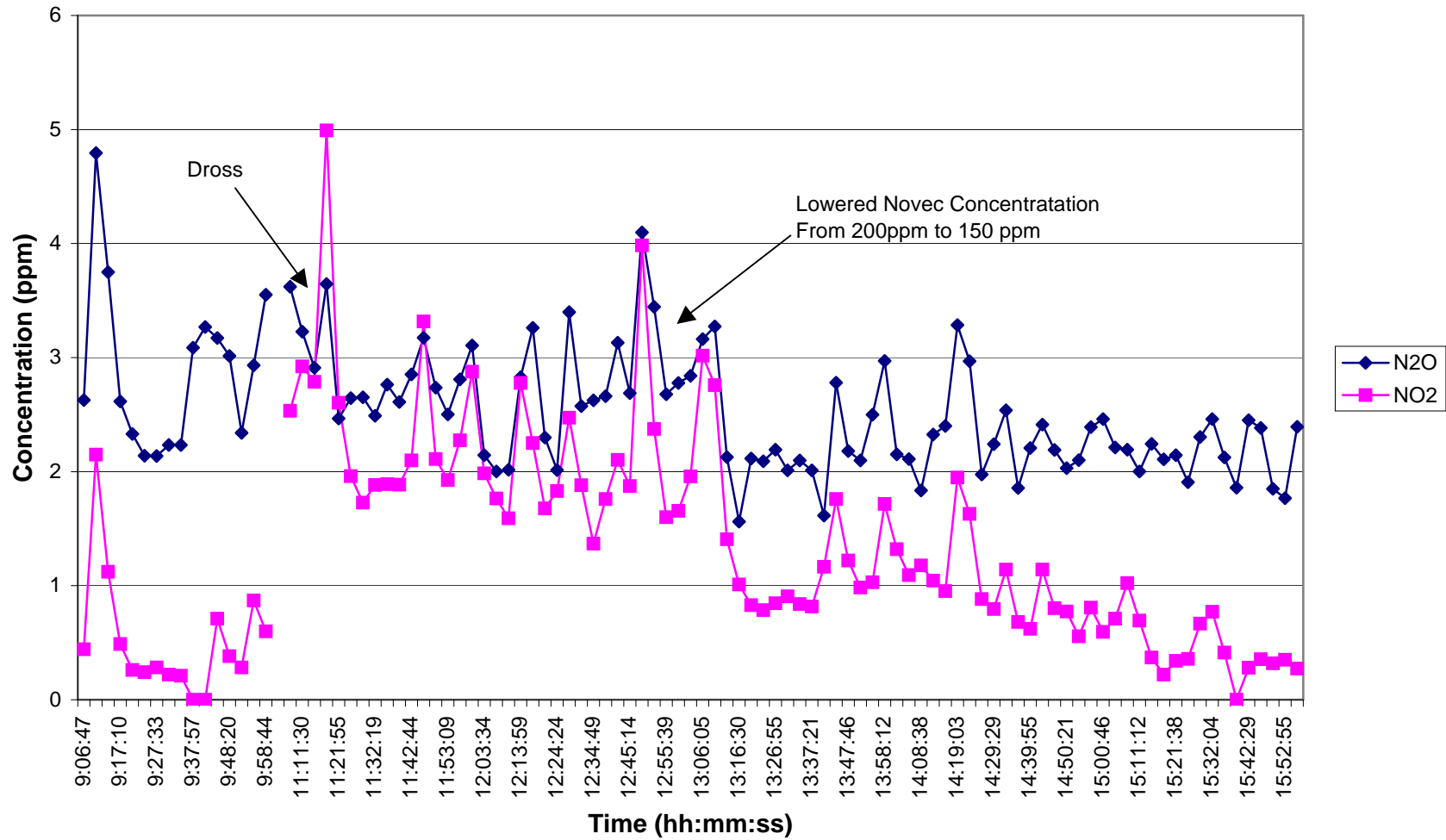
Time Series Plot for Nitrogen Oxides Using Novec™-612 Cover Gas on 8/23/06
