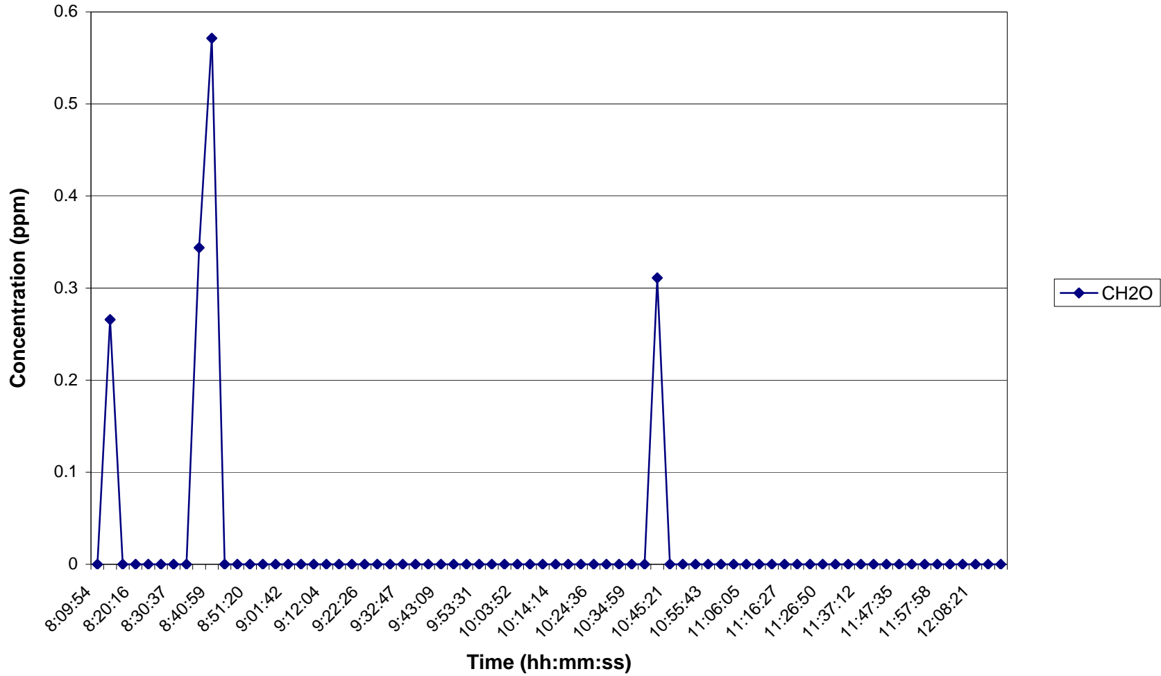
Time Series Plot for CH2O During HFC-134a Injection at 3600 ppm on 8/25/06
