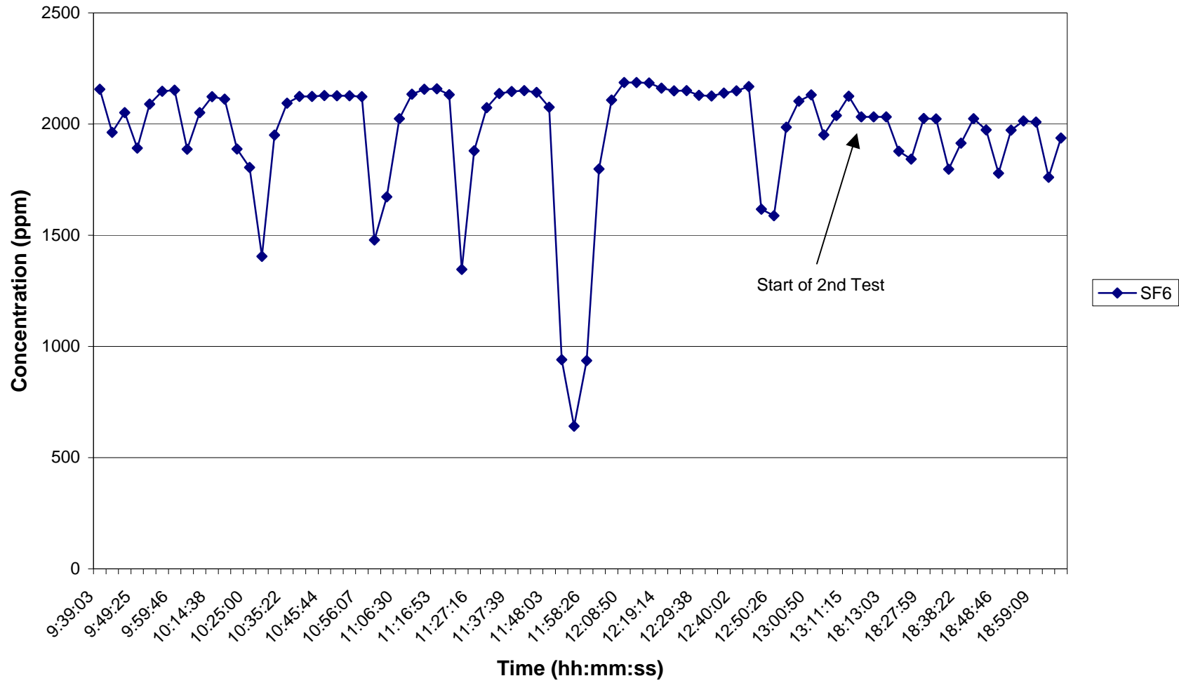
Time Series Plot of SF 6 During SF 6 Injection at 3000ppm on 8/24/06
