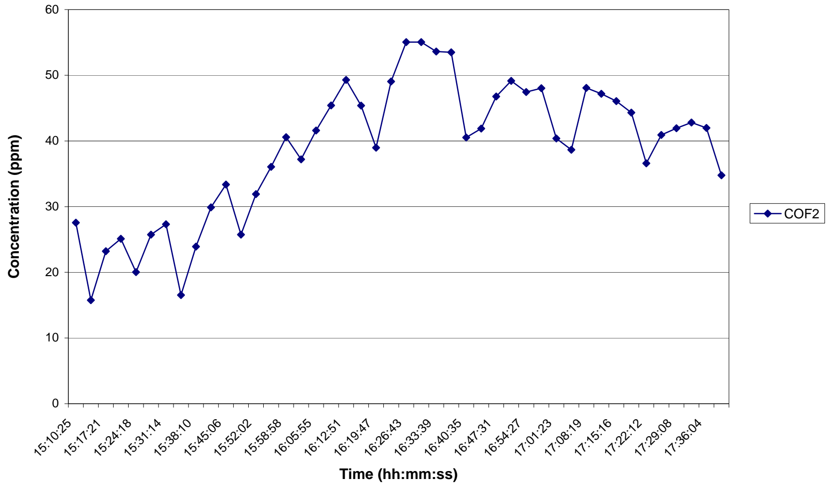
Time Series Plot for COF 2 During HFC-134a Injection at 4200 ppm on 8/24/06
