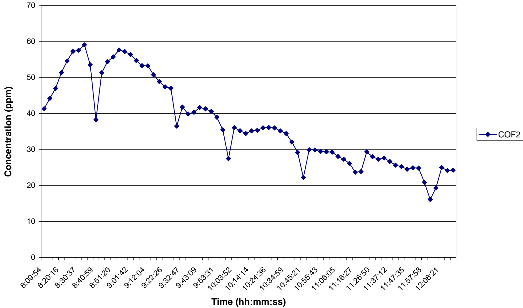
Time Series Plot for COF 2 During HFC-134a Injection at 3600 ppm on 8/25/06
