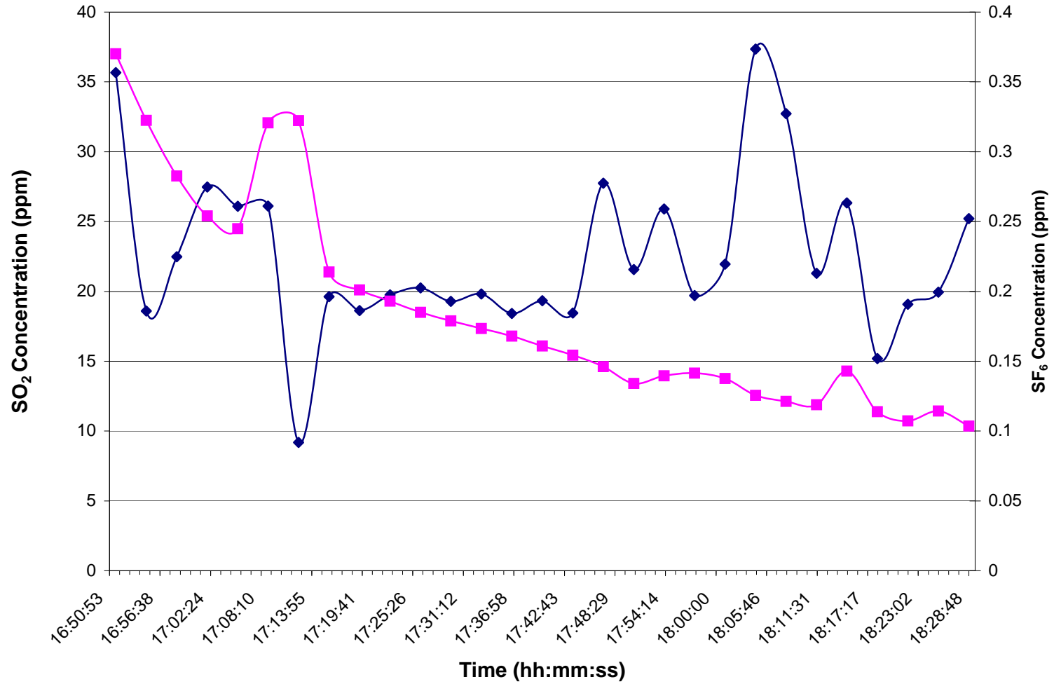
Time Series Plot of SO 2 and SF 6 During CO 2 Injection on 8/29/06
