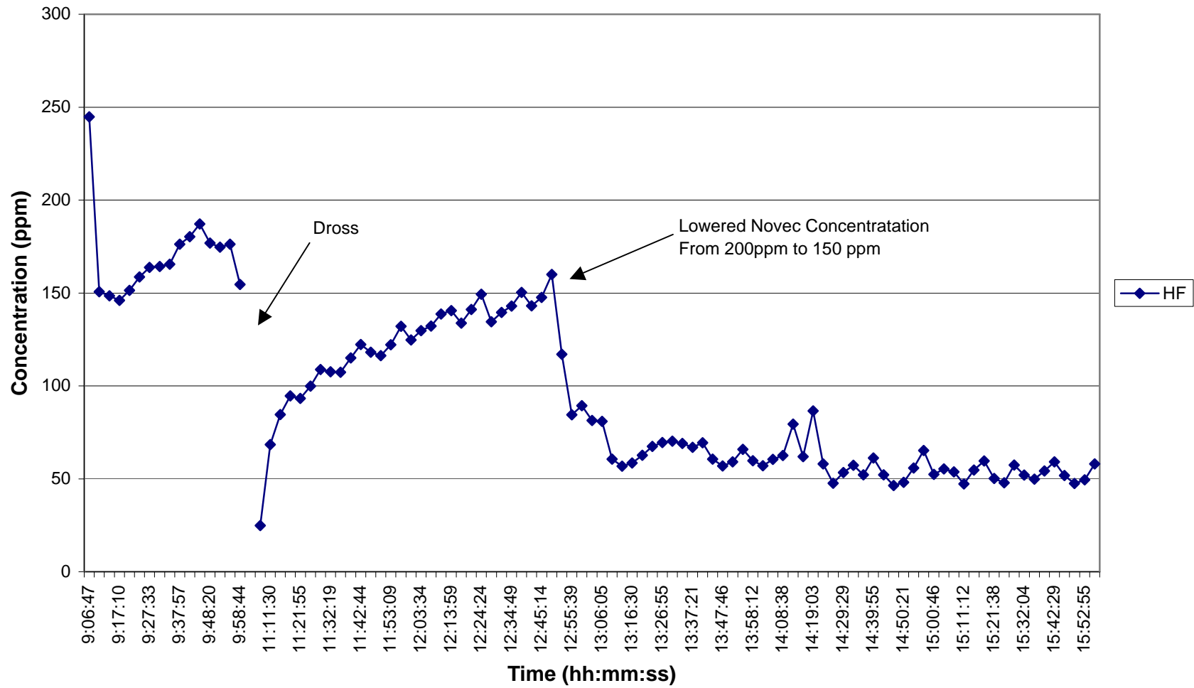
Time Series Plot for HF Using Novec™-612 Cover Gas on 8/23/06
