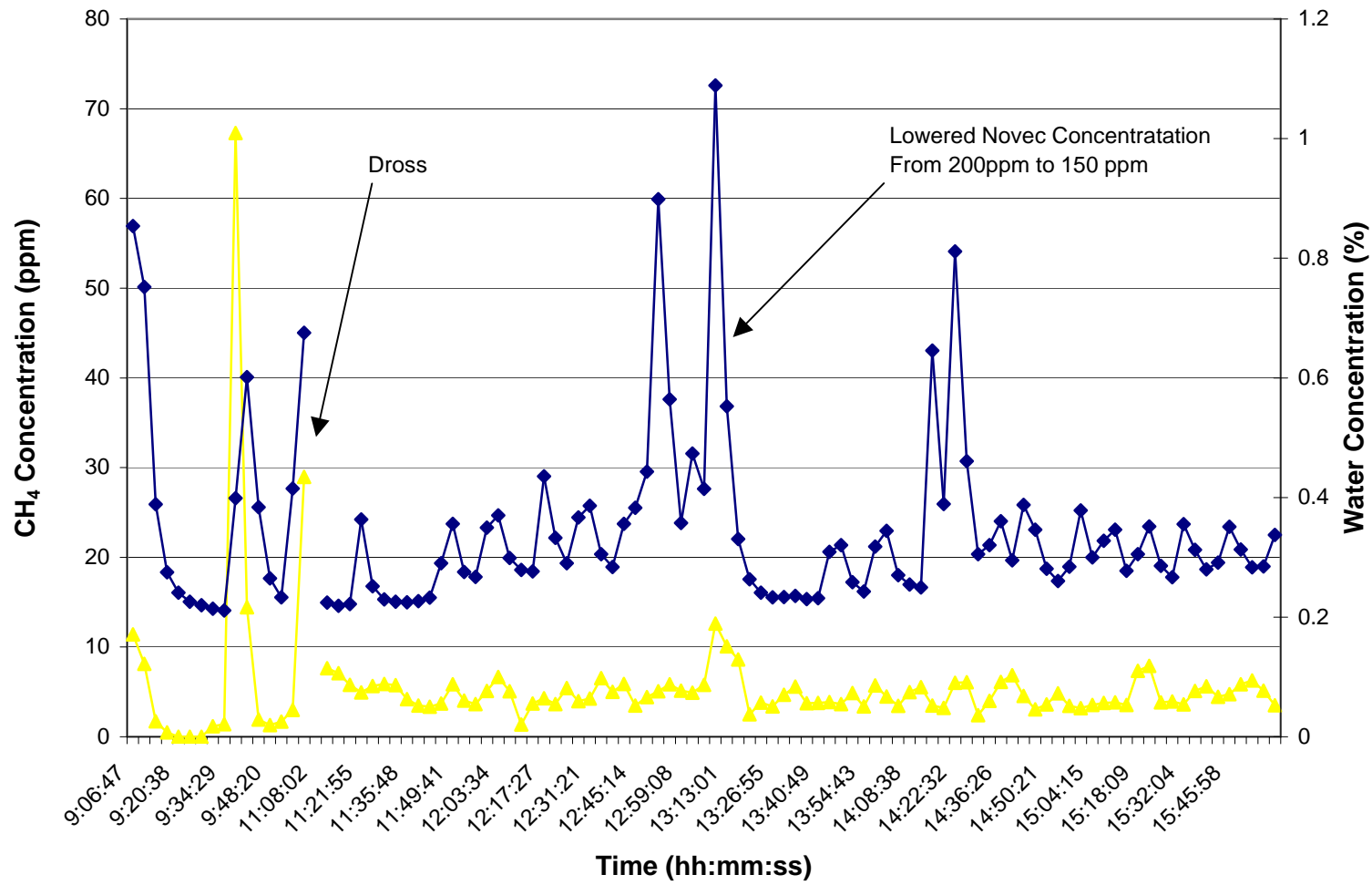
Time Series Plot for CH 4 and H 2 O Using Novec™-612 Cover Gas on 8/23/06
