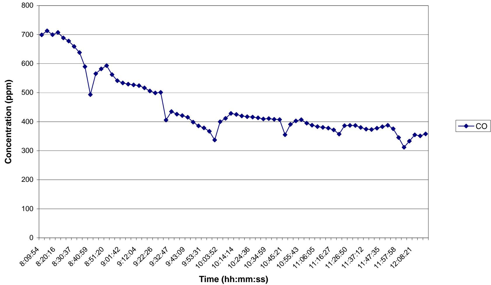
Time Series Plot for CO During HFC-134a Injection at 3600 ppm on 8/25/06
