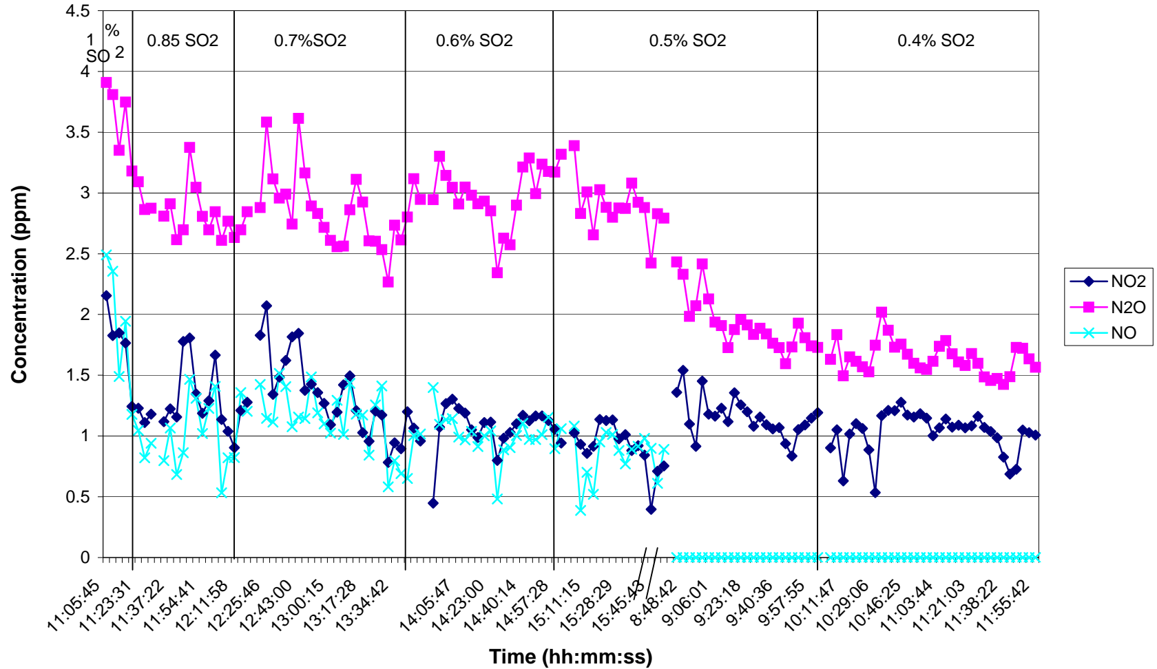
Time Series Plot for Nitrogen Oxides During SO 2 Cover Gas Injections on 8/28-8/29, 2006
