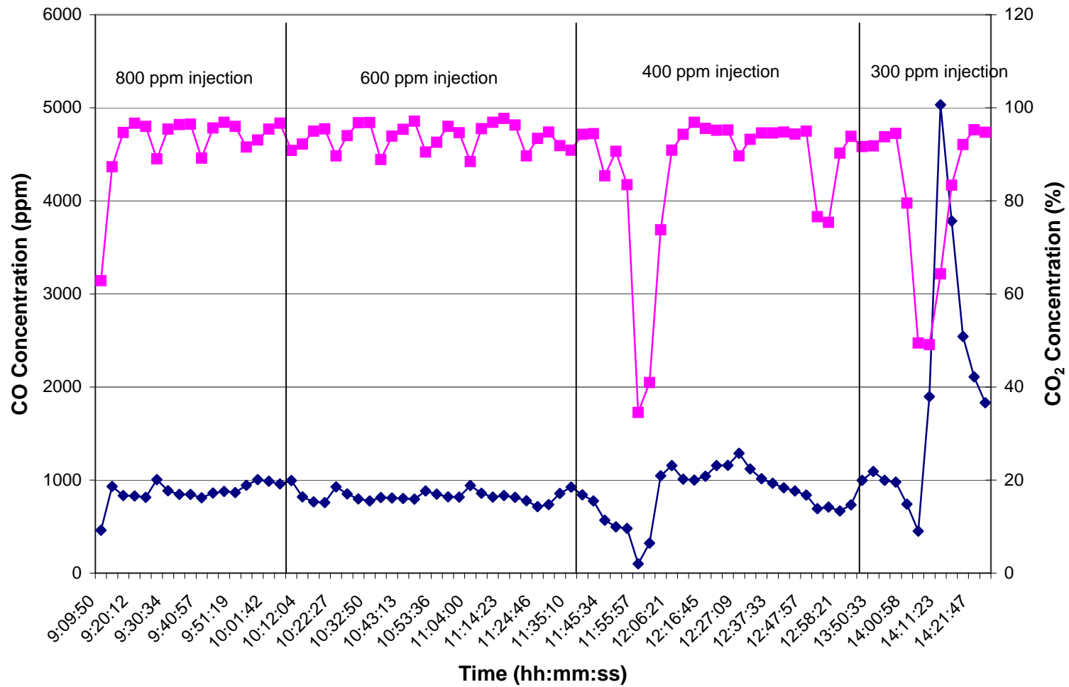
Time Series Plot for CO 2 and CO Using Novec™-612 Cover Gas on 8/22/06
