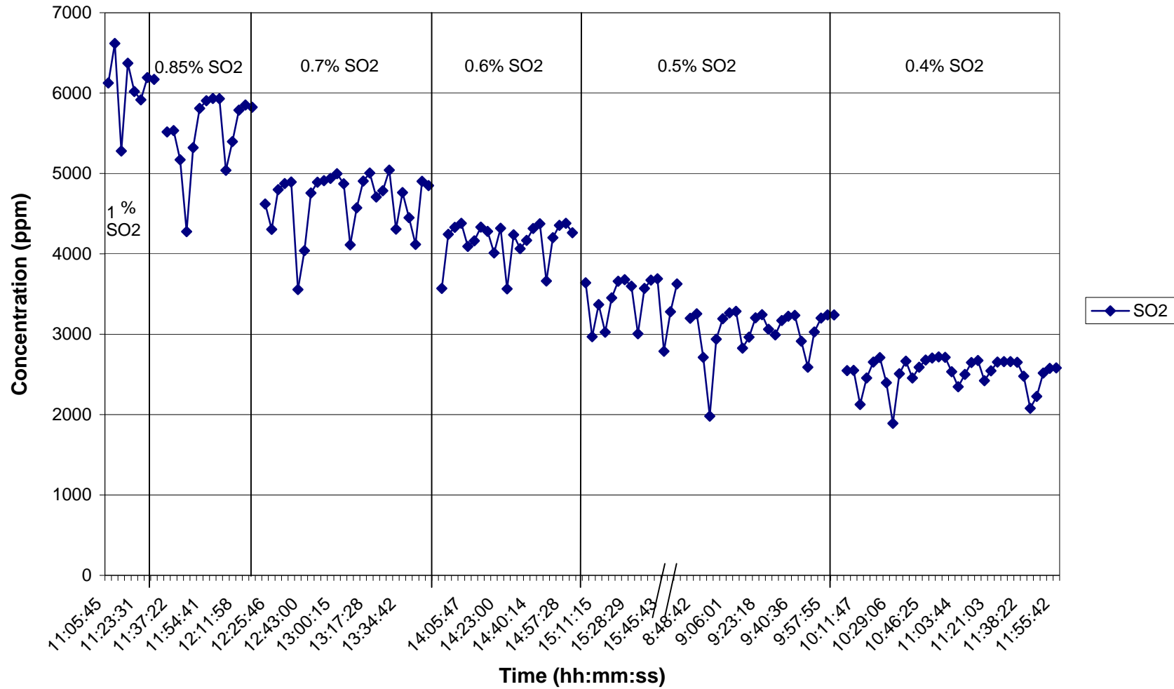
Time Series Plot for SO 2 During SO 2 Cover Gas Injections on 8/28-8/29, 2006
