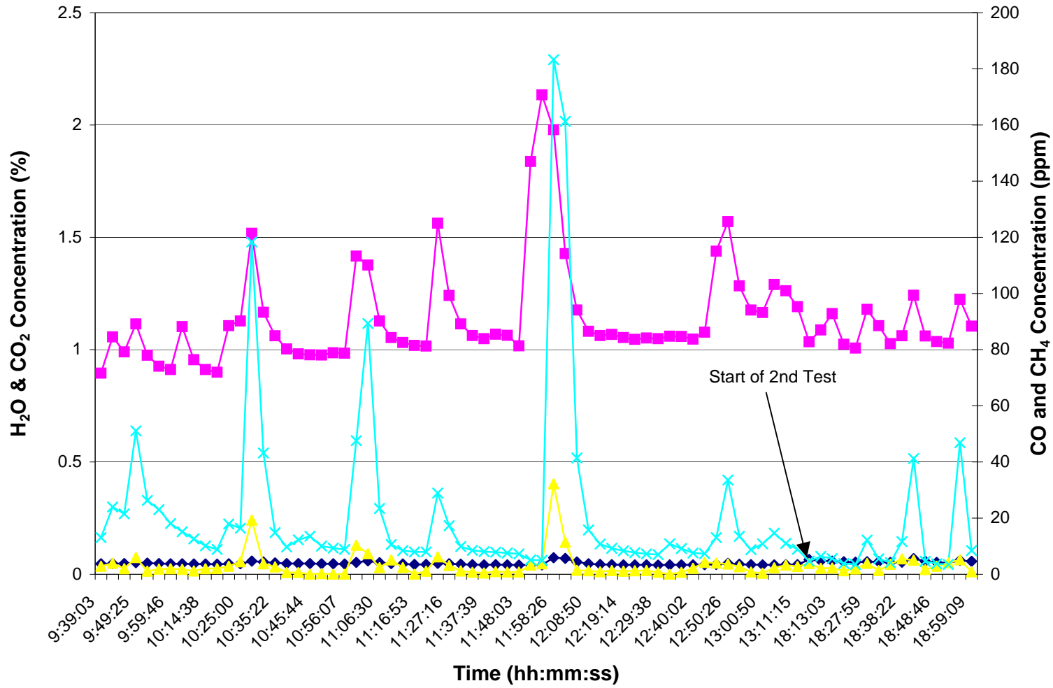
Time Series Plot of Ambient Compounds During SF 6 Injection at 3000ppm on 8/24/06
