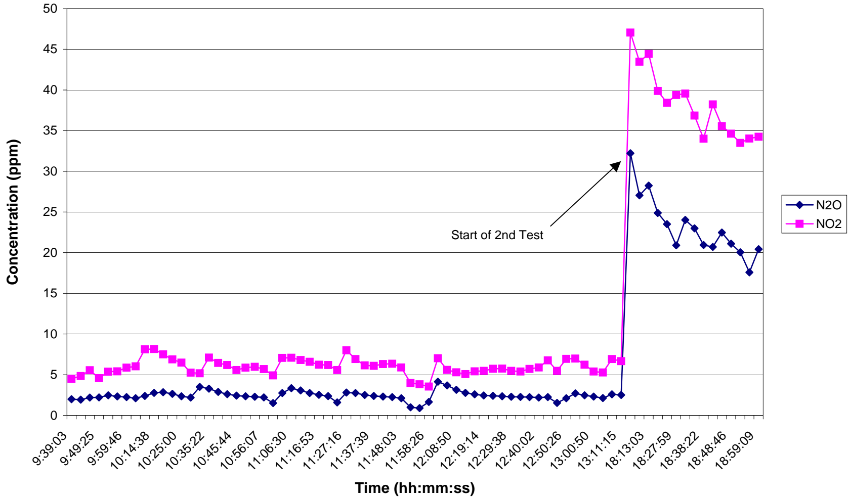
Time Series Plot of N 2 O and NO 2 During SF 6 Injection at 3000ppm on 8/24/06
