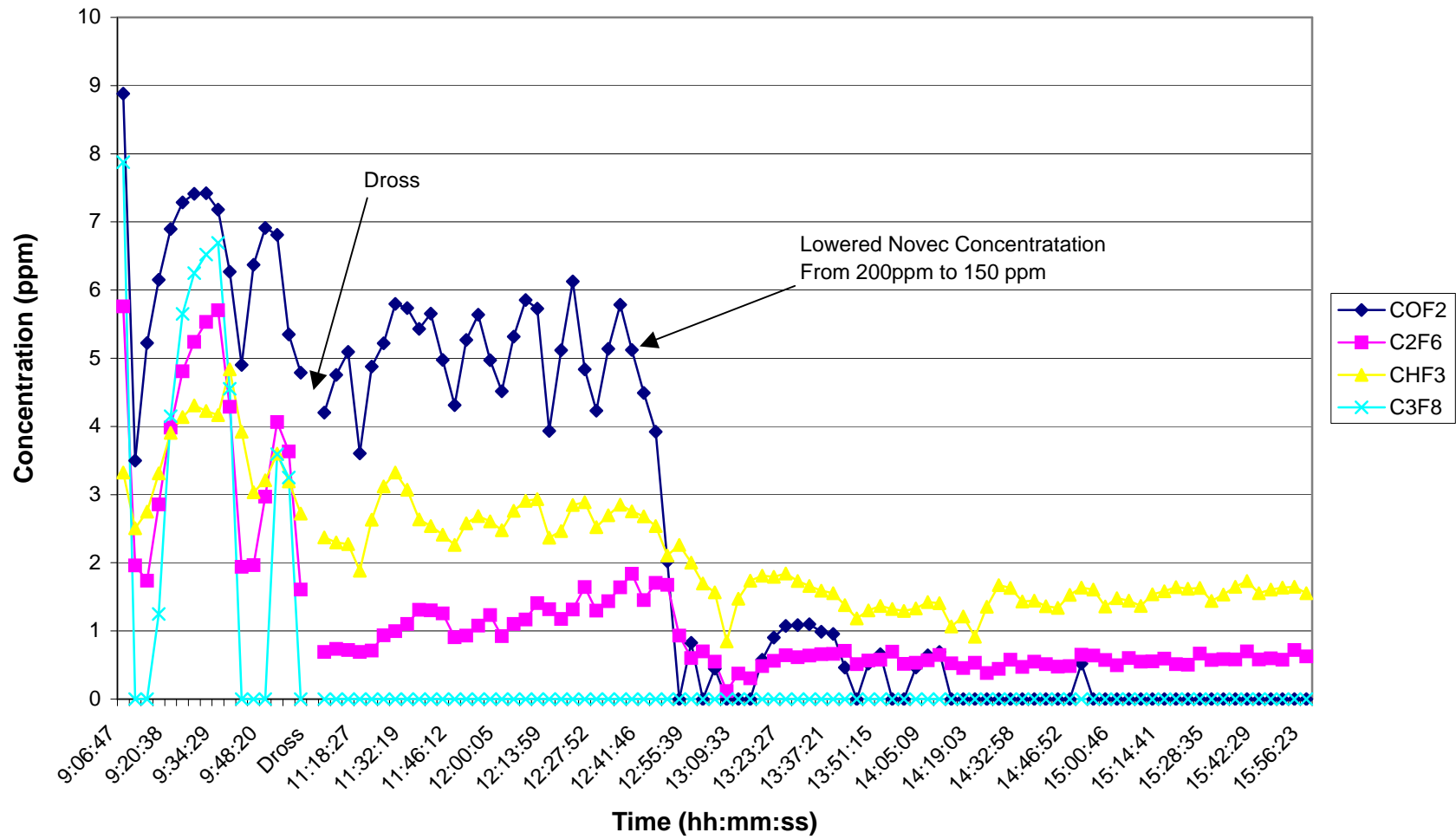
Time Series Plot for PFCs Using Novec™-612 Cover Gas on 8/23/06
