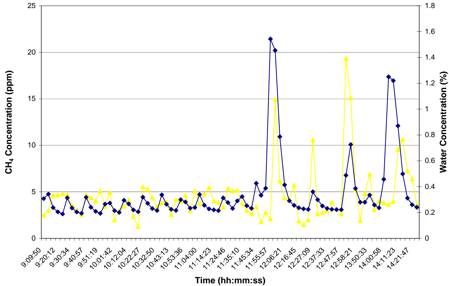
Time Series Plot for CH 4 and H 2 O Using Novec™-612 Cover Gas on 8/22/06
