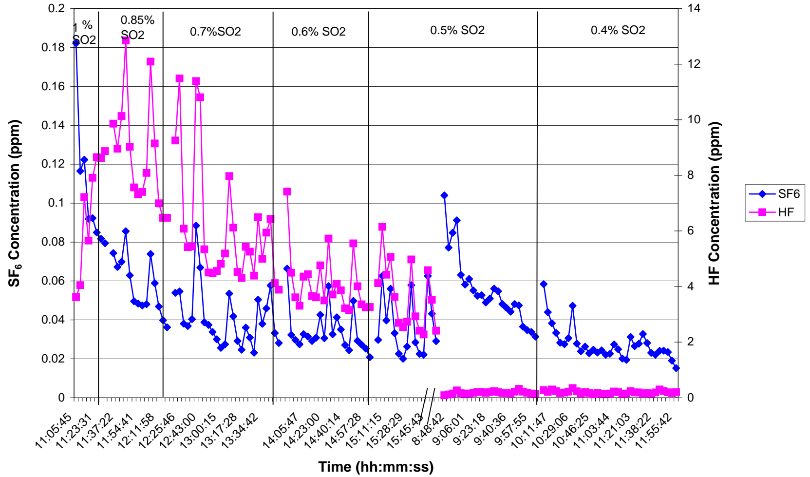
Time Series Plot for SF 6 and HF During SO 2 Cover Gas Injections on 8/28-8/29, 2006
