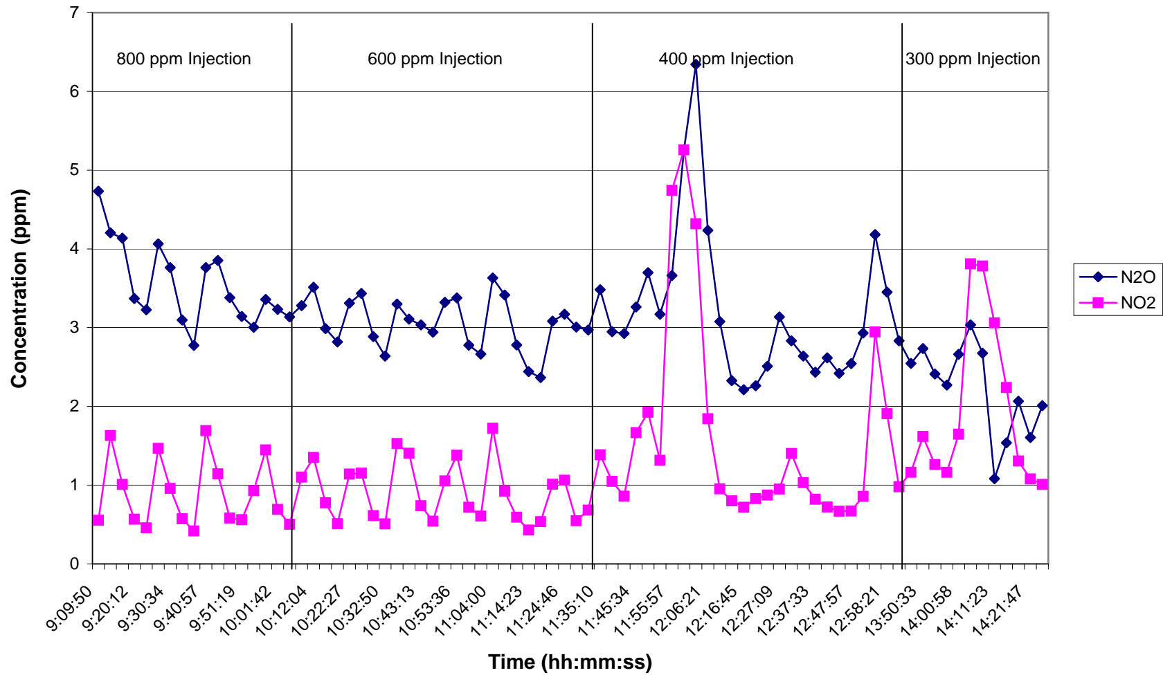
Time Series Plot for Nitrogen Oxides Using Novec™-612 Cover Gas on 8/22/06
