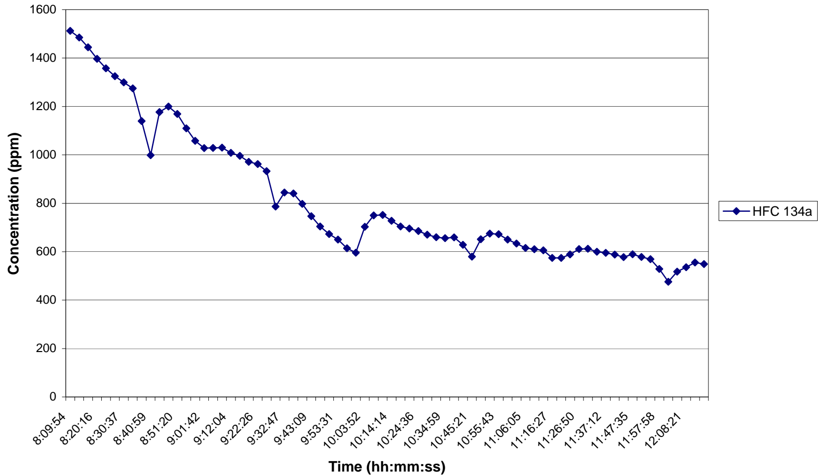
Time Series Plot for HFC-134a During Injection at 3600 ppm on 8/25/06
