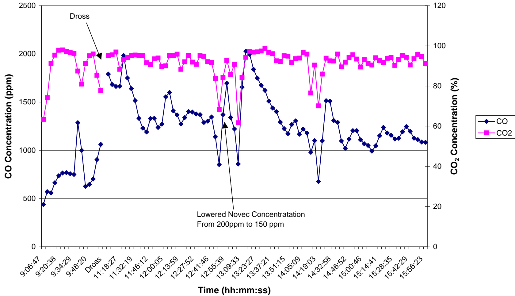
Time Series Plot for CO 2 and CO Using Novec™-612 Cover Gas on 8/23/06
