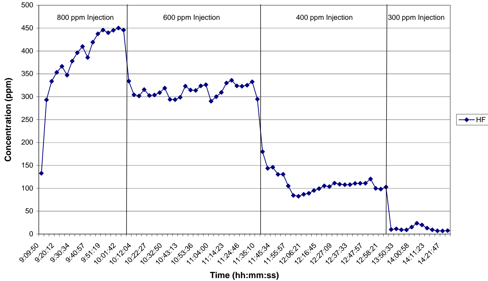
Time Series Plot for HF Using Novec™-612 Cover Gas on 8/22/06
