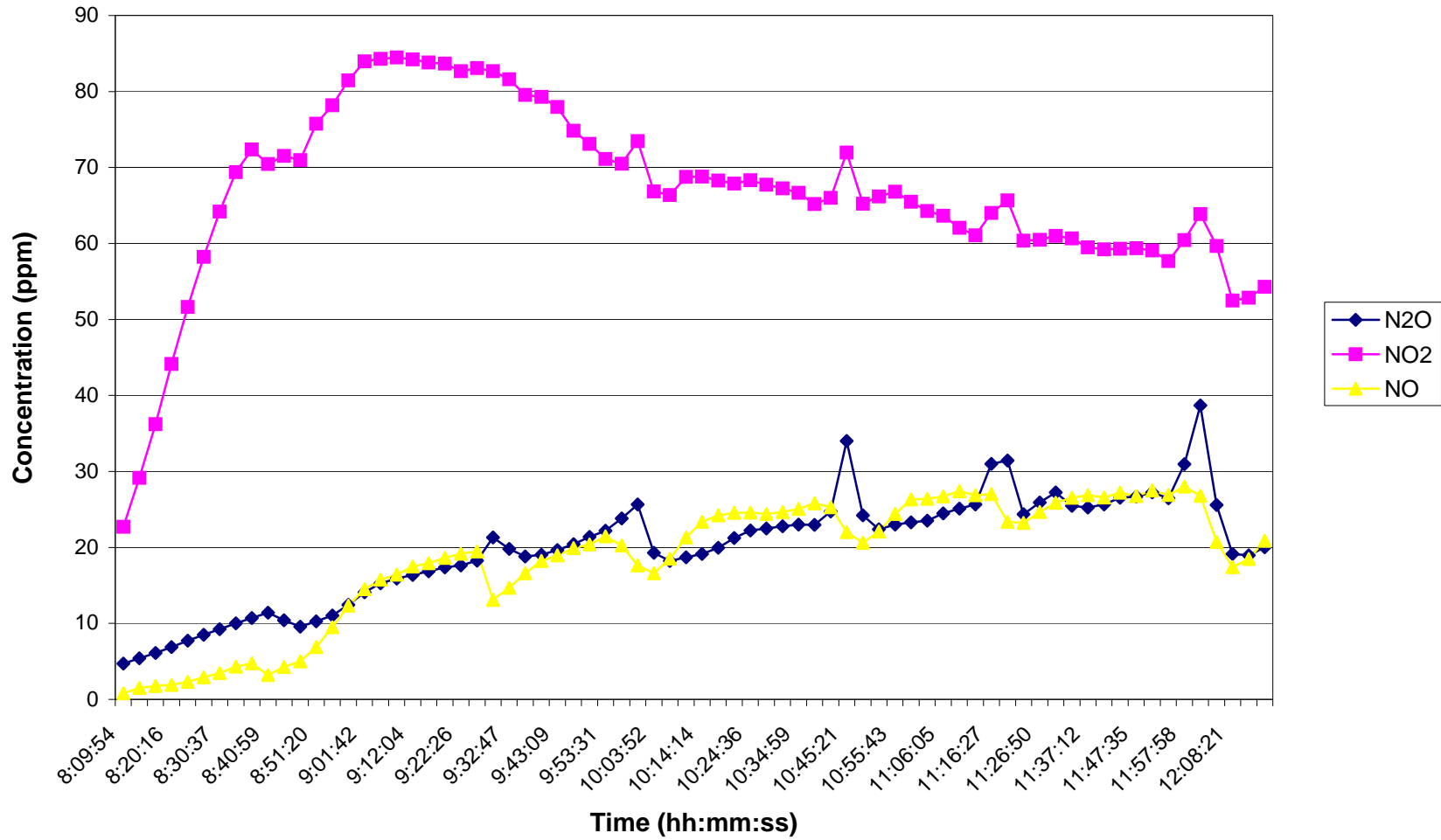
Time Series Plot for Nitrogen Oxide By-Products During HFC-134a Injection at 3600 ppm on 8/25/06
