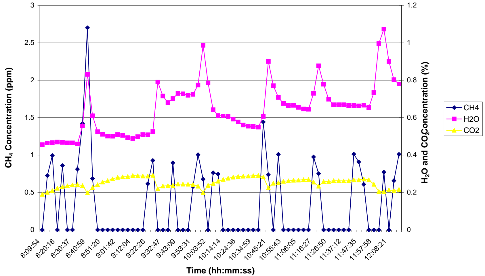
Time Series Plot for Ambient Air Compounds During HFC-134a Injection at 3600 ppm on 8/25/06
