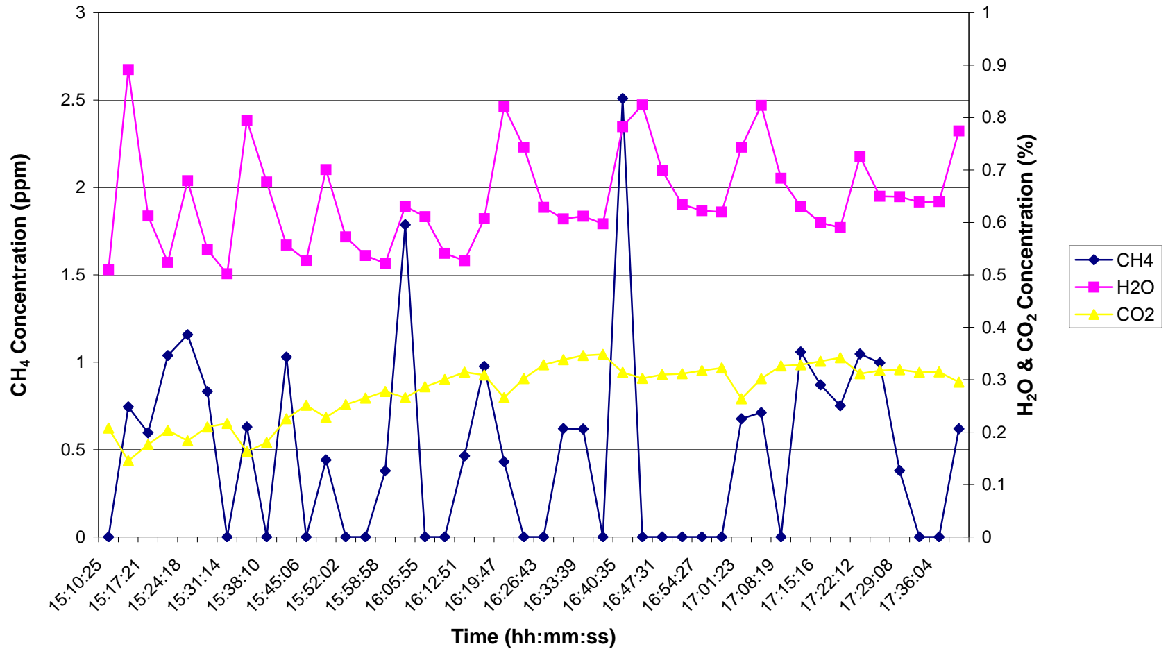
Time Series Plot for Ambient Air Compounds During HFC-134a Injection at 4200 ppm on 8/24/06
