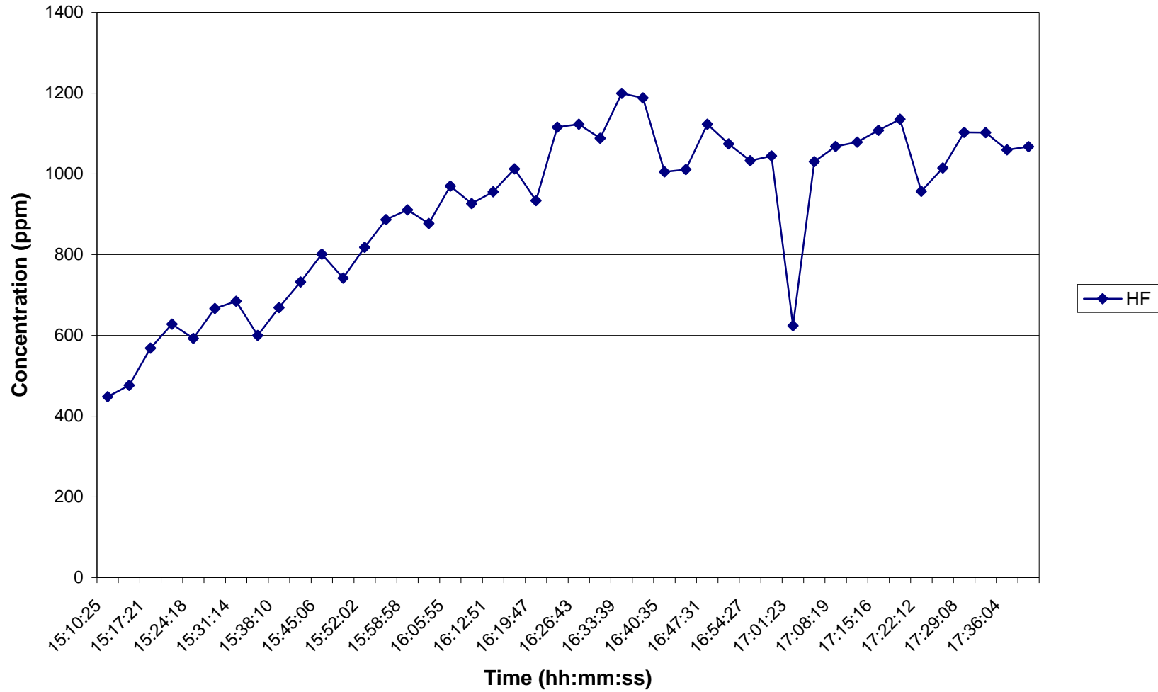
Time Series Plot for HF During HFC-134a Injection at 4200 ppm on 8/24/06
