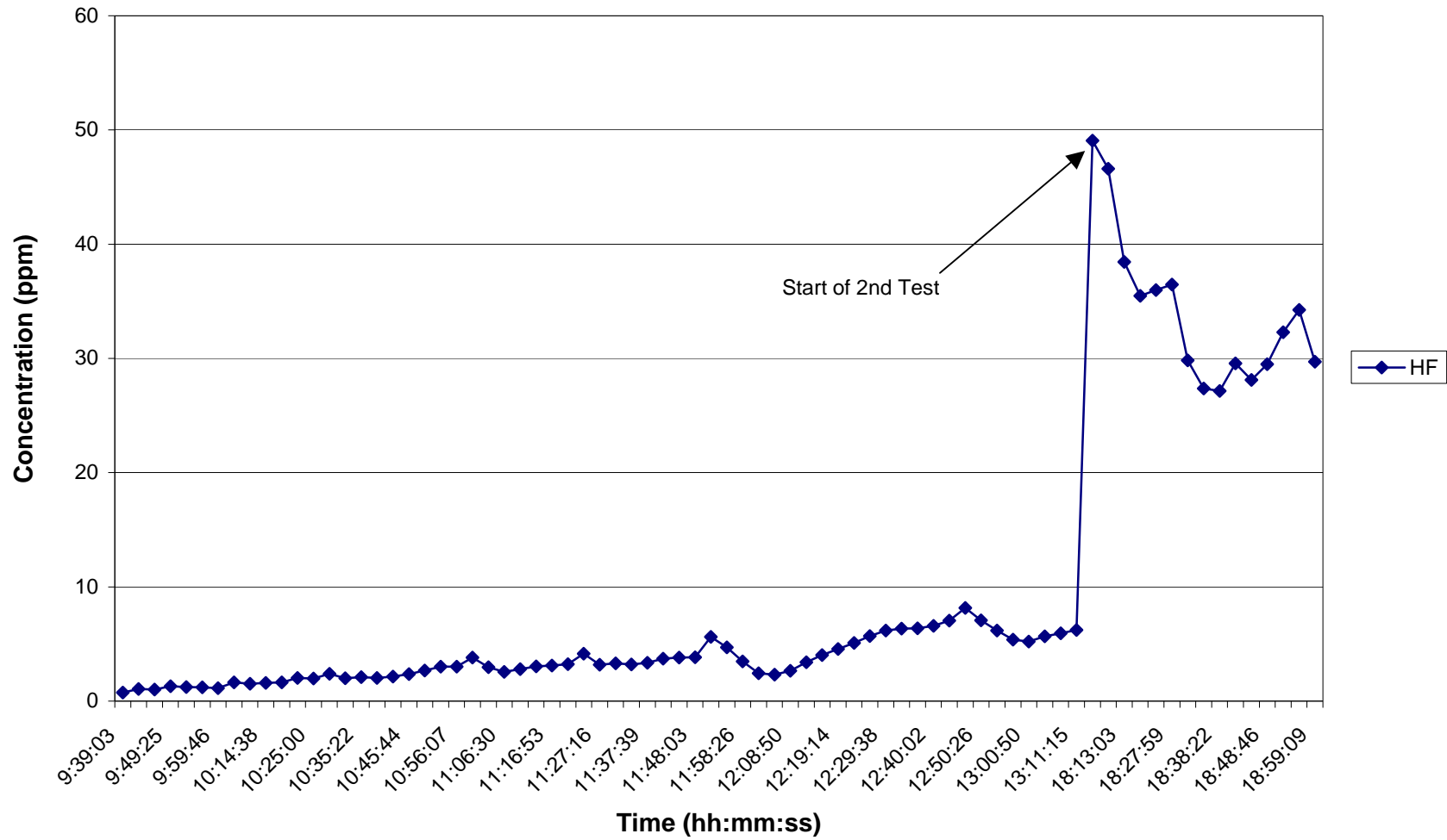
Time Series Plot of HF During SF 6 Injection at 3000ppm on 8/24/06
