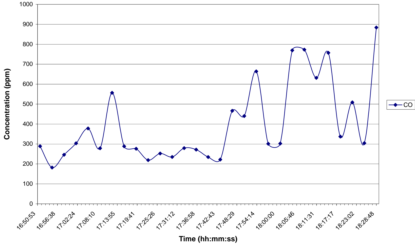
Time Series Plot of CO During CO 2 Injection on 8/29/06
