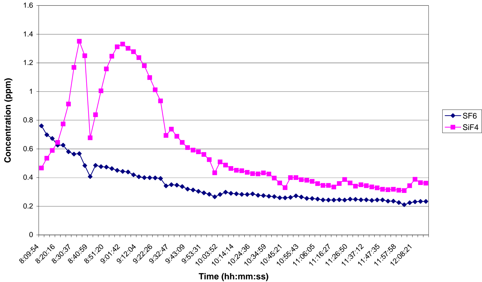
Time Series Plot for Non-Process By-Products During HFC-134a Injection at 3600 ppm on 8/25/06
