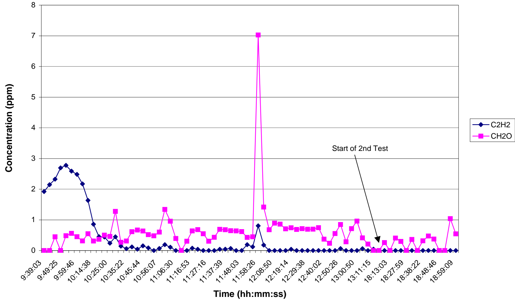
Time Series Plot of C 2 H 2 and CH 2 O During SF 6 Injection at 3000ppm on 8/24/06
