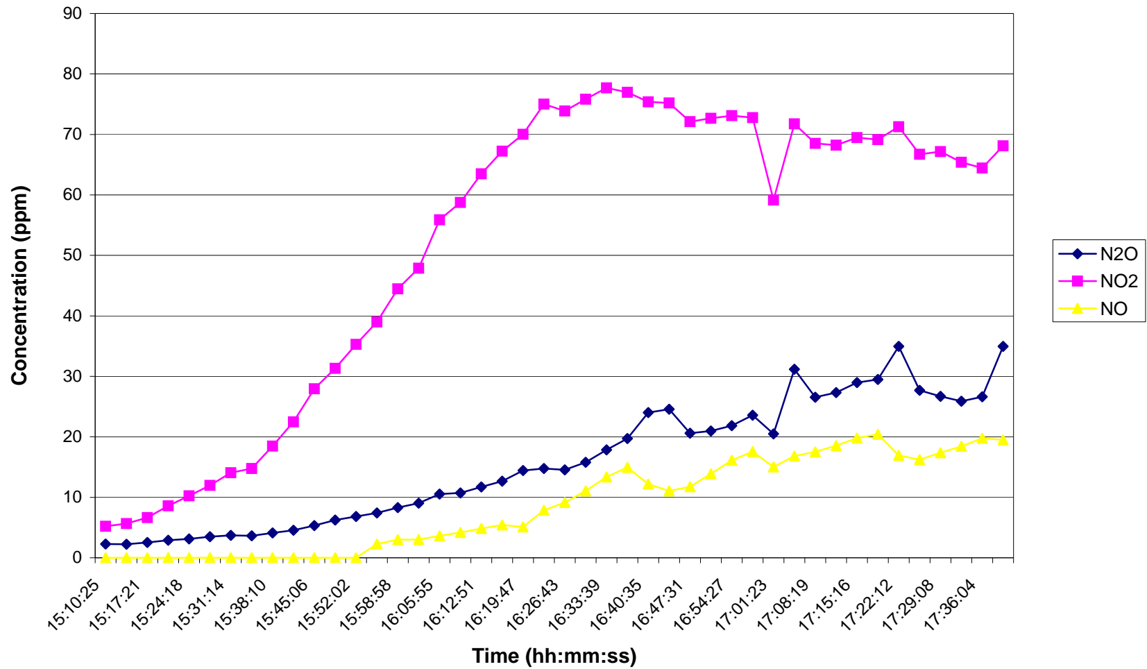
Time Series Plot for Nitrogen Oxide By-Products During HFC-134a Injection at 4200 ppm on 8/24/06
