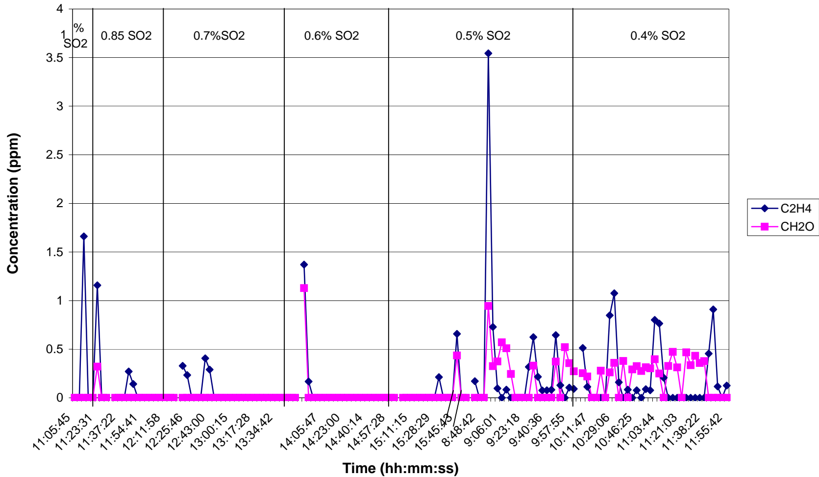
Time Series Plot for C 2 H 4 and CH 2 O During SO 2 Cover Gas Injections on 8/28-8/29, 2006
