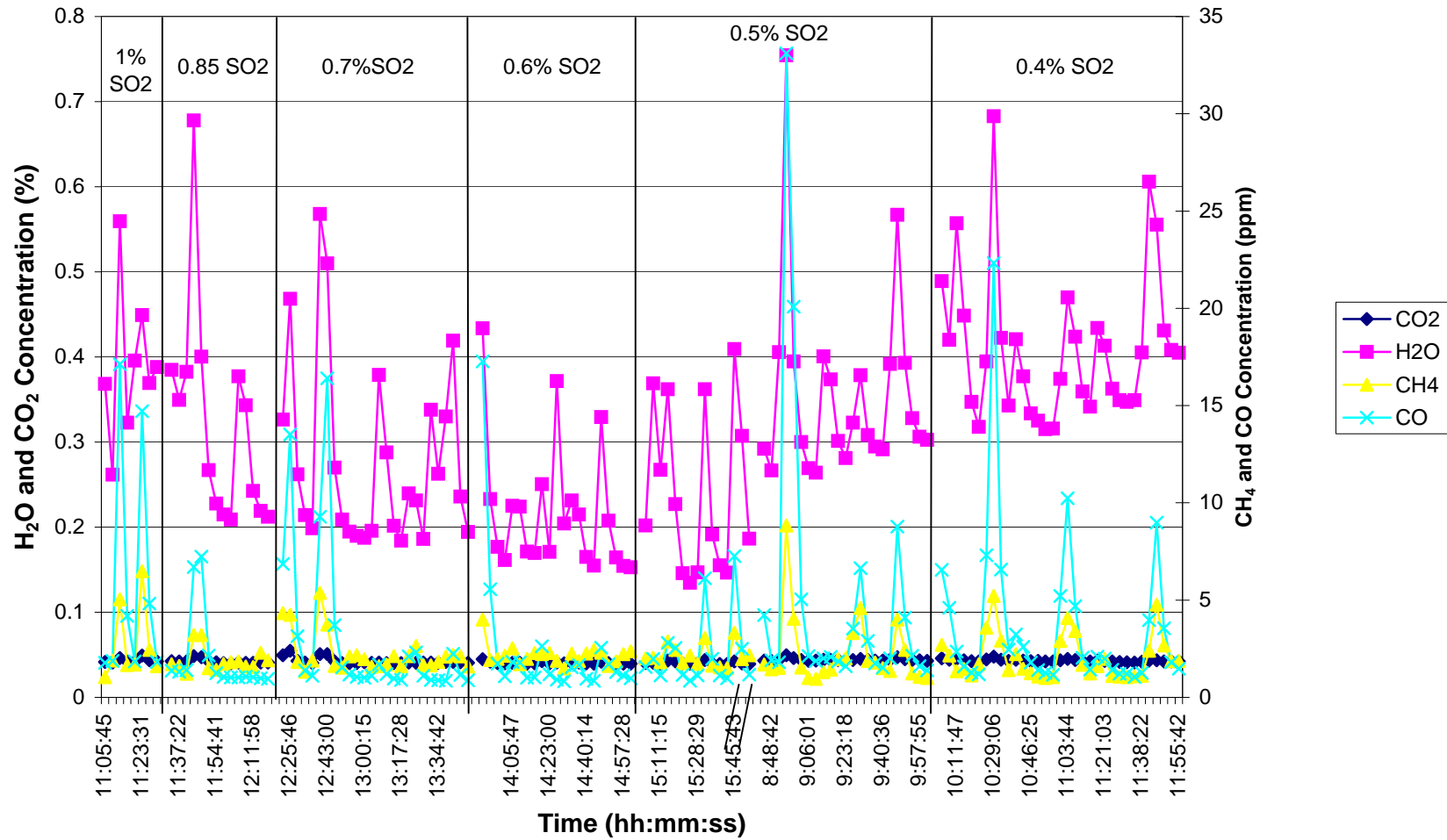
Time Series Plot for Ambient Compounds During SO 2 Cover Gas Injections on 8/28-8/29, 2006
