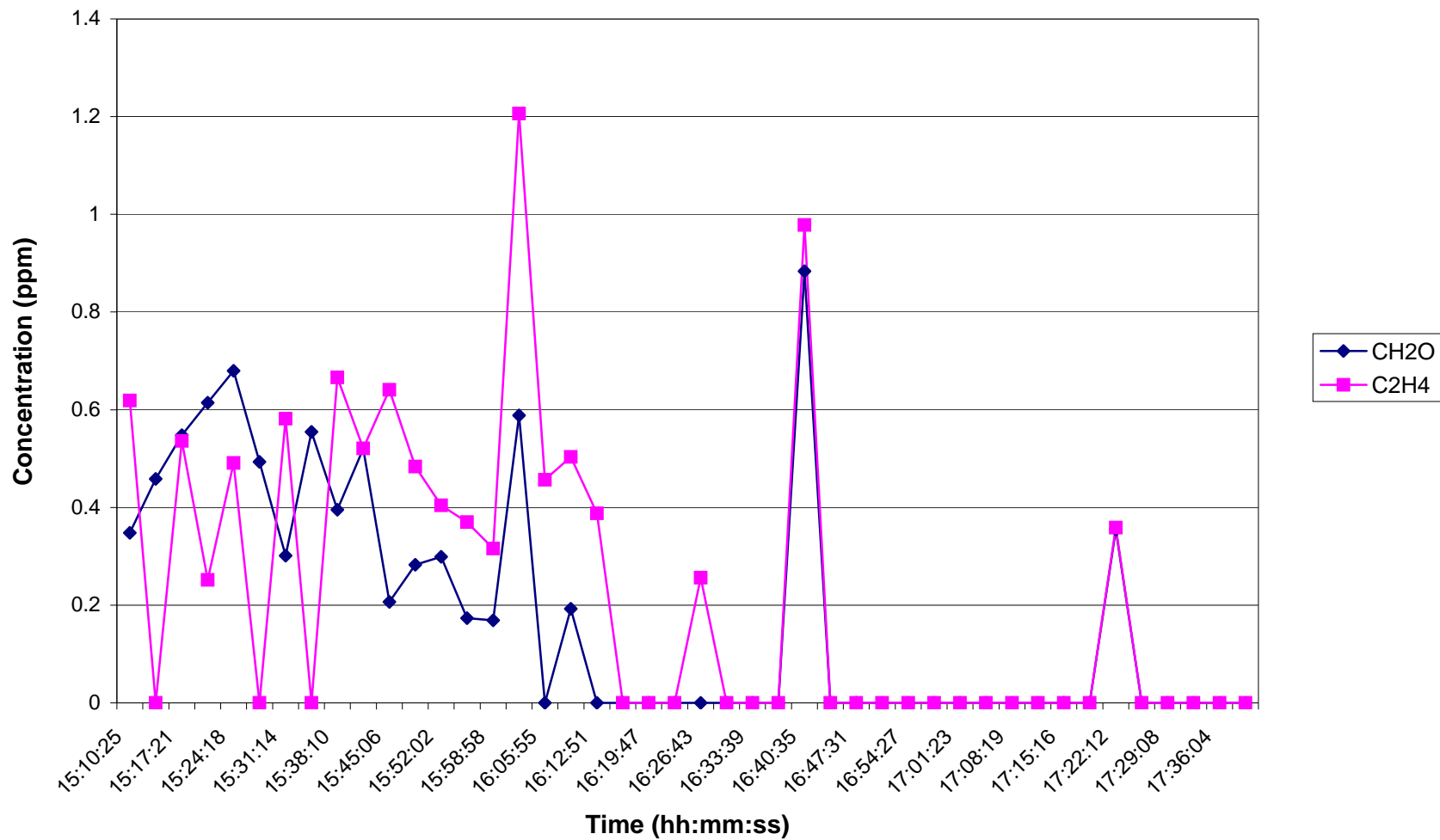
Time Series Plot for CH 2 O and C 2 H 4 During HFC-134a Injection at 4200 ppm on 8/24/06
