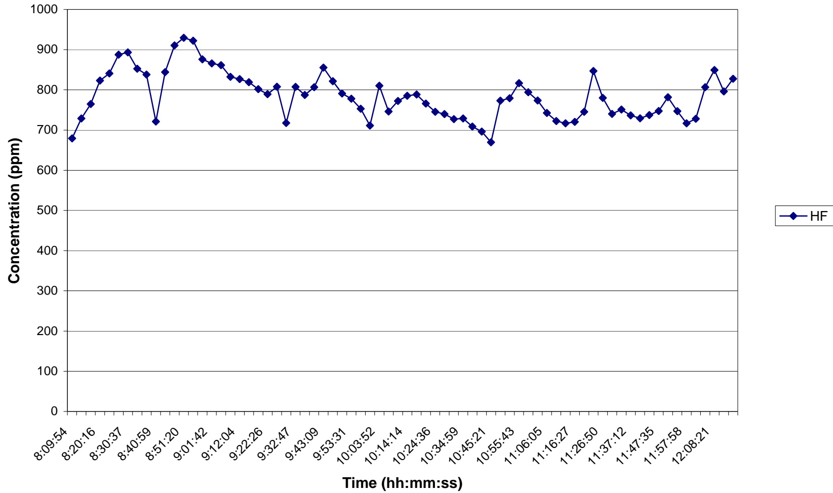
Time Series Plot for HF During HFC-134a Injection at 3600 ppm on 8/25/06
