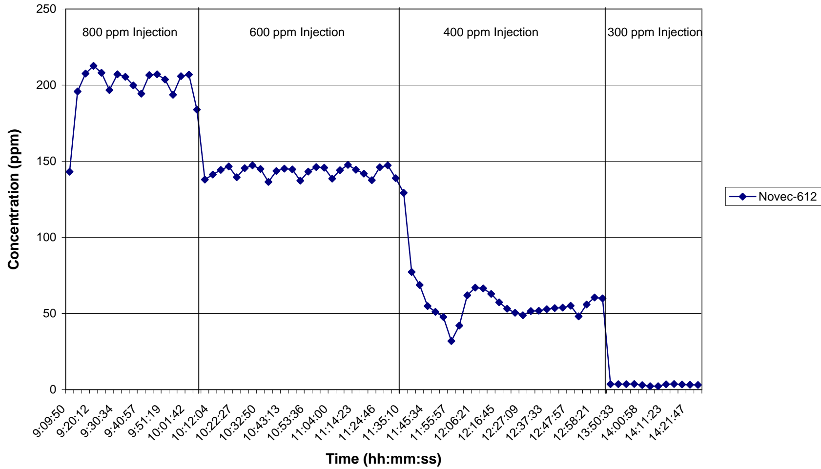
Time Series Plot for Novec™-612 on 8/22/06
