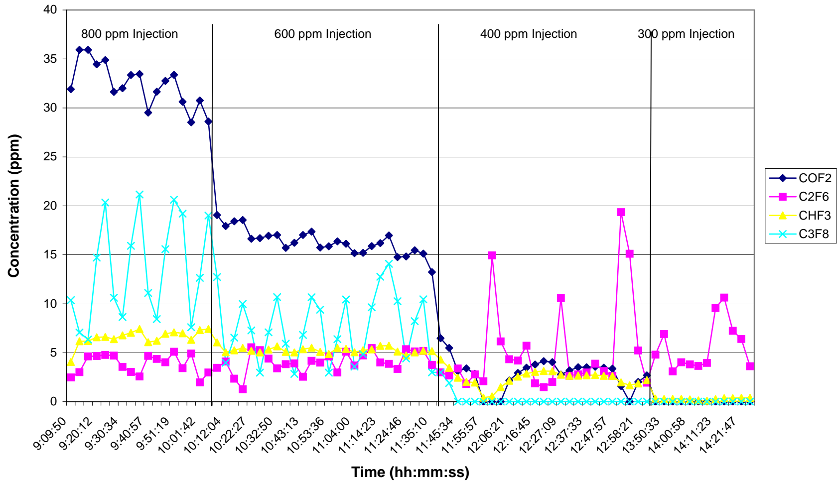
Time Series Plot for PFCs Using Novec™-612 Cover Gas on 8/22/06
