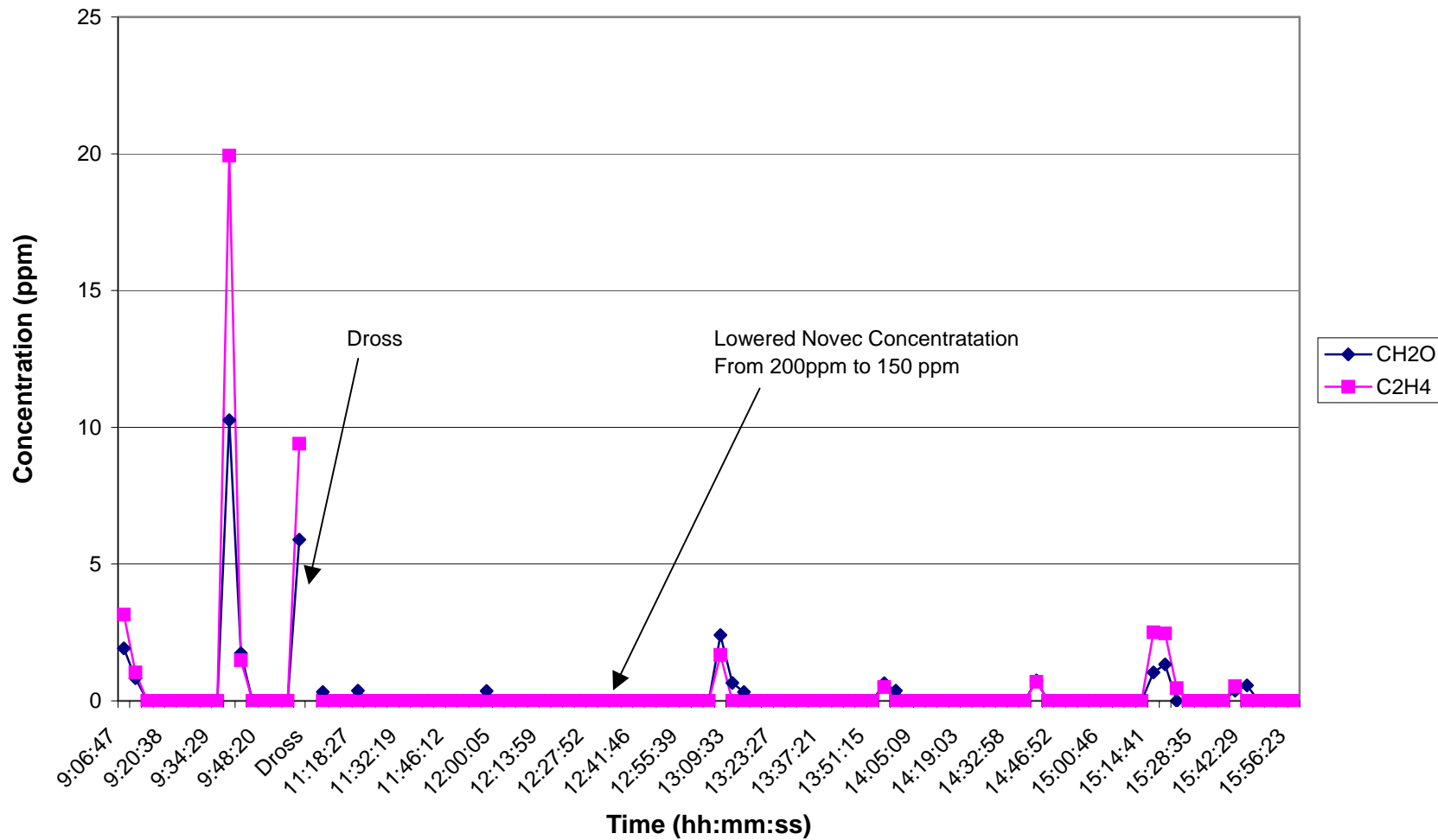
Time Series Plot for CH 2 O and C 2 H 4 on Using Novec™-612 Cover Gas 8/23/06
