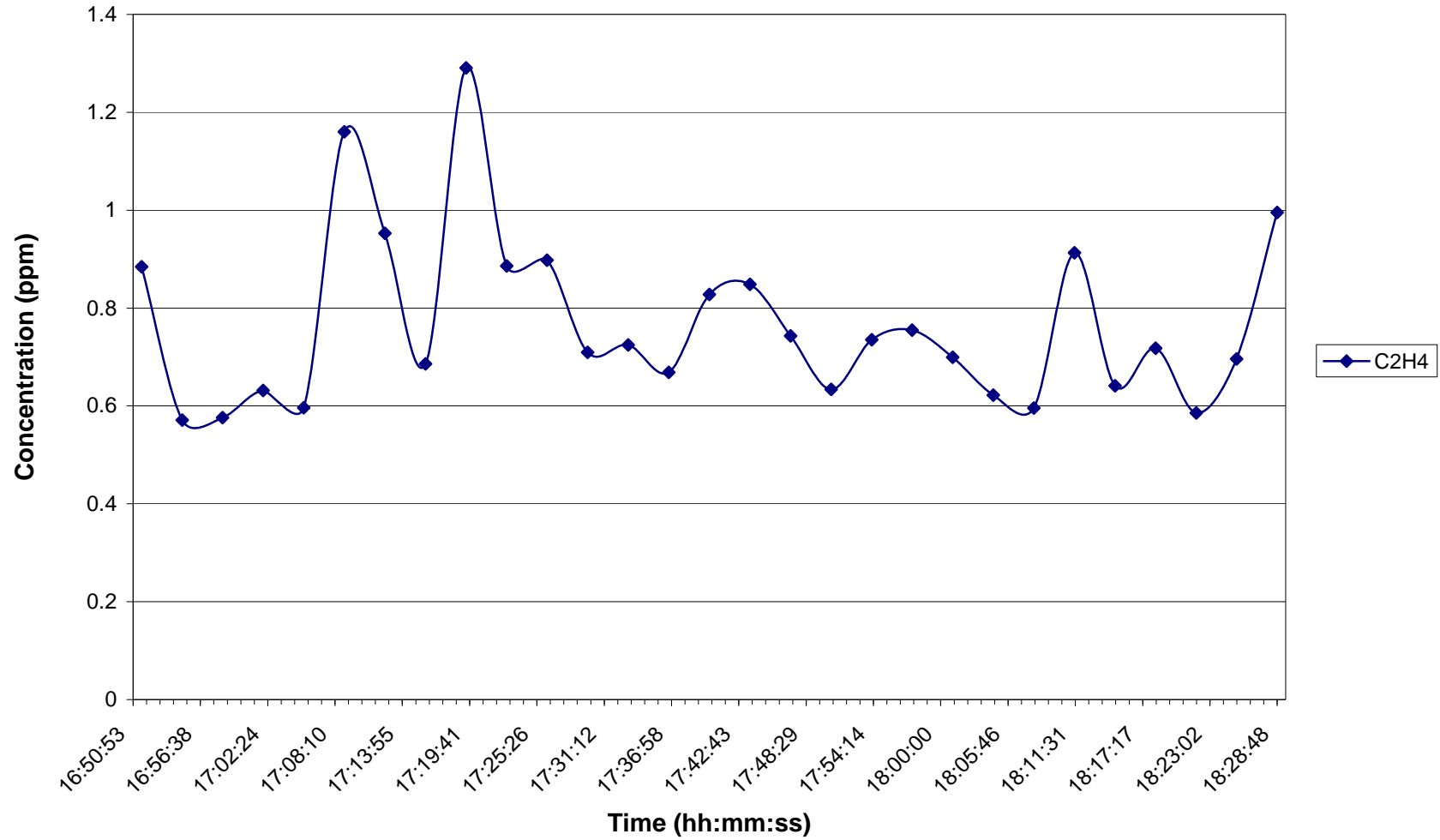
Time Series Plot of C 2 H 4 During CO 2 Injection on 8/29/06
