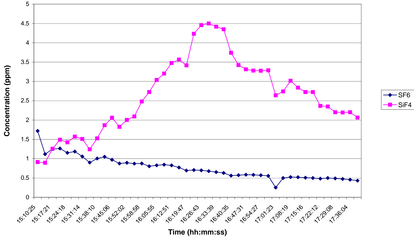
Time Series Plot for Non-Process By-Products During HFC-134a Injection at 4200 ppm on 8/24/06
