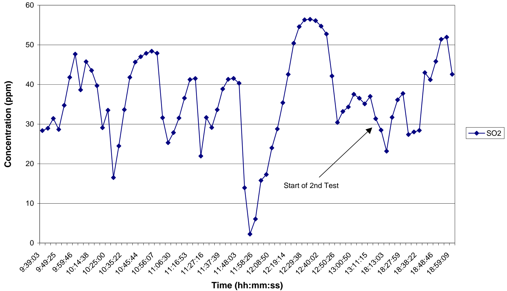
Time Series Plot of SO 2 During SF 6 Injection at 3000ppm on 8/24/06
