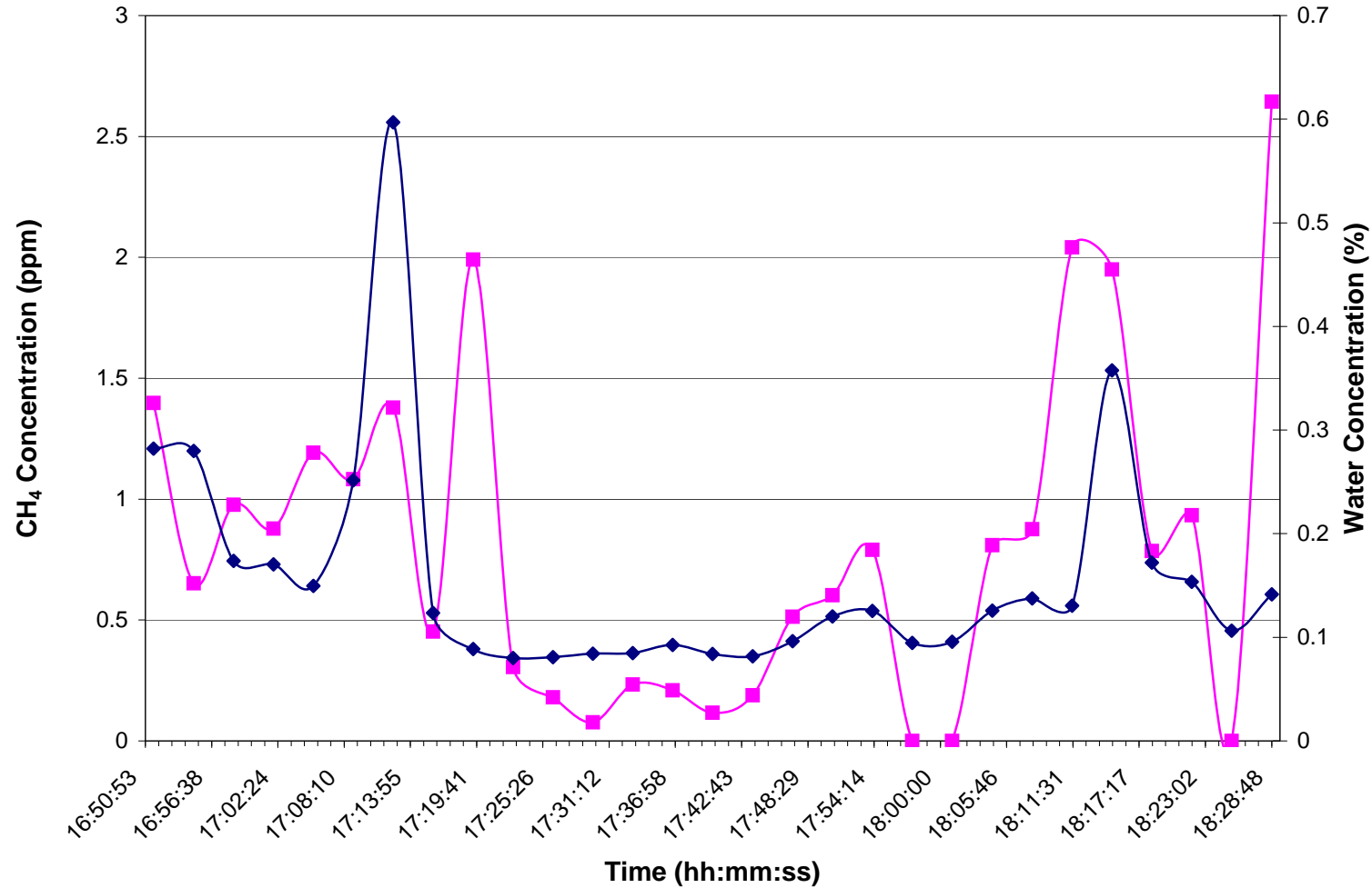
Time Series Plot of CH 4 and H 2 O During CO 2 Injection on 8/29/06
