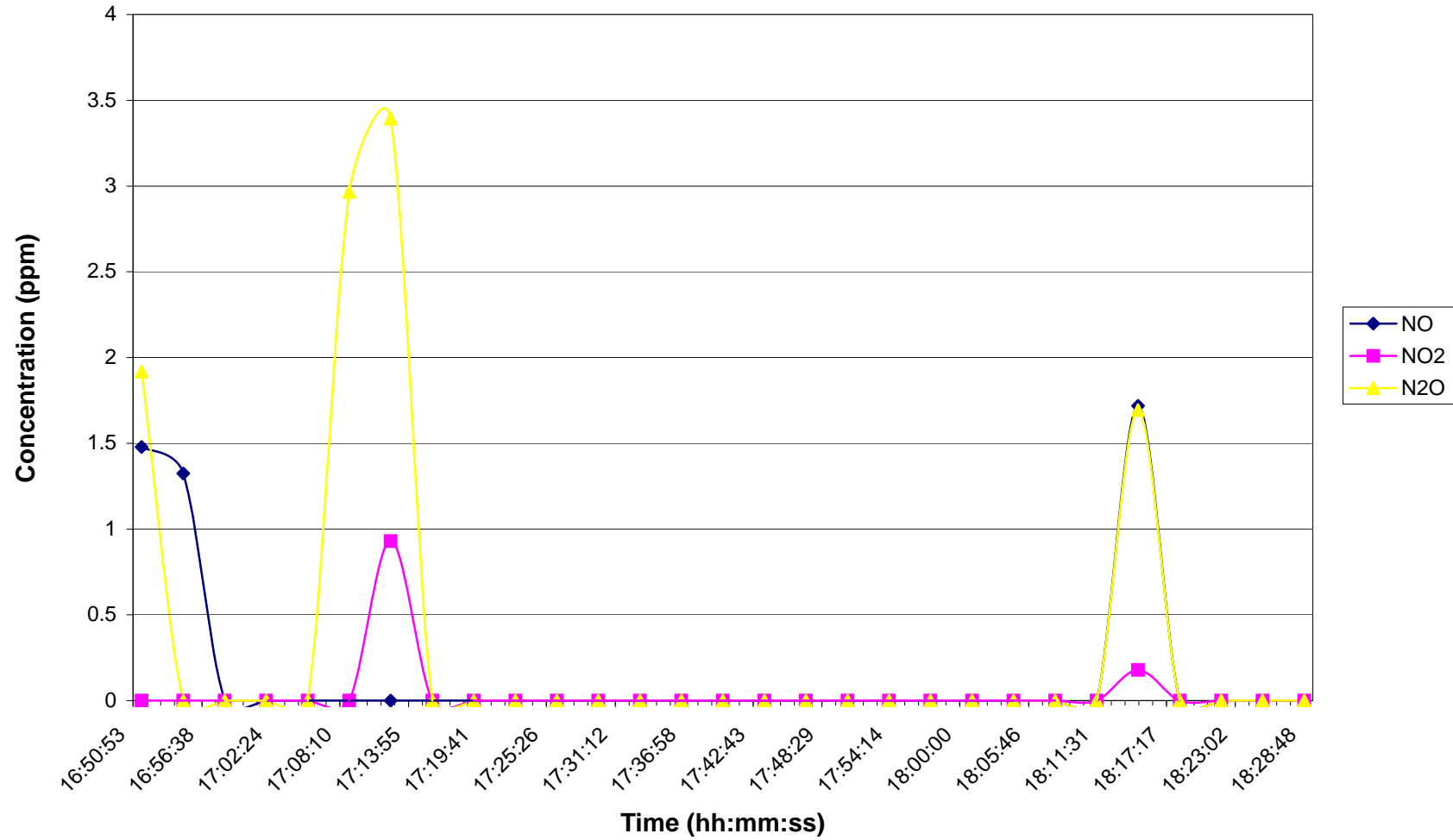
Time Series Plot of Nitrogen Oxides During CO 2 Injection on 8/29/06
