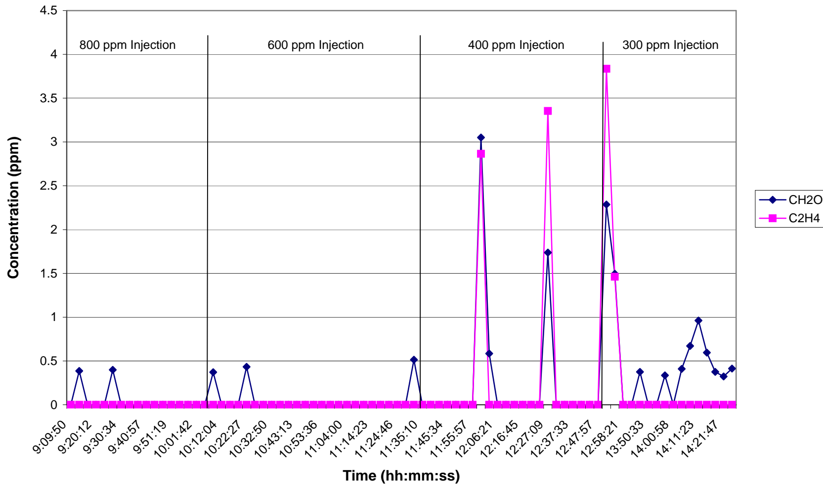
Time Series Plot for CH 2 O and C 2 H 4 Using Novec™-612 Cover Gas on 8/22/06
