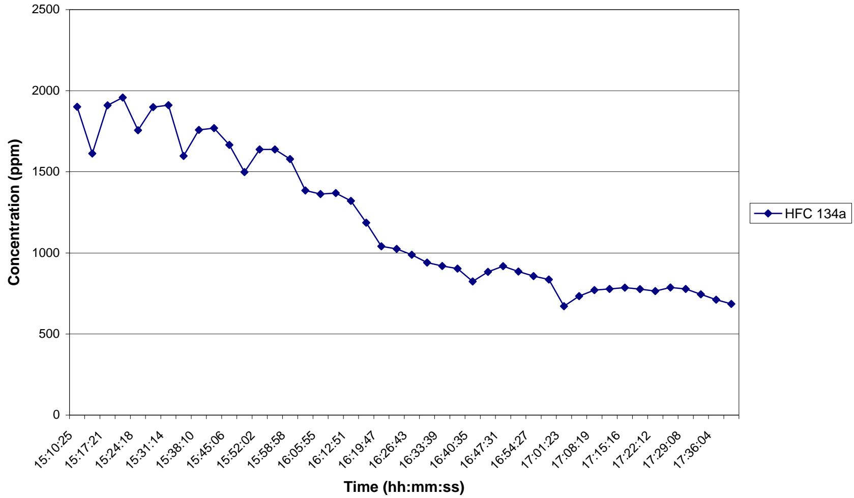
Time Series Plot for HFC-134a During Injection at 4200 ppm on 8/24/06
