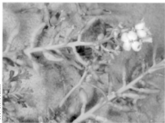
Sea rocket ( Cakile maritima ). This European beach plant spread up and down the west coast of North America at an average rate of 33 miles per year! Its seed capsules are resistant to salt water.
