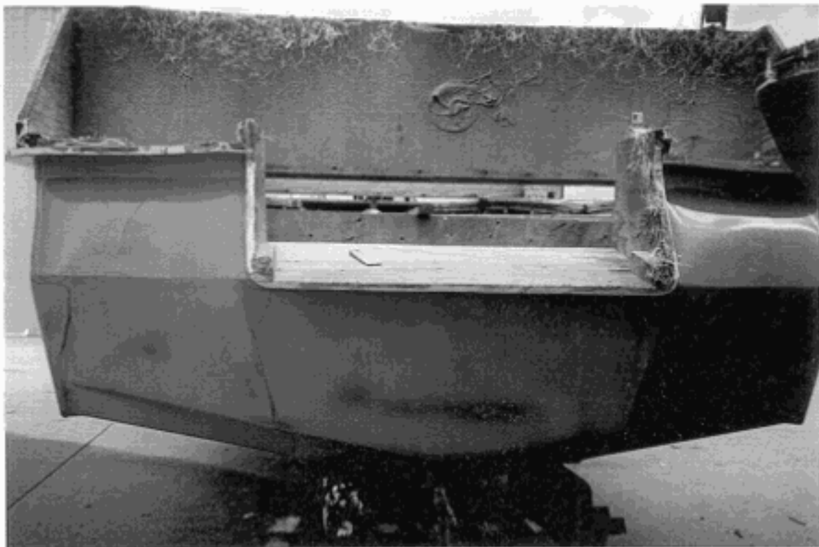
POLAR P3 1700 DV PLUG/MASTER TRANSOM VIEW EXTENDED TRANSOM
