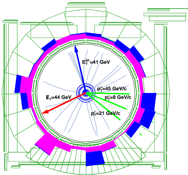
FIG. 9: The trimuon event in the transverse view of the central CDF detector. Tracks with transverse momenta above 1 GeV/c are shown.
