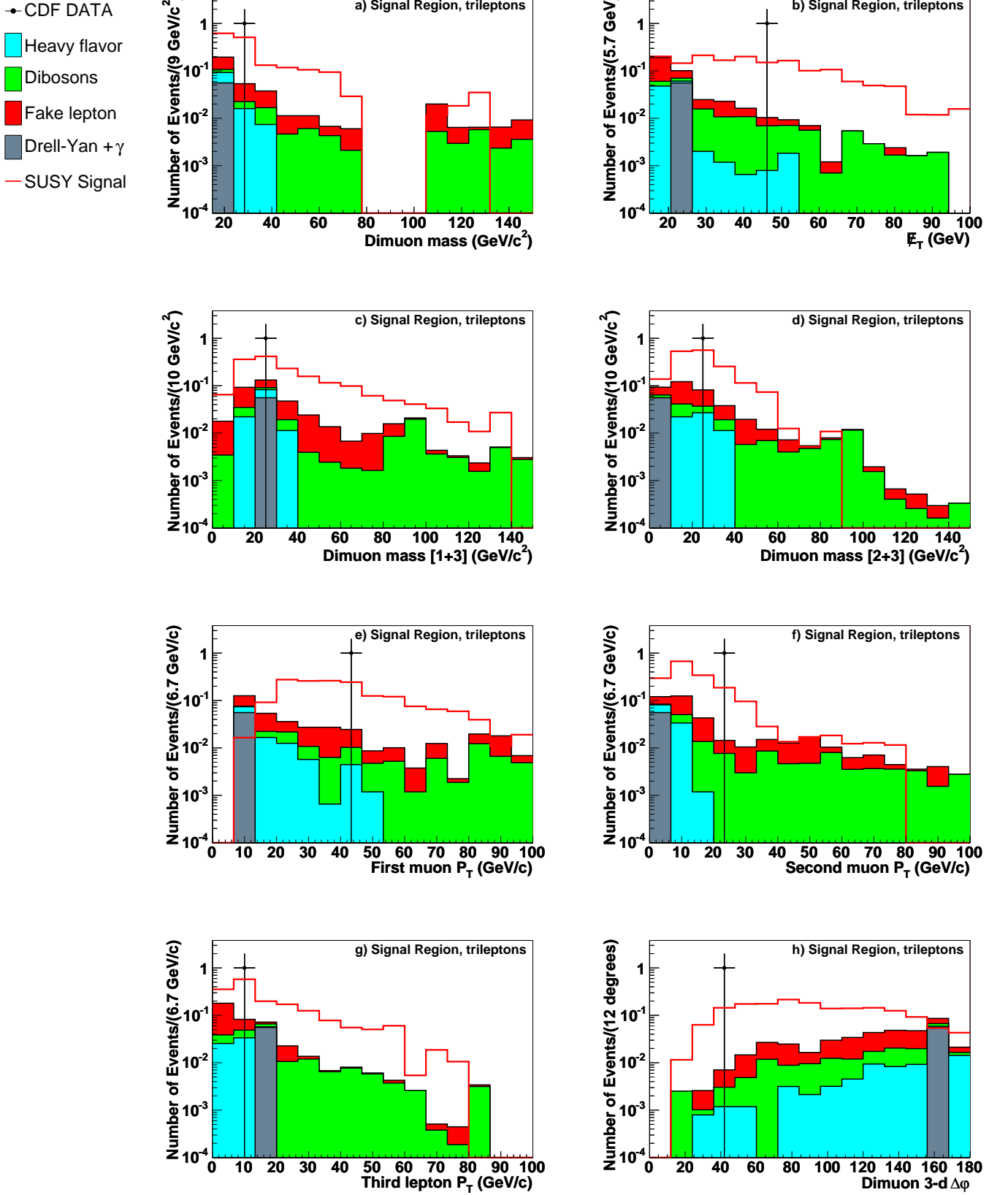
FIG. 8: Kinematic variables for the SM background and the SIG2 SUSY signal, in the trilepton signal region. The background histograms are stacked; the signal histogram is not. The CDF data are indicated by points with error bars.
