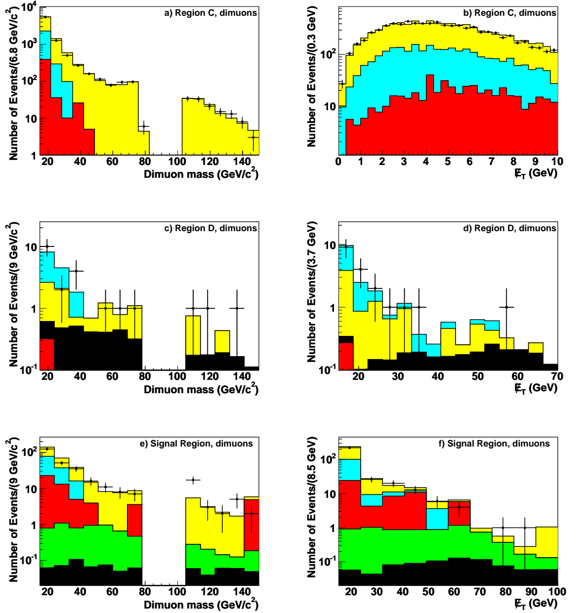
FIG. 7: Dimuon mass and E_T for the SM background in the dimuon control regions C (a,b), D (c,d), and dimuon signal region (e,f). The background histograms are stacked. The CDF data are indicated by points with error bars.
