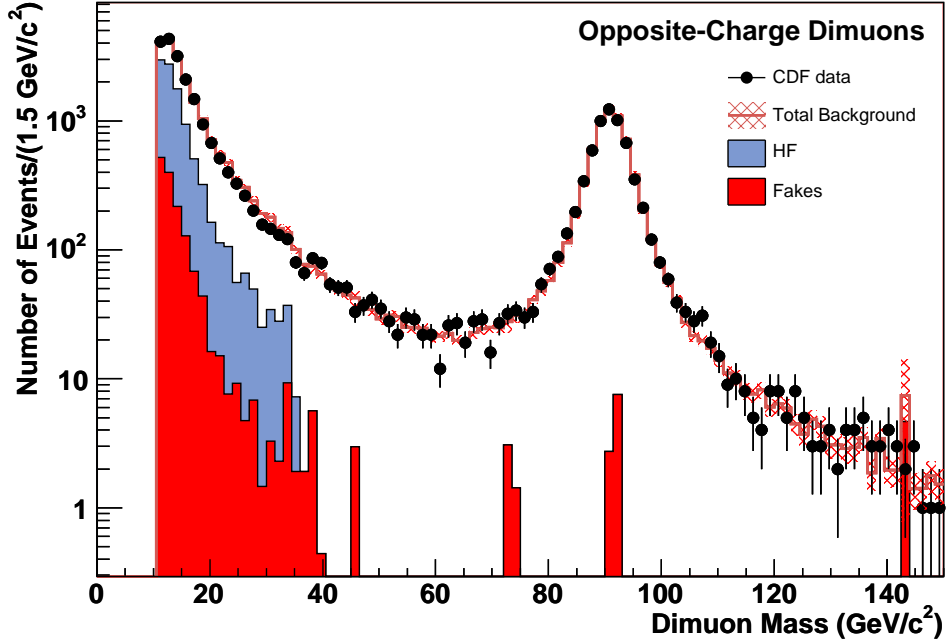
FIG. 3: Fit of HF+DY+fakes dimuon mass distribution to the observed data for opposite-charge dimuons. The HF normalization is the only free parameter of the fit. The blue (light gray) filled histogram is the HF and the red (dark gray) is the fakes. The thick line represents the total background, which is almost exclusively DY, HF, and fakes at the opposite-charge dimuon level. The hatched areas indicate the total uncertainty on the prediction.
