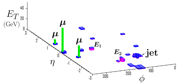
FIG. 10: The trimuon event in the \eta - \phi view. Calorimeter transverse energies above 1 GeV are shown. The longer bars correspond to the track momenta of the three muons (high \phi ). The calorimeter energy depositions E_1 and E_2 are mainly electromagnetic and could be associated with two photons.
