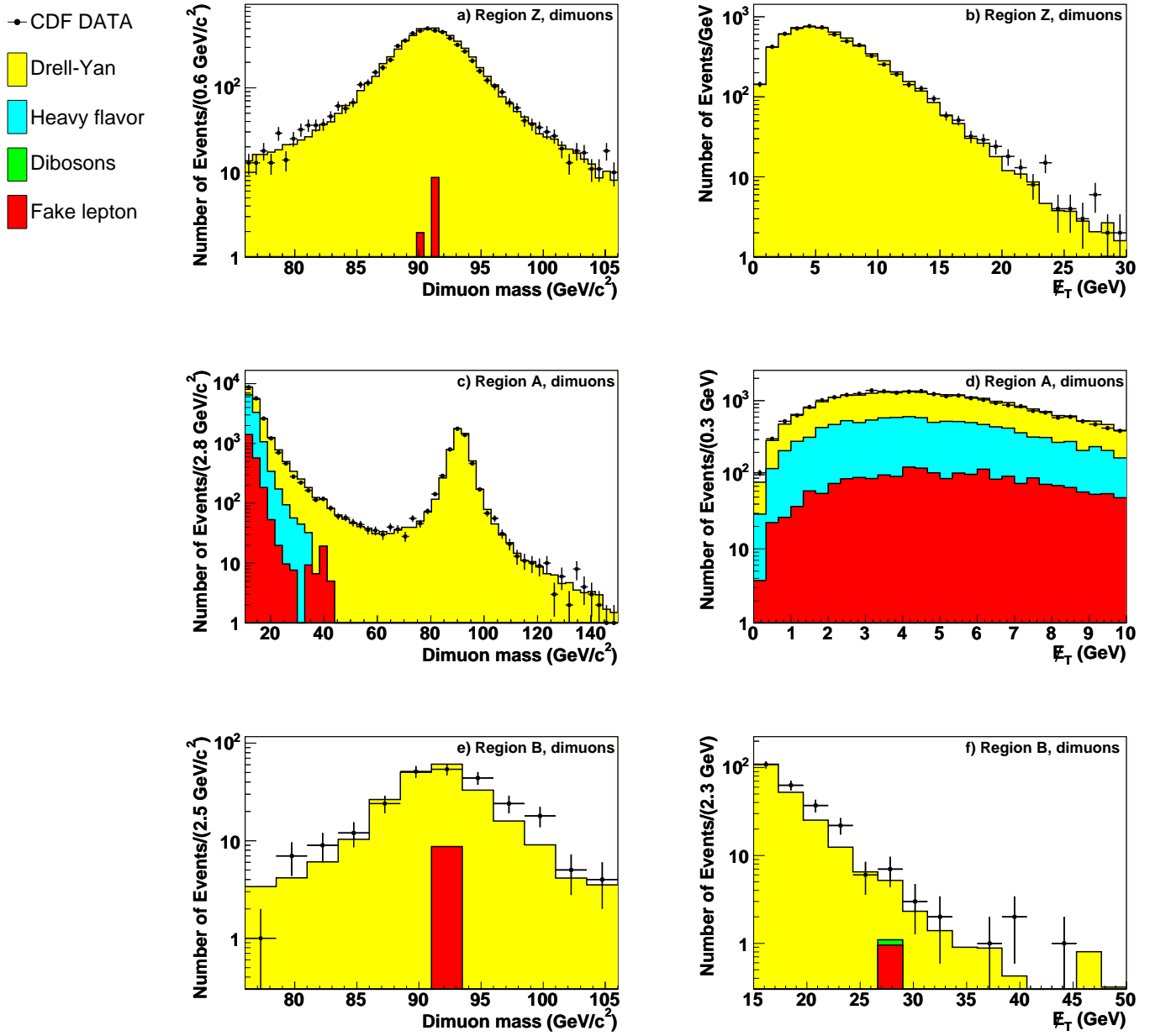
FIG. 6: Dimuon mass and E_T distributions for the SM background in the dimuon control regions Z (a,b), A (c,d), and B (e,f). The background histograms are stacked. The CDF data are indicated by points with error bars.
