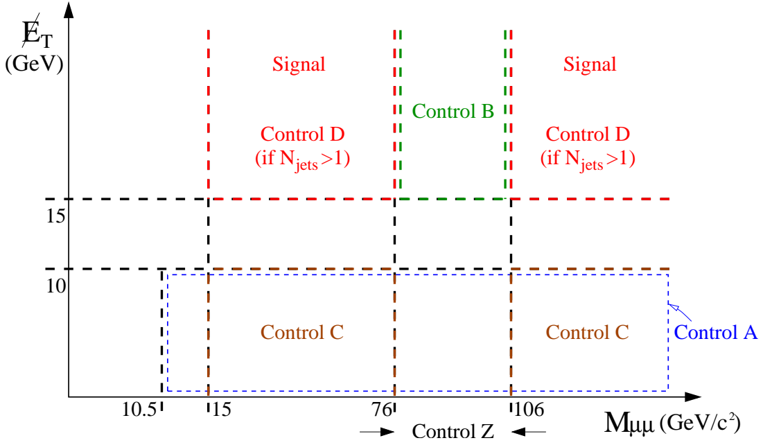
FIG. 5: The control and signal regions used in our analysis are defined in the dimuon mass vs. \cancel{E}_T plane, with the extra requirement of low ( \leq 1 ) or high ( > 1 ) jet multiplicity. In this paper we show results for the control regions that result from the inversion of one of the three main kinematic selections (dimuon mass, missing transverse energy, and jet multiplicity), with the addition of a Z -mass control region (Control Z) and a low- \cancel{E}_T control region (Control A). The control regions above are defined for low jet multiplicity, unless otherwise stated.
