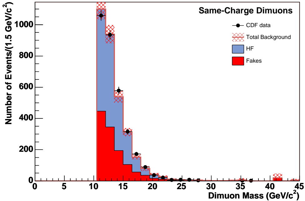
FIG. 4: Fit of HF+DY+fakes dimuon mass distribution to the observed data for same-charge dimuons. The HF normalization is the only free parameter of the fit. The blue (light gray) filled histogram is the HF and the red (dark gray) is the fakes. The thick line represents the total background, which is constituted almost exclusively by HF and fakes for same-charge dimuon pairs. The hatched areas indicate the total uncertainty on the prediction.
