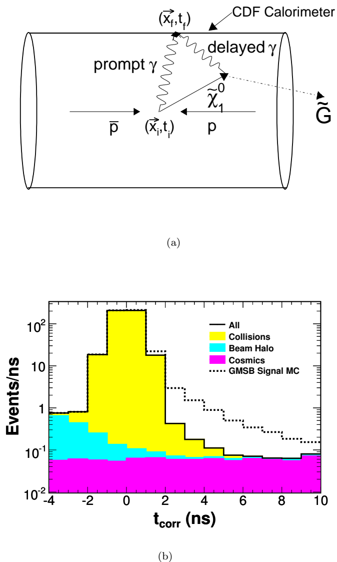
FIG. 2: (a) The schematic of a long-lived \tilde{\chi}_1^0 decaying into a G and a photon inside the detector. While the G leaves undetected the photon travels to the detector wall and deposits energy in the detector. A prompt photon would travel directly from the collision point to the detector walls. Relative to the expected arrival time, the photon from the \tilde{\chi}_1^0 would appear “delayed.” (b) The t_{\text{corr}} distribution for a simulated GMSB signal at an example point of m_{\tilde{\chi}_1^0} = 100 \text{ GeV}/c^2 and \tau_{\tilde{\chi}_1^0} = 5 \text{ ns} as well as for standard model and non-collision backgrounds.
