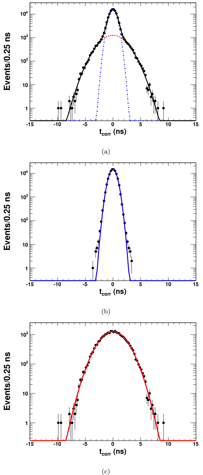
FIG. 13: The t_{\text{corr}} distribution for electrons in a sample of W \rightarrow e\nu events. In plot (a) the two Gaussians correspond to the cases when the highest- \Sigma p_T vertex is associated to the electron track and when it is not. These cases can be separated by requiring a match (b) and an anti-match (c), respectively, between the vertex and the electron track in both space and time.
