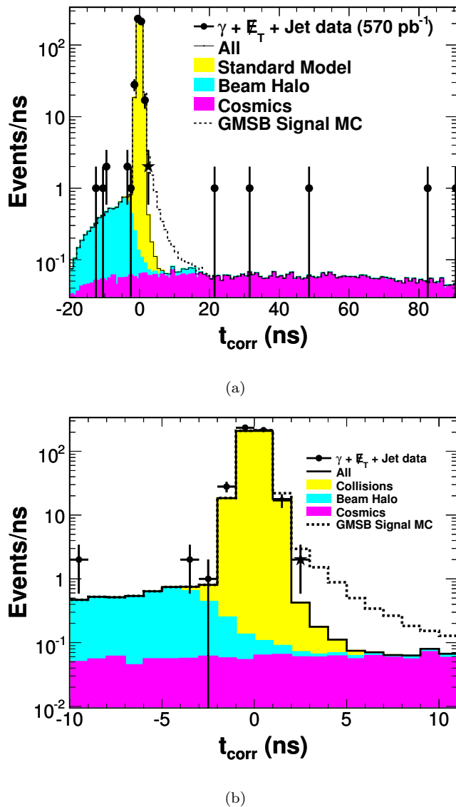
FIG. 21: The t_{\text{corr}} distribution including the control and signal regions, after all but the timing cut for all backgrounds, for the expected signal and the observed data. A total of 508 events is observed in the full time window. The two observed events in the signal region, 2 < t_{\text{corr}} < 10 ns, are in the first signal time bin (marked with a star). This is consistent with the background expectation of 1.3 \pm 0.7 events.
