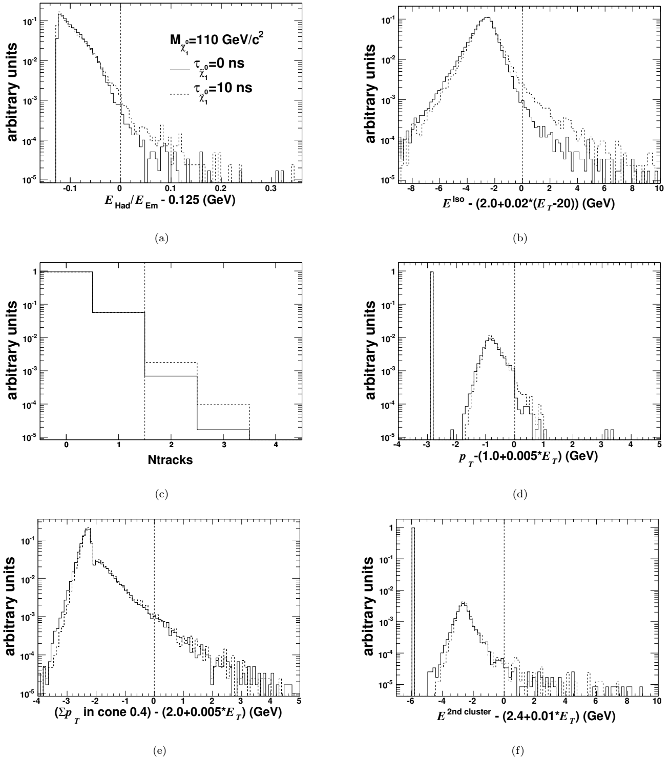
FIG. 5: A simulation of the ID variable distributions (minus their requirement value) for photons in a GMSB model with m_{\tilde{\chi}_1^0} = 110 \text{ GeV}/c^2 . The solid line is for prompt photons, simulated as decay photons from \tilde{\chi}_1^0 's with a lifetime of 0 ns and the dashed line is for photons from long-lived \tilde{\chi}_1^0 's with a lifetime of 10 ns. Entries to the left of the dashed vertical line pass the corresponding requirement. The bin at -2.8 in (d) collects the photons that have no track within the isolation cone. In (f) the bin at -6 shows the photons that have no 2nd CES cluster nearby. The distributions for all ID variables do not change significantly between the prompt and the long-lived case except for slight deviations in the energy isolation in (b) as discussed in the text.
