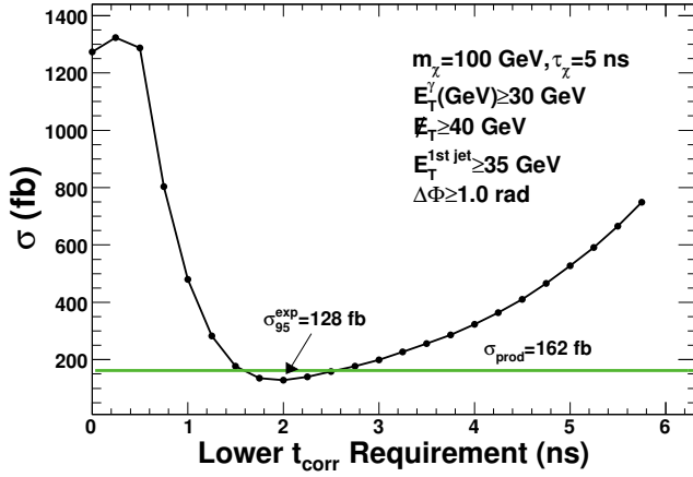
FIG. 20: The expected 95% C.L. cross section limit as a function of the lower value of the t_{\text{corr}} requirement for a GMSB example point with m_{\tilde{\chi}_1^0} = 100 \text{ GeV}/c^2 and \tau_{\tilde{\chi}_1^0} = 5 \text{ ns} . The values of the kinematic sample requirements are held at their optimized values.
