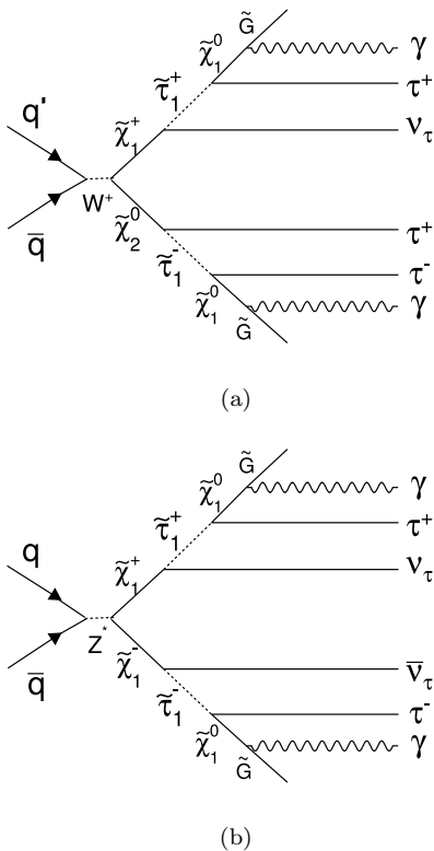
FIG. 1: Feynman diagrams of the dominant tree-production processes at the Fermilab Tevatron for the SPS 8 GMSB model line. The taus and second photons, if available, can be identified as jets in the detector. Note that only one choice for the charge is shown.
