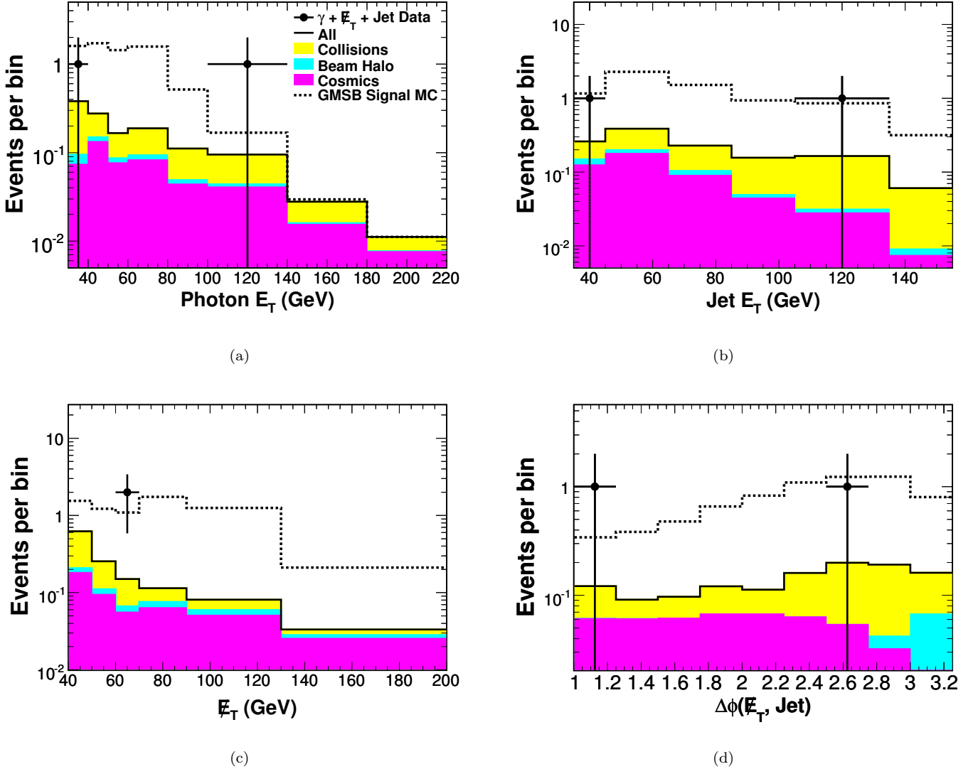
FIG. 22: The predicted and observed photon E_T , jet E_T , \cancel{E}_T , and \Delta\phi(\cancel{E}_T, \text{jet}) distributions for the signal region after the final event selection requirements. The GMSB distributions are for m_{\tilde{\chi}_1^0} = 100 \text{ GeV}/c^2 and \tau_{\tilde{\chi}_1^0} = 5 \text{ ns} . There is no evidence for new physics.
