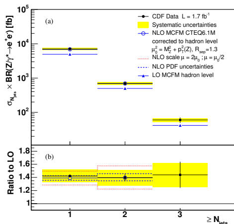
FIG. 2: (a) Measured total cross section for inclusive jet production in Z/\gamma^*(\rightarrow e^+e^-)+\text{jets} events as a function of N_{\text{jet}} compared to LO and NLO pQCD predictions. The shaded bands show the total systematic uncertainty, except for the 5.8% luminosity uncertainty. (b) Ratio of data and NLO to LO pQCD predictions versus N_{\text{jet}} . The dashed and dotted lines indicate the PDF uncertainty and the variation with \mu of the NLO pQCD predictions, respectively.
