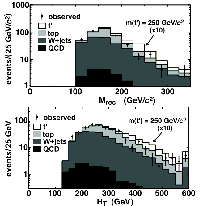
FIG. 1: Observed and predicted distributions of M_{rec} (above) and H_T (below). The predicted distribution corresponds to that for a 250 \text{ GeV}/c^2 mass t'\bar{t}' signal assuming a value of the cross section at ten times the theoretical one. Note that in each plot the last bin is an overflow bin, and that the W +jets contribution also represents other similar backgrounds.
